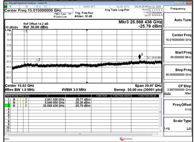
Band41_40MHz_DFT_s_OFDM_SCS30kHz_BPSK_RB1_1_CH518598
