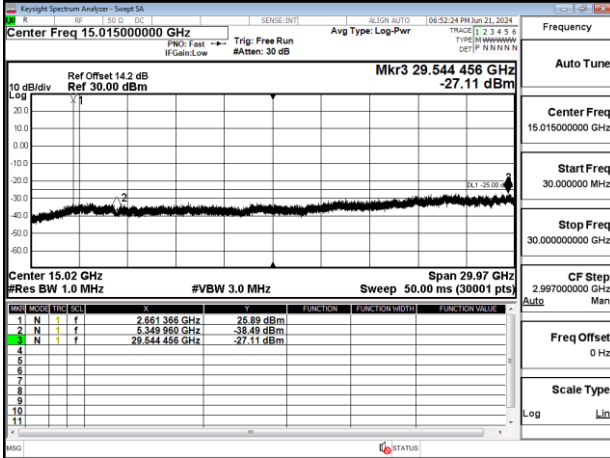
Band41_40MHz_DFT_s_OFDM_SCS30kHz_BPSK_RB1_1_CH503202
