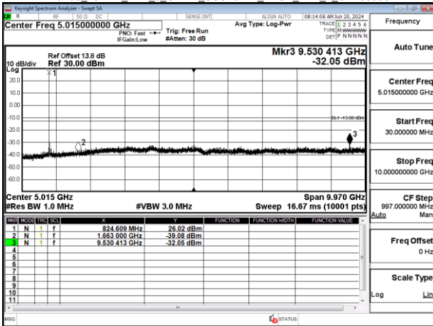
Band5 15MHz DFT s OFDM_SCS15kHz_BPSK_RB1_1_CH167300
