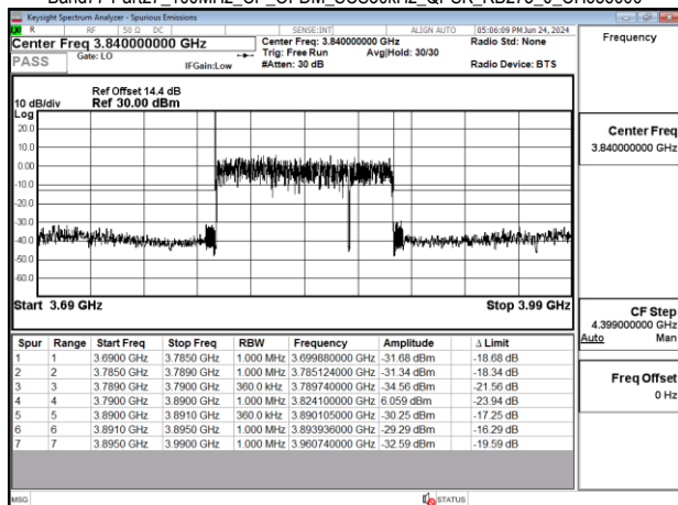
Band77-Part27_100MHz_CP_OFDM_SCS30kHz_QPSK_RB273_0_CH656000
