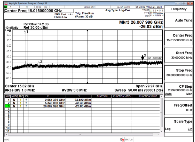
Band41_40MHz_DFT_s_OFDM_SCS30kHz_BPSK_RB1_1_CH534000
