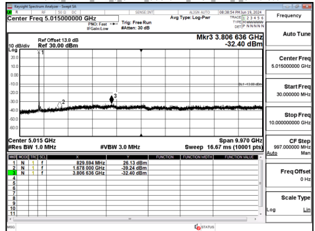
Band5 20MHz DFT s OFDM_SCS15kHz_BPSK_RB1_1_CH167800
