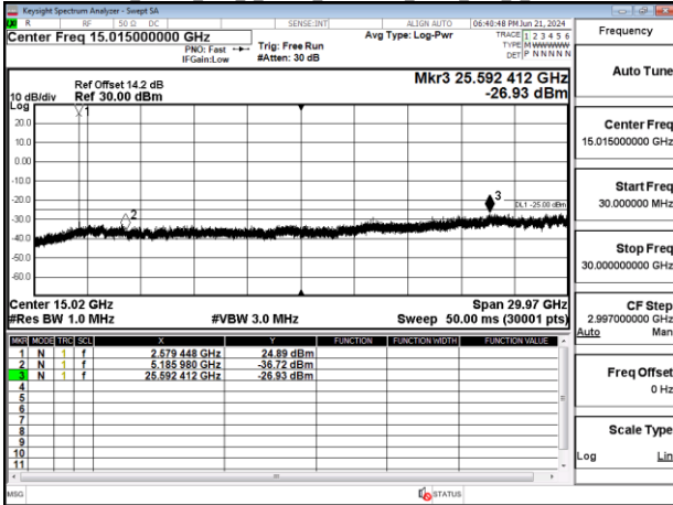
Band41_30MHz_DFT_s_OFDM_SCS30kHz_BPSK_RB1_1_CH534996
