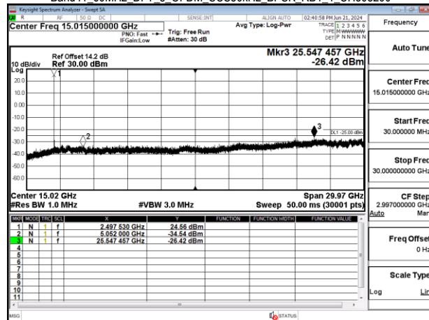
Band41_60MHz_DFT_s_OFDM_SCS30kHz_BPSK_RB1_1_CH506004
