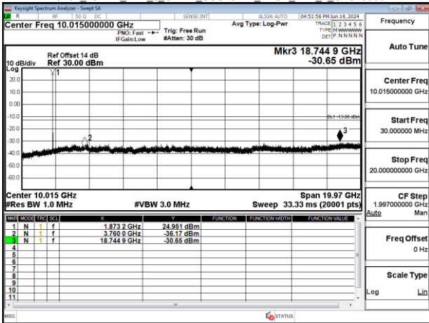
Band2 15MHz DFT s OFDM_SCS15kHz_BPSK_RB1_1_CH380500
