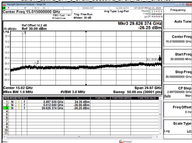
Band41_20MHz_DFT_s_OFDM_SCS30kHz_BPSK_RB1_1_CH502002
