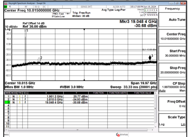
Band2 10MHz DFT s_OFDM_SCS15kHz_BPSK_RB1_1_CH381000
