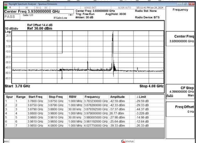
Band77-Part27_100MHz_CP_OFDM_SCS30kHz_QPSK_RB1_272_CH662000
