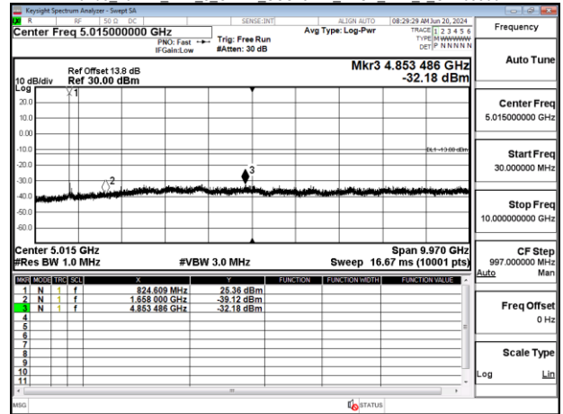
Band5 10MHz DFT s_OFDM_SCS15kHz_BPSK_RB1_1_CH167300
