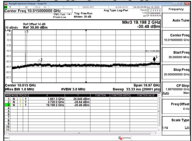
Band2 20MHz DFT s OFDM_SCS15kHz_BPSK_RB1_1_CH376000
