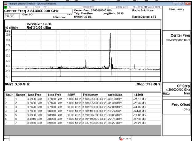
Band77-Part27_100MHz_CP_OFDM_SCS30kHz_QPSK_RB1_272_CH662000
