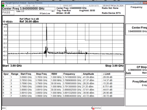
Band77-Part27_100MHz_CP_OFDM_SCS30kHz_QPSK_RB1_0_CH662000
