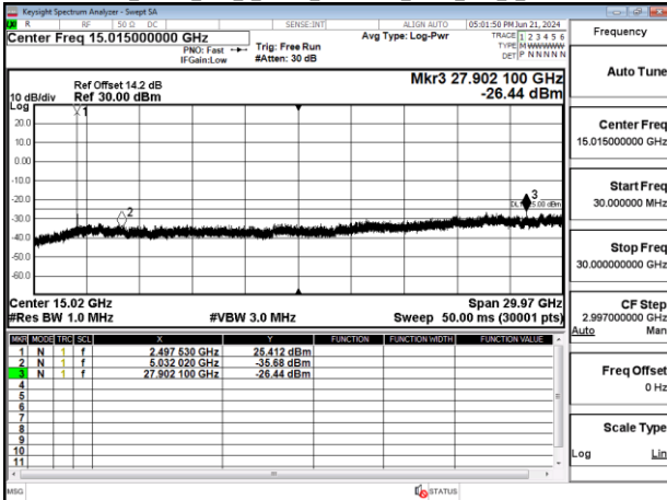
Band41_40MHz_DFT_s_OFDM_SCS30kHz_BPSK_RB1_1_CH503202
