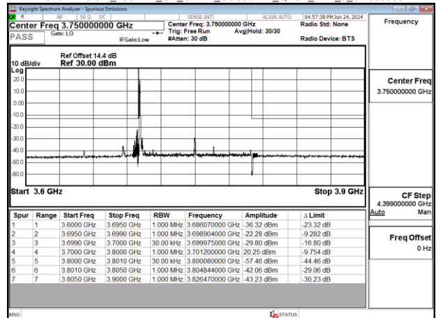
Band77-Part27_100MHz_CP_OFDM_SCS30kHz_QPSK_RB1_0_CH650000
