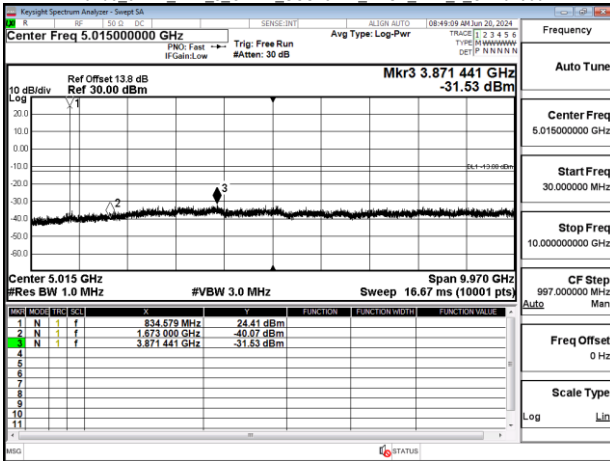
Band5 5MHz DFT s_OFDM_SCS15kHz_BPSK_RB1_1_CH169300
