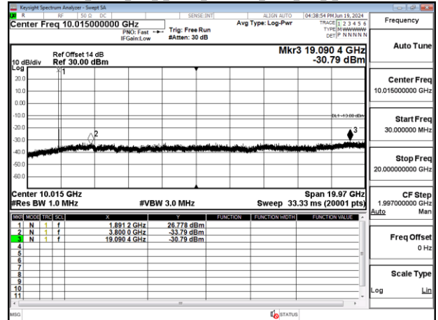
Band2 20MHz DFT s OFDM_SCS15kHz_BPSK_RB1_1_CH380000
