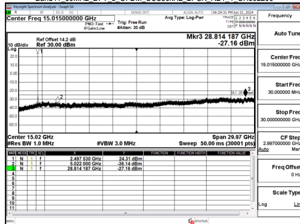
Band41_30MHz_DFT_s_OFDM_SCS30kHz_BPSK_RB1_1_CH503004
