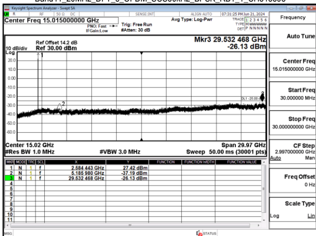
Band41_20MHz_DFT_s_OFDM_SCS30kHz_BPSK_RB1_1_CH518598
