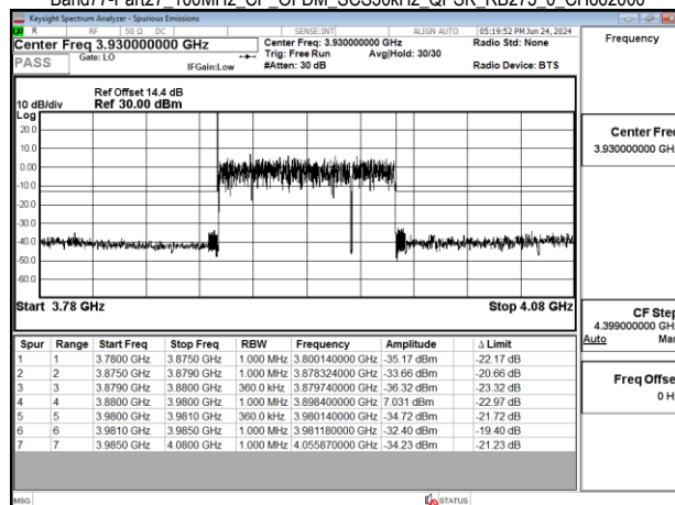
Band77-Part27_100MHz_CP_OFDM_SCS30kHz_QPSK_RB273_0_CH662000
