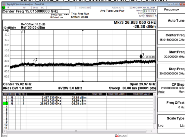
Band41_50MHz_DFT_s_OFDM_SCS30kHz_BPSK_RB1_1_CH505002
