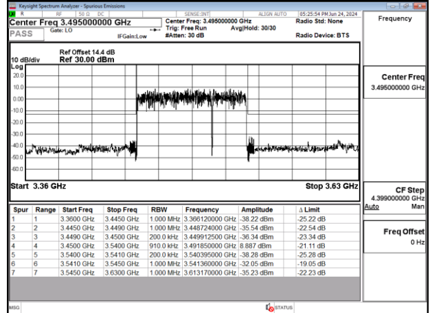
Band77-Part27_90MHz_DFT_s_OFDM_SCS30kHz_BPSK_RB243_0_CH633334
