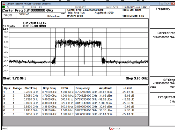
Band77-Part27_80MHz_CP_OFDM_SCS30kHz_QPSK_RB217_0_CH656000
