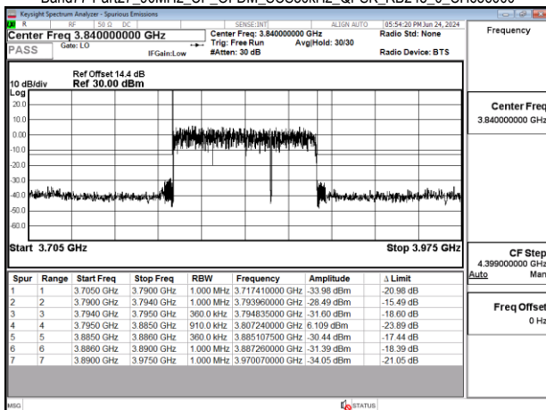
Band77-Part27_90MHz_CP_OFDM_SCS30kHz_QPSK_RB245_0_CH656000
