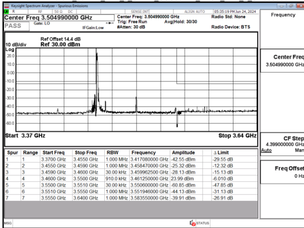
Band77-Part27_90MHz_DFT_s_OFDM_SCS30kHz_BPSK_RB1_0_CH649668
