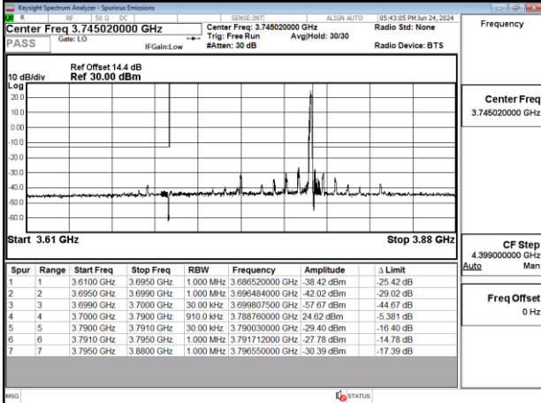
Band77-Part27_90MHz_DFT_s_OFDM_SCS30kHz_BPSK_RB1_244_CH656000
