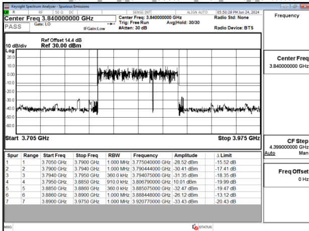
Band77-Part27_90MHz_DFT_s_OFDM_SCS30kHz_BPSK_RB243_0_CH656000
