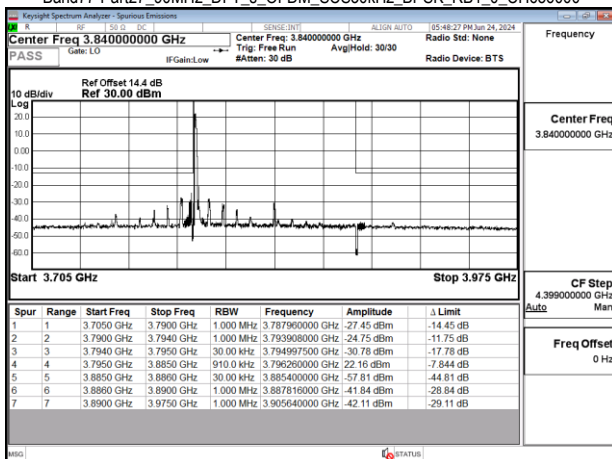
Band77-Part27_90MHz_DFT_s_OFDM_SCS30kHz_BPSK_RB1_0_CH656000
