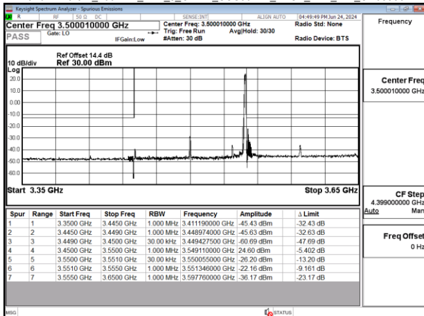
Band77-Part27_100MHz_DFT_s_OFDM_SCS30kHz_BPSK_RB1_272_CH633334
