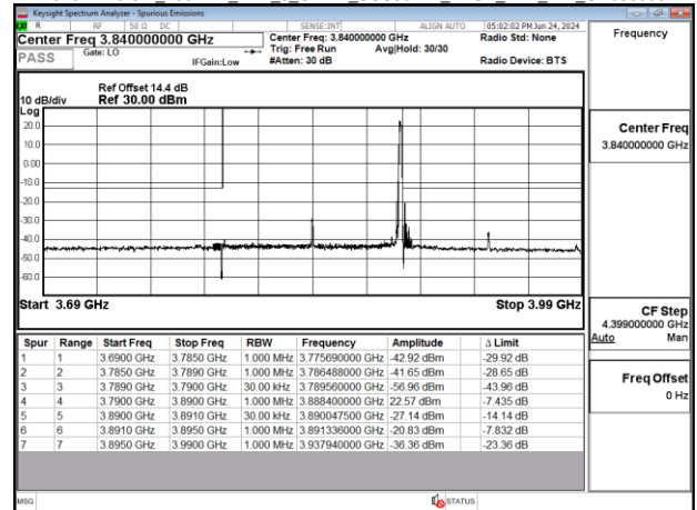
Band77-Part27_100MHz_DFT_s_OFDM_SCS30kHz_BPSK_RB1_272_CH662000
