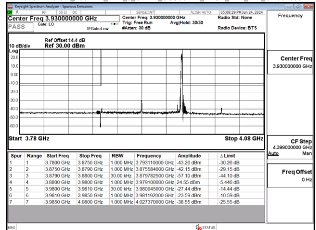
Band77-Part27_100MHz_DFT_s_OFDM_SCS30kHz_BPSK_RB1_272_CH662000
