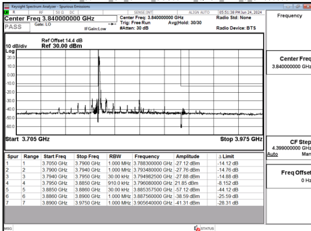
Band77-Part27_90MHz_CP_OFDM_SCS30kHz_QPSK_RB1_0_CH656000
