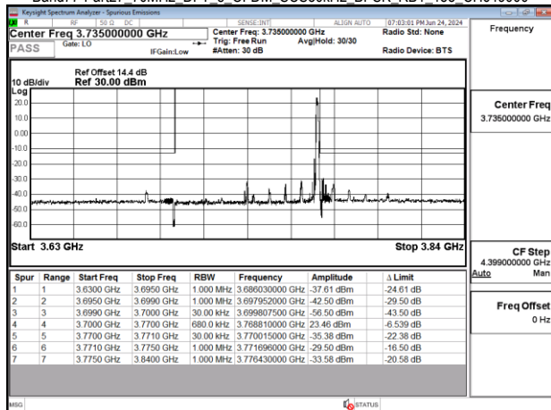
Band77-Part27_70MHz_DFT_s_OFDM_SCS30kHz_BPSK_RB1_188_CH656000
