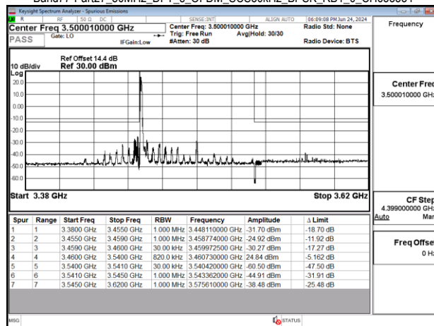
Band77-Part27_80MHz_DFT_s_OFDM_SCS30kHz_BPSK_RB1_0_CH633334
