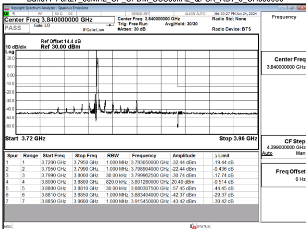
Band77-Part27_80MHz_CP_OFDM_SCS30kHz_QPSK_RB1_0_CH656000
