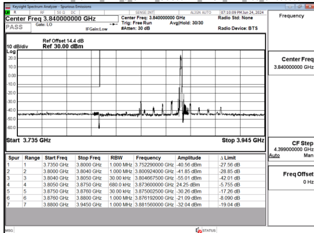
Band77-Part27_70MHz_DFT_s_OFDM_SCS30kHz_BPSK_RB1_188_CH656000
