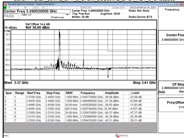
Band77-Part27_80MHz_DFT_s_OFDM_SCS30kHz_BPSK_RB1_0_CH633334
