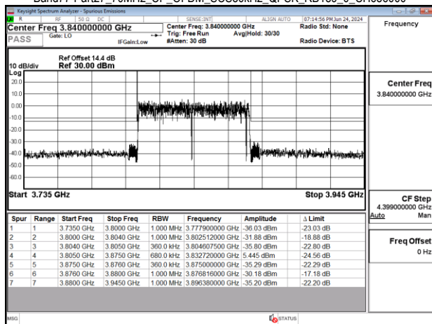
Band77-Part27_70MHz_CP_OFDM_SCS30kHz_QPSK_RB189_0_CH656000
