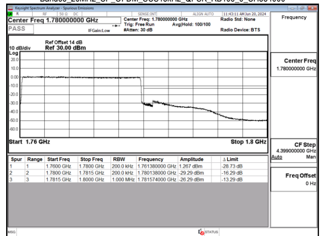
Band66_20MHz_CP_OFDM_SCS15kHz_QPSK_RB106_0_CH354000
