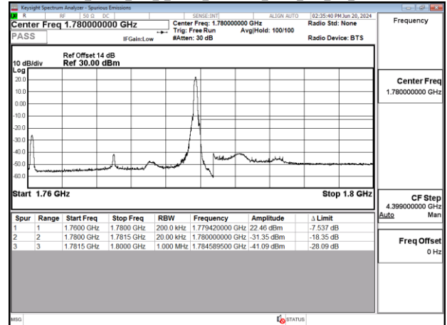
Band66_20MHz_DFT_s_OFDM_SCS15kHz_BPSK_RB1_105_CH354000
