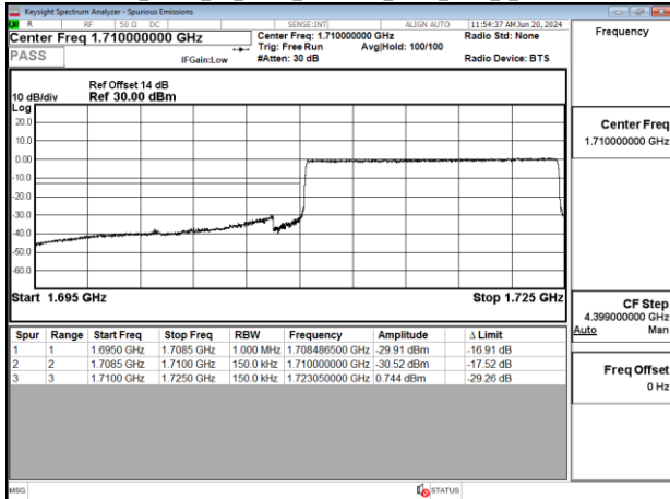
Band66_15MHz_CP_OFDM_SCS15kHz_QPSK_RB79_0_CH343500
