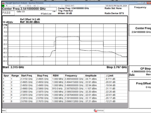
Band41_90MHz_CP_OFDM_SCS30kHz_QPSK_RB245_0_CH509004
