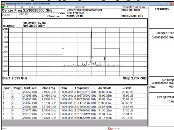
Band41_80MHz_DFT_s_OFDM_SCS30kHz_BPSK_RB1_216_CH507204
