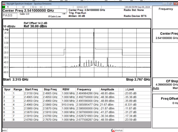
Band41_90MHz_DFT_s_OFDM_SCS30kHz_BPSK_RB1_244_CH508200
