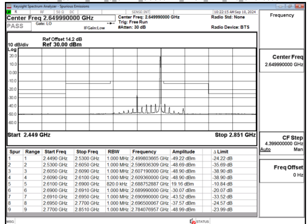
Band41_80MHz_DFT_s_OFDM_SCS30kHz_BPSK_RB1_216_CH529998
