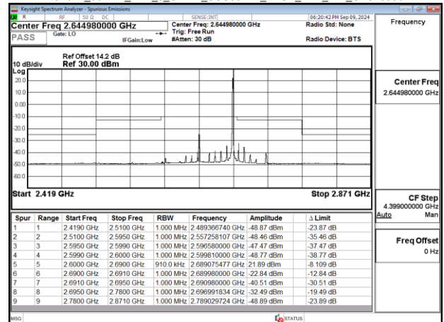
Band41_90MHz_DFT_s_OFDM_SCS30kHz_BPSK_RB1_244_CH528996
