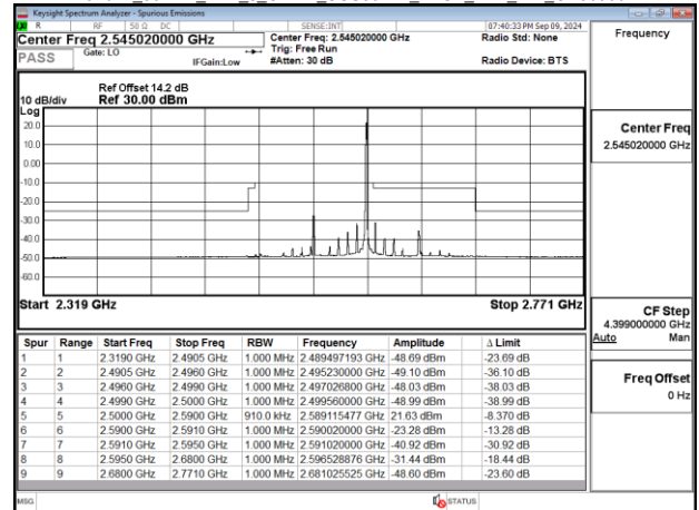
Band41_90MHz_DFT_s_OFDM_SCS30kHz_BPSK_RB1_244_CH518598
