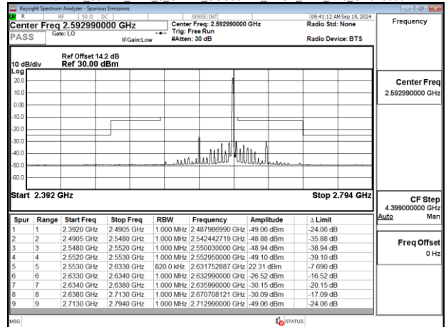
Band41_80MHz_DFT_s_OFDM_SCS30kHz_BPSK_RB1_216_CH529998
