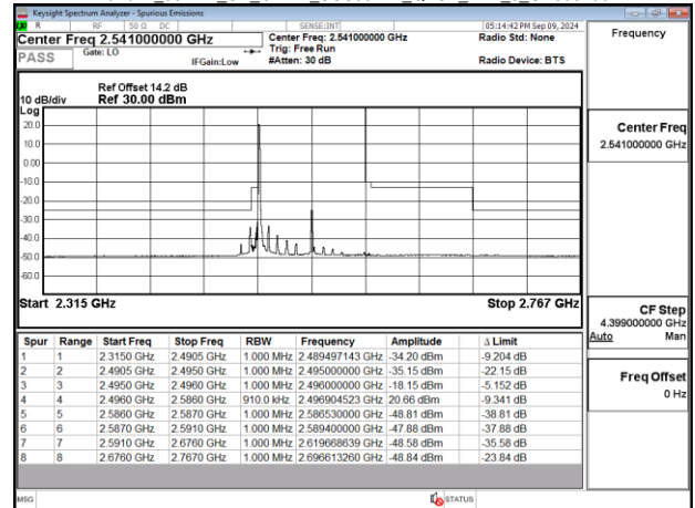
Band41_90MHz_CP_OFDM_SCS30kHz_QPSK_RB1_0_CH509004
