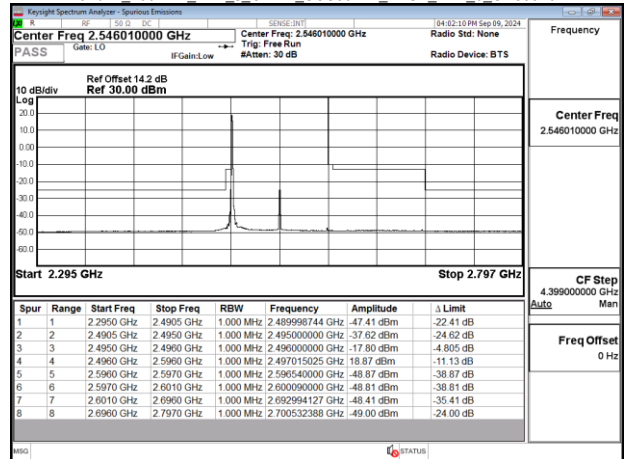
Band41_100MHz_DFT_s_OFDM_SCS30kHz_BPSK_RB1_0_CH510000
