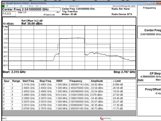
Band41_90MHz_DFT_s_OFDM_SCS30kHz_BPSK_RB243_0_CH509004
