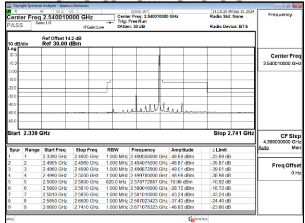
Band41_80MHz_DFT_s_OFDM_SCS30kHz_BPSK_RB1_216_CH518598
