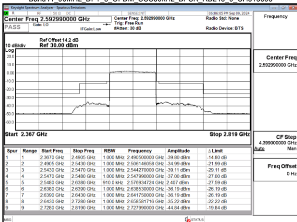
Band41_90MHz_DFT_s_OFDM_SCS30kHz_BPSK_RB243_0_CH518598
