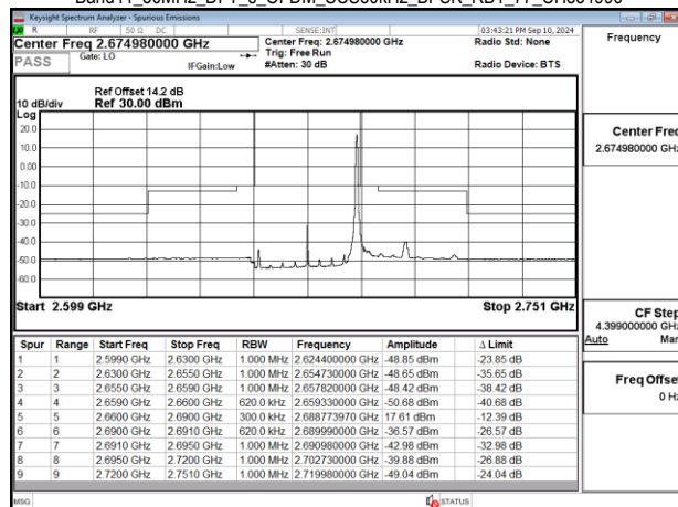
Band41_30MHz_DFT_s_OFDM_SCS30kHz_BPSK_RB1_77_CH534996
