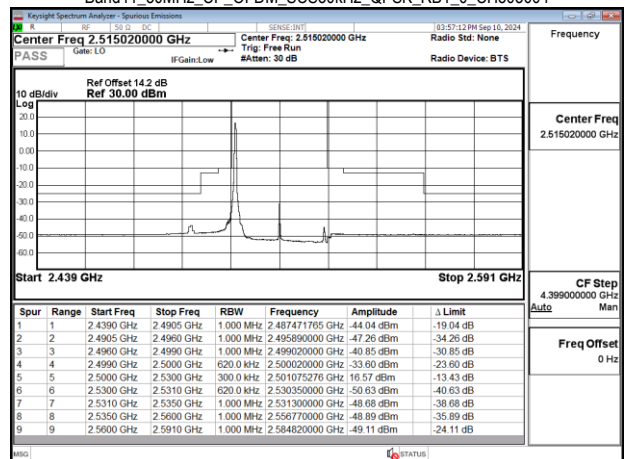
Band41_30MHz_CP_OFDM_SCS30kHz_QPSK_RB1_0_CH503004
