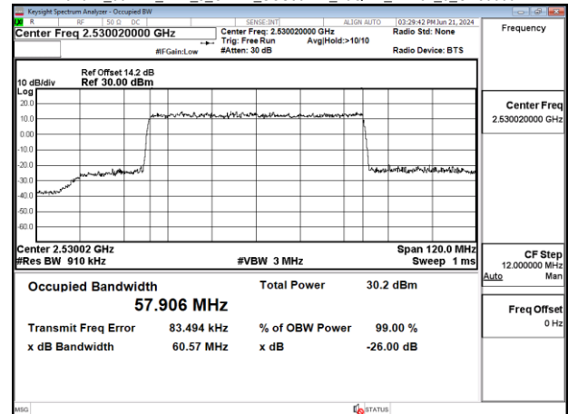
Band41_60MHz_DFT_s_OFDM_SCS30kHz_16QAM_RB162_0_CH506004
