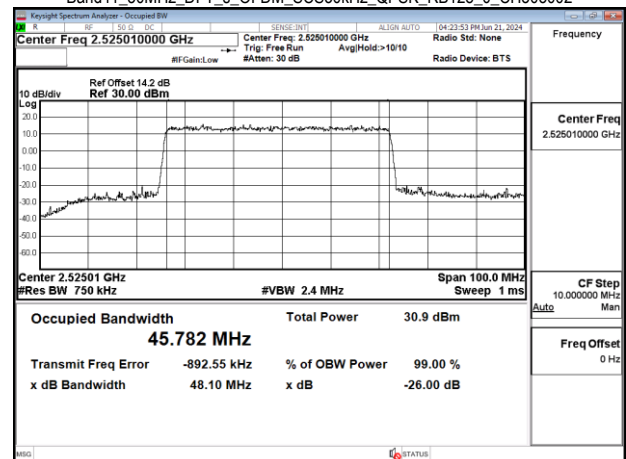
Band41_50MHz_DFT_s_OFDM_SCS30kHz_QPSK_RB128_0_CH505002
