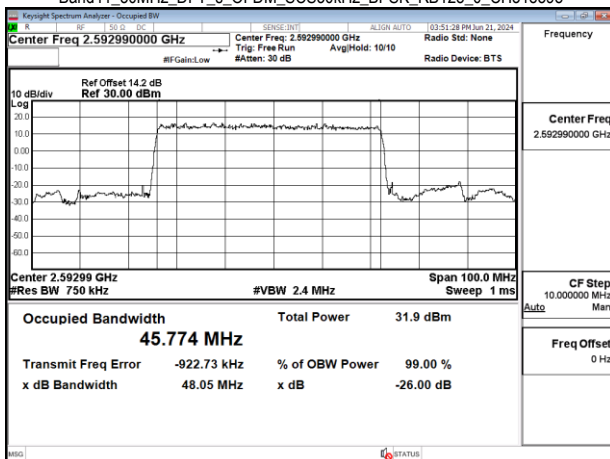
Band41_50MHz_DFT_s_OFDM_SCS30kHz_BPSK_RB128_0_CH518598
