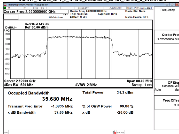
Band41_40MHz_DFT_s_OFDM_SCS30kHz_BPSK_RB100_0_CH504000
