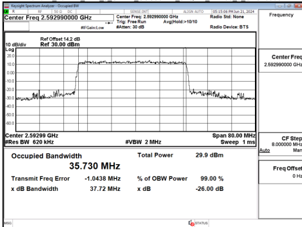
Band41 40MHz DFT s OFDM SCS30kHz 64QAM RB100_0 CH534000
