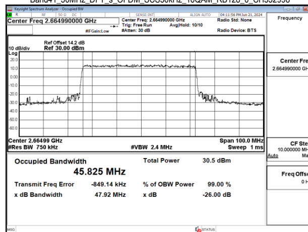
Band41_50MHz_DFT_s_OFDM_SCS30kHz_16QAM_RB128_0_CH532998
