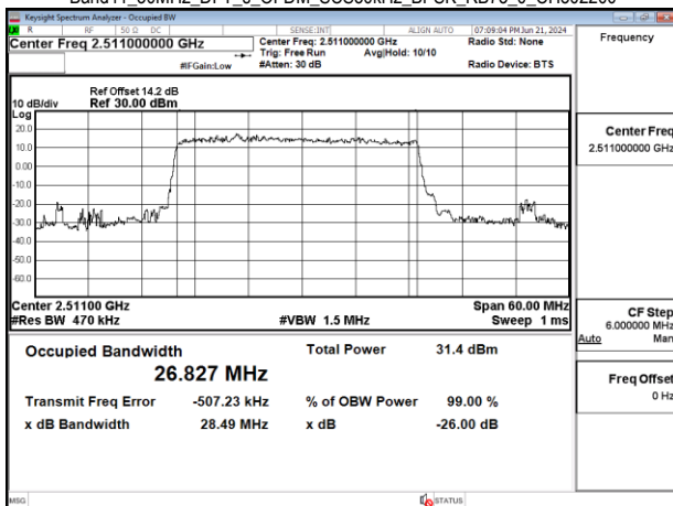
Band41_30MHz_DFT_s_OFDM_SCS30kHz_BPSK_RB75_0_CH502200
