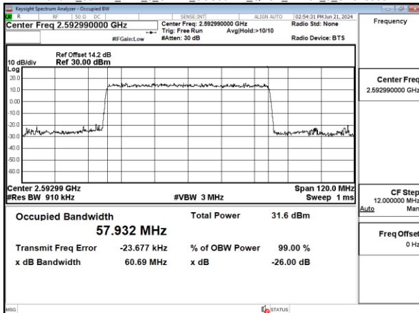
Band41_60MHz_DFT_s_OFDM_SCS30kHz_QPSK_RB162_0_CH518598
