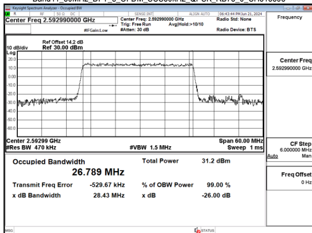
Band41_30MHz_DFT_s_OFDM_SCS30kHz_QPSK_RB75_0_CH518598
