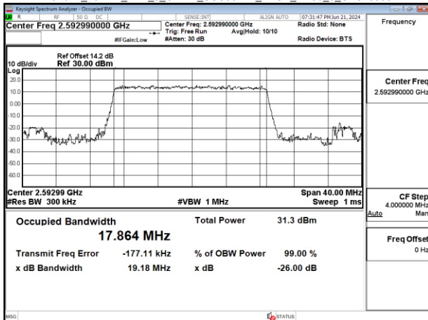
Band41_20MHz_DFT_s_OFDM_SCS30kHz_BPSK_RB50_0_CH518598
