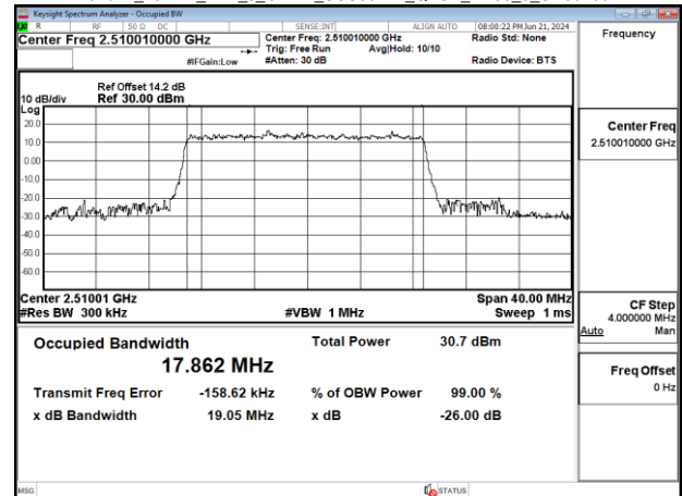
Band41_20MHz_DFT_s_OFDM_SCS30kHz_QPSK_RB50_0_CH502002
