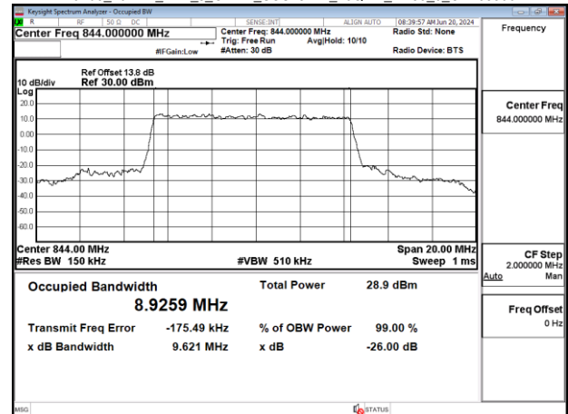
Band5_10MHz_DFT_s_OFDM_SCS15kHz_16QAM_RB50_0_CH168800
