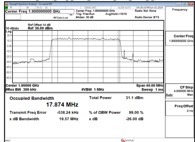
Band2_20MHz_DFT_s_OFDM_SCS15kHz_BPSK_RB100_0_CH380000
