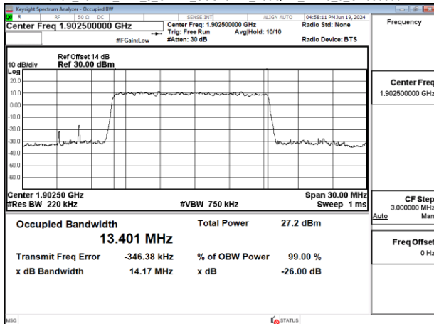
Band2_15MHz_DFT_s_OFDM_SCS15kHz_256QAM_RB75_0_CH380500
