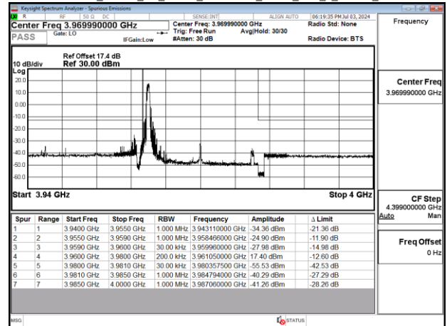
Band77-Part27_20MHz_CP_OFDM_SCS30kHz_QPSK_RB1_0_Chain0_CH664666
