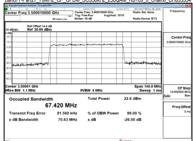
Band77-Part27_70MHz_CP_OFDM_SCS30kHz_256QAM_RB189_0_Chain0_CH632334
