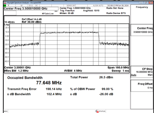
Band77-Part27_80MHz_CP_OFDM_SCS30kHz_16QAM_RB217_0_Chain0_CH633334
