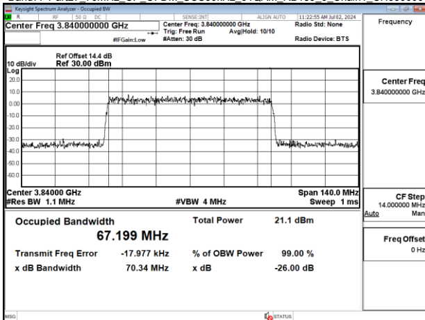
Band77-Part27_70MHz_CP_OFDM_SCS30kHz_64QAM_RB189_0_Chain1_CH656000
