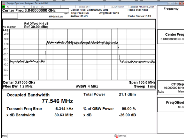
Band77-Part27_80MHz_CP_OFDM_SCS30kHz_QPSK_RB217_0_Chain1_CH656000
