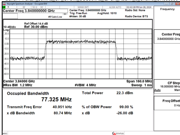
Band77-Part27_80MHz_CP_OFDM_SCS30kHz_QPSK_RB217_0_Chain0_CH656000
