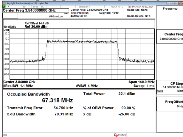
Band77-Part27_70MHz_CP_OFDM_SCS30kHz_QPSK_RB189_0_Chain1_CH656000
