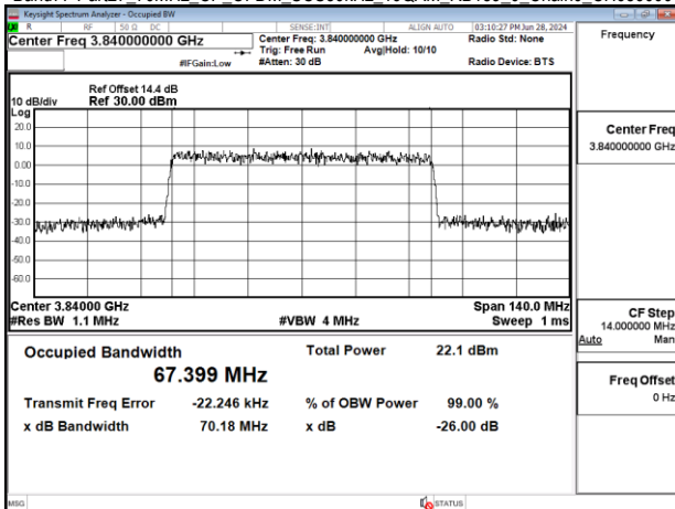
Band77-Part27_70MHz_CP_OFDM_SCS30kHz_16QAM_RB189_0_Chain0_CH656000
