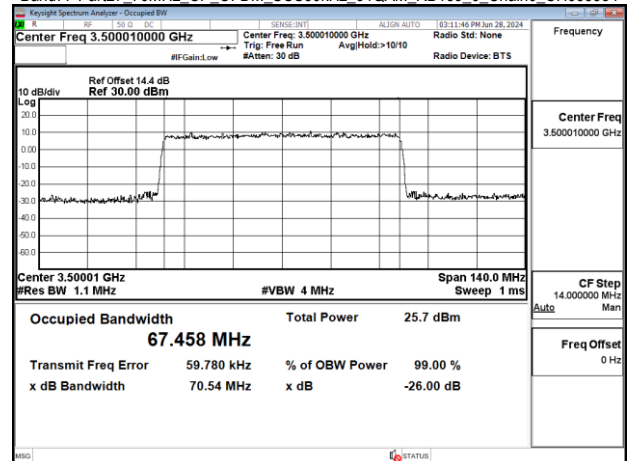
Band77-Part27_70MHz_CP_OFDM_SCS30kHz_64QAM_RB189_0_Chain0_CH633334
