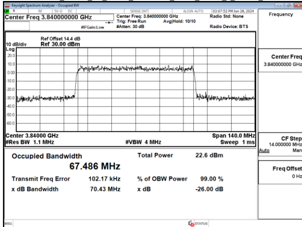
Band77-Part27_70MHz_CP_OFDM_SCS30kHz_QPSK_RB189_0_Chain0_CH656000
