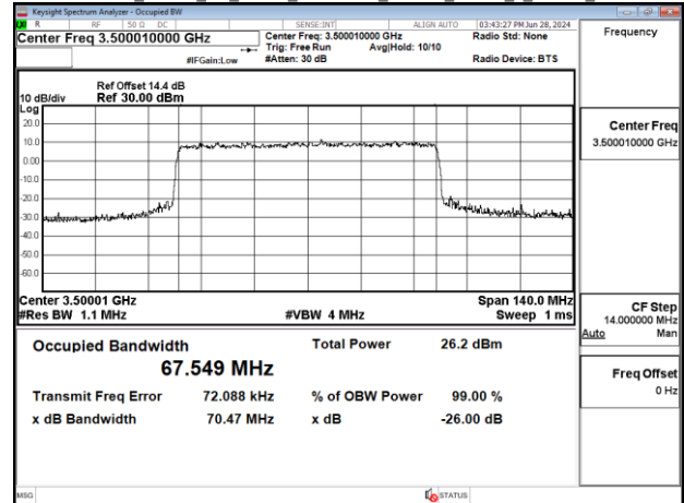
Band77-Part27_70MHz_CP_OFDM_SCS30kHz_16QAM_RB189_0_Chain0_CH633334
