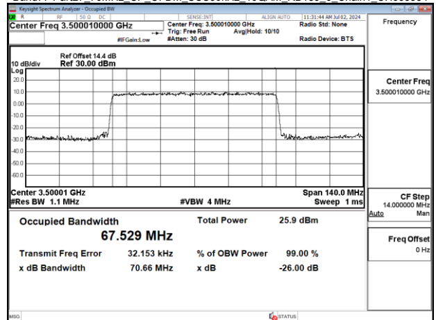
Band77-Part27_70MHz_CP_OFDM_SCS30kHz_16QAM_RB189_0_Chain1_CH633334
