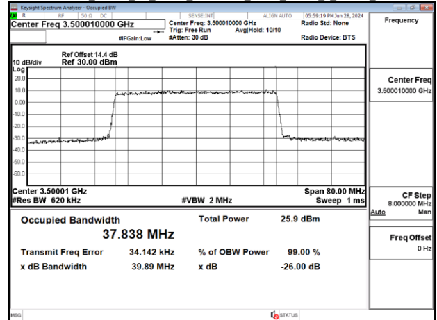
Band77-Part27_40MHz_CP_OFDM_SCS30kHz_QPSK_RB106_0_Chain0_CH633334
