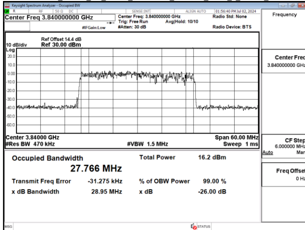
Band77-Part27_30MHz_CP_OFDM_SCS30kHz_256QAM_RB78_0_Chain1_CH656000
