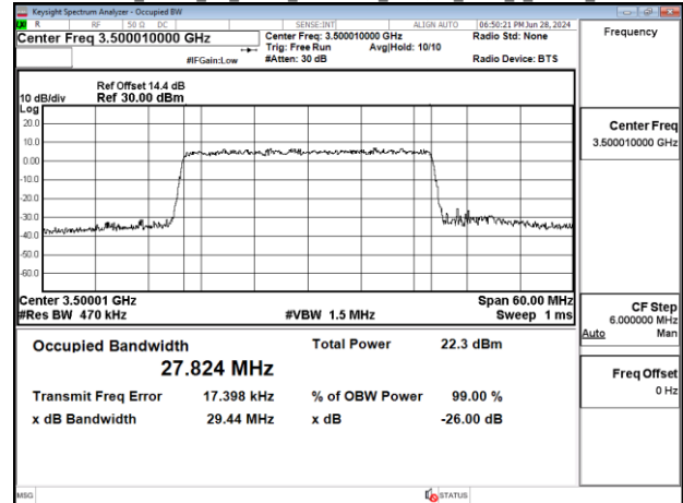
Band77-Part27_30MHz_CP_OFDM_SCS30kHz_256QAM_RB78_0_Chain0_CH633334
