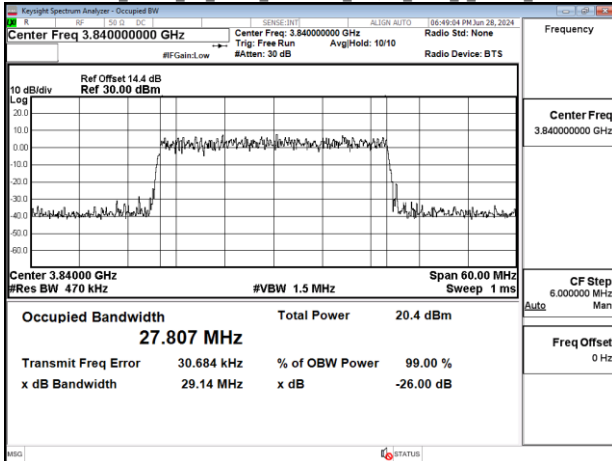
Band77-Part27_30MHz_CP_OFDM_SCS30kHz_64QAM_RB78_0_Chain0_CH656000
