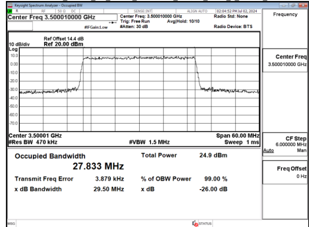
Band77-Part27_30MHz_CP_OFDM_SCS30kHz_64QAM_RB78_0_Chain1_CH633334
