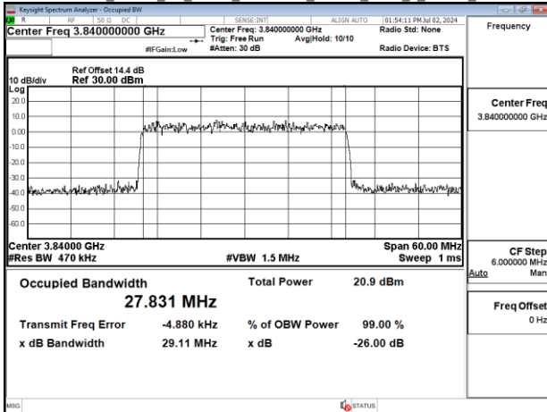
Band77-Part27_30MHz_CP_OFDM_SCS30kHz_64QAM_RB78_0_Chain1_CH656000
