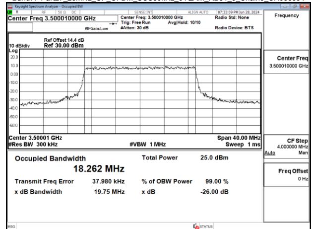
Band77-Part27_20MHz_CP_OFDM_SCS30kHz_64QAM_RB51_0_Chain0_CH633334
