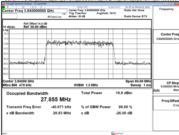
Band77-Part27_30MHz_CP_OFDM_SCS30kHz_16QAM_RB78_0_Chain1_CH656000
