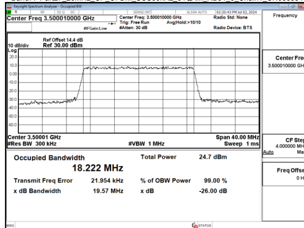
Band77-Part27_20MHz_CP_OFDM_SCS30kHz_64QAM_RB51_0_Chain1_CH633334
