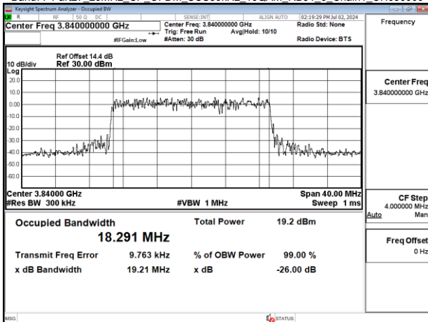
Band77-Part27_20MHz_CP_OFDM_SCS30kHz_16QAM_RB51_0_Chain1_CH656000
