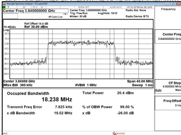
Band77-Part27_20MHz_CP_OFDM_SCS30kHz_16QAM_RB51_0_Chain0_CH656000
