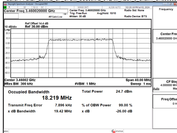
Band77-Part27_20MHz_CP_OFDM_SCS30kHz_64QAM_RB51_0_Chain1_CH633334
