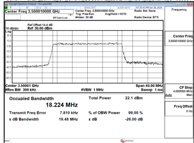
Band77-Part27_20MHz_CP_OFDM_SCS30kHz_256QAM_RB51_0_Chain0_CH633334
