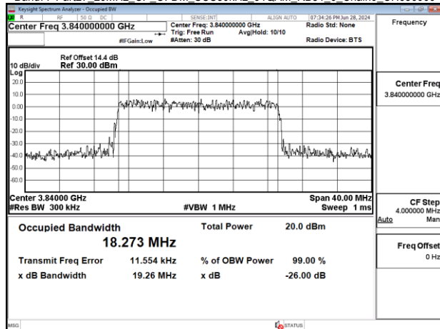
Band77-Part27_20MHz_CP_OFDM_SCS30kHz_64QAM_RB51_0_Chain0_CH656000
