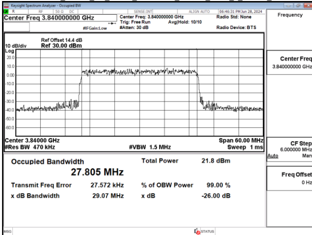
Band77-Part27_30MHz_CP_OFDM_SCS30kHz_16QAM_RB78_0_Chain0_CH656000
