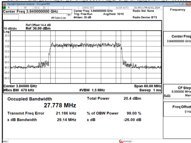
Band77-Part27_30MHz_CP_OFDM_SCS30kHz_QPSK_RB78_0_Chain1_CH656000
