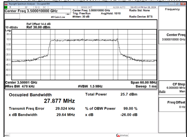
Band77-Part27_30MHz_CP_OFDM_SCS30kHz_16QAM_RB78_0_Chain0_CH633334
