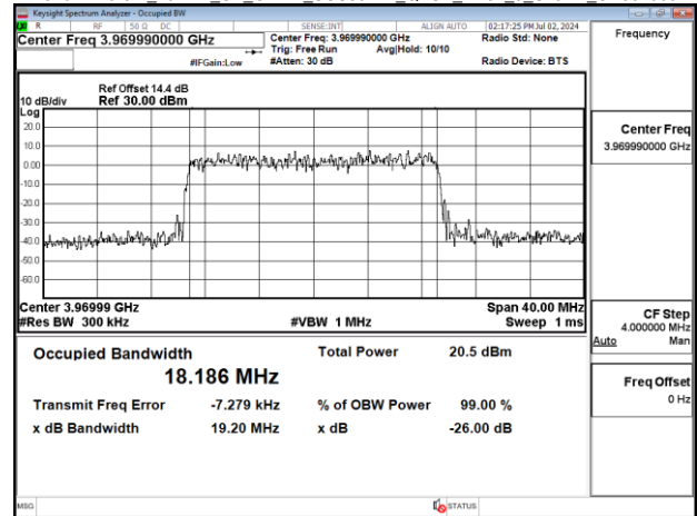
Band77-Part27_20MHz_CP_OFDM_SCS30kHz_16QAM_RB51_0_Chain0_CH63068
