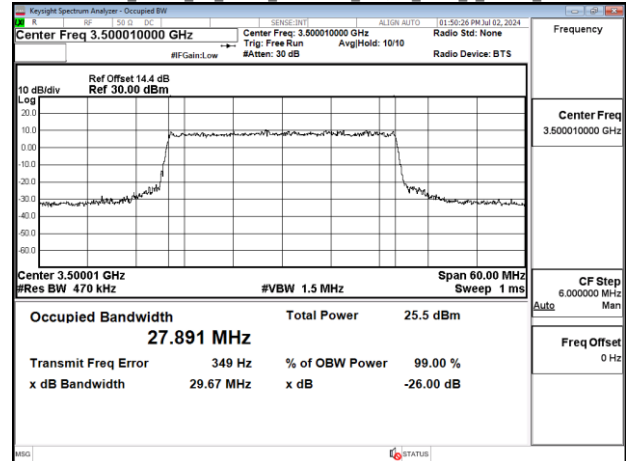
Band77-Part27_30MHz_CP_OFDM_SCS30kHz_16QAM_RB78_0_Chain1_CH633334
