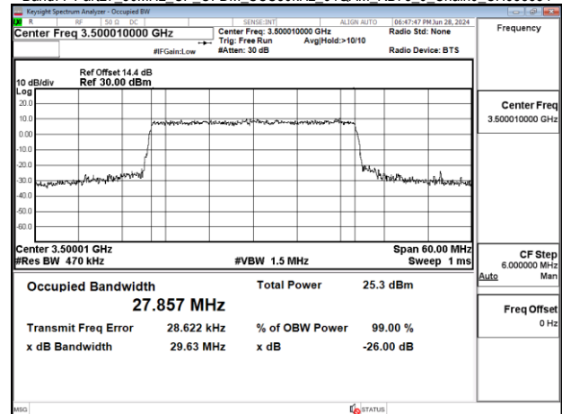
Band77-Part27_30MHz_CP_OFDM_SCS30kHz_64QAM_RB78_0_Chain0_CH633334
