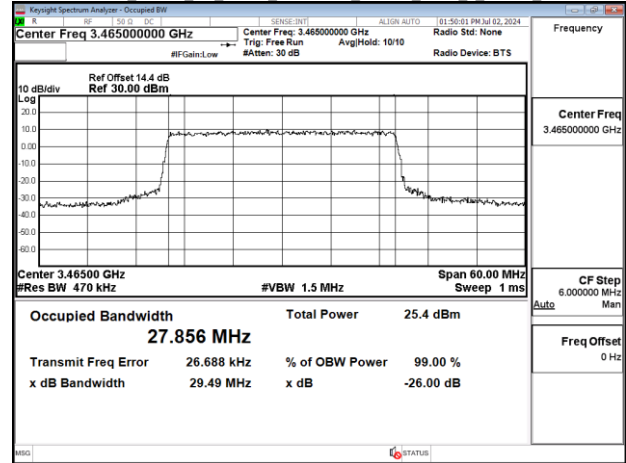
Band77-Part27_30MHz_CP_OFDM_SCS30kHz_16QAM_RB78_0_Chain1_CH633334
