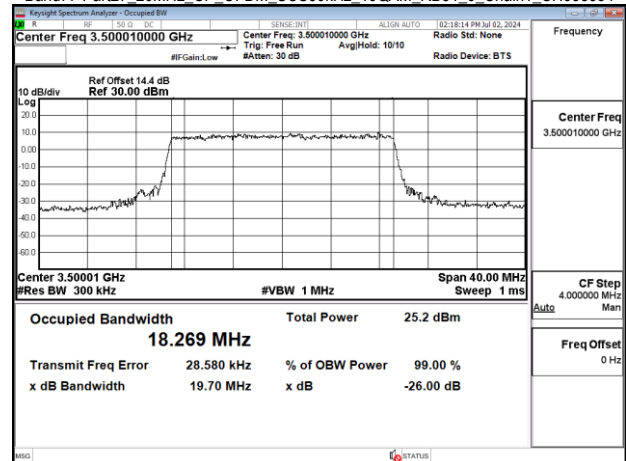
Band77-Part27_20MHz_CP_OFDM_SCS30kHz_16QAM_RB51_0_Chain1_CH633334
