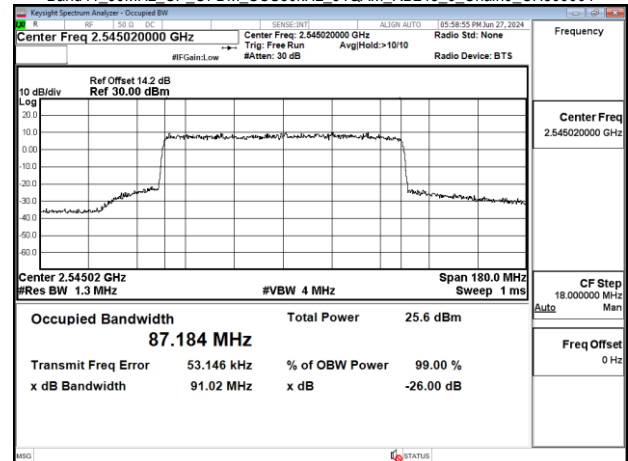
Band41_90MHz_CP_OFDM_SCS30kHz_64QAM_RB245_0_Chain0_CH509004
