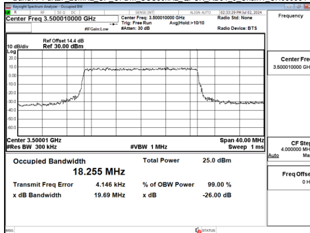
Band77-Part27_20MHz_CP_OFDM_SCS30kHz_QPSK_RB51_0_Chain1_CH633334
