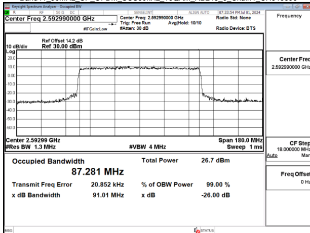
Band41_90MHz_CP_OFDM_SCS30kHz_16QAM_RB245_0_Chain1_CH518598
