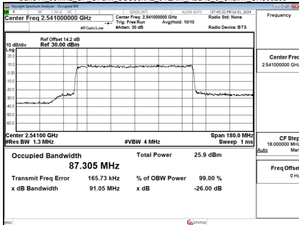
Band41_90MHz_CP_OFDM_SCS30kHz_64QAM_RB245_0_Chain1_CH508200
