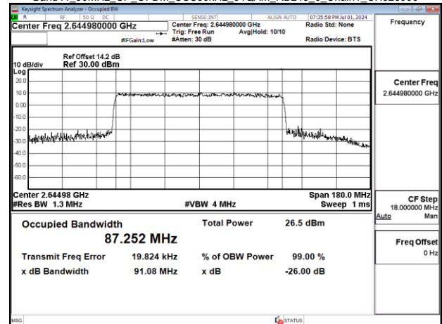
Band41_90MHz_CP_OFDM_SCS30kHz_64QAM_RB245_0_Chain1_CH528996
