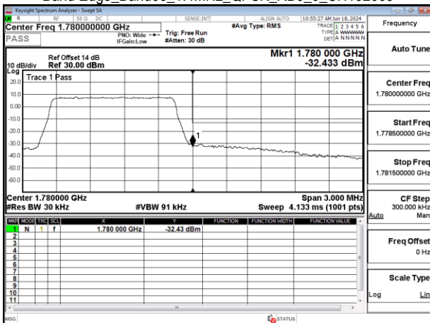
Band Edge_Band66_1.4MHz_QPSK_RB6_0_CH132665
