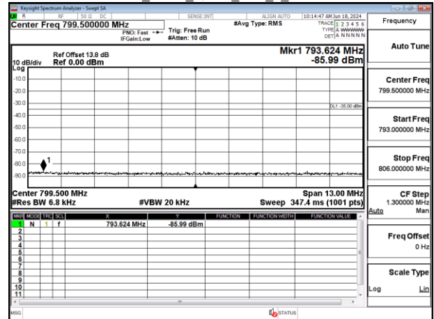
Band13 5MHz_QPSK_RB1_0_CH23230
