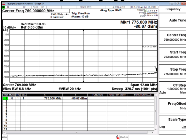
Band13 5MHz_QPSK_RB1_0_CH23230
