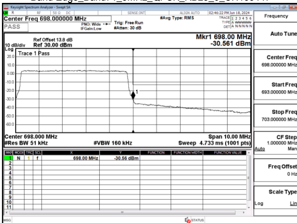
Band Edge_Band71_5MHz_QPSK_RB25_0_CH133447
