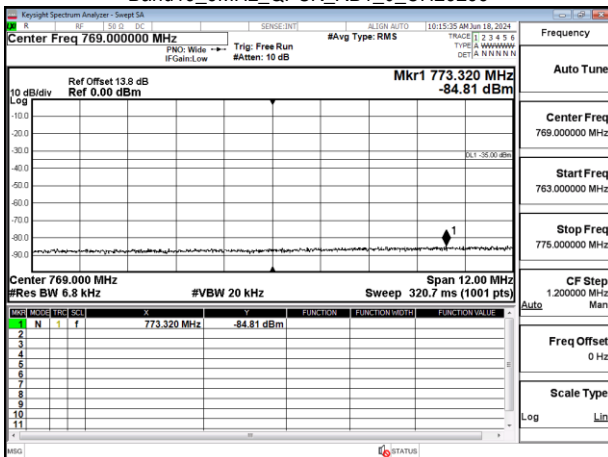
Band13 5MHz_QPSK_RB1_0_CH23255
