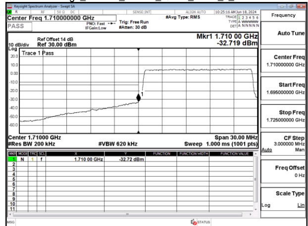
Band Edge_Band66_15MHz_QPSK_RB75_0_CH132047
