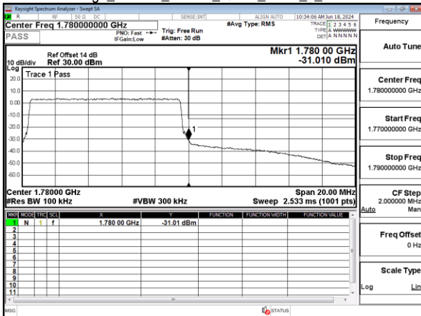
Band Edge_Band66_10MHz_QPSK_RB50_0_CH132622
