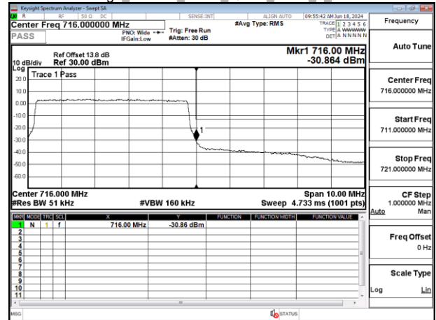
Band Edge_Band12_10MHz_QPSK_RB1_0_CH23060
