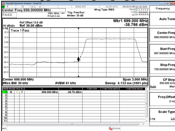
Band Edge_Band12_1.4MHz_QPSK_RB6_0_CH23173
