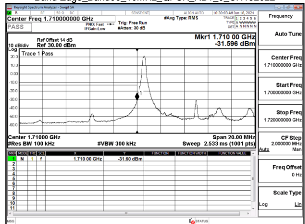
Band Edge_Band66_10MHz_QPSK_RB1_0_CH132022
