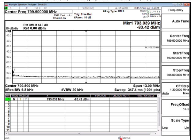
Band13 5MHz_QPSK_RB1_0_CH23255
