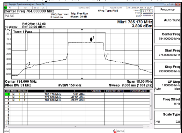
Band Edge_Band13_5MHz_QPSK_RB25_0_CH23255
