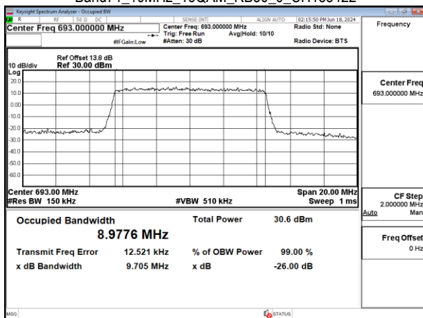
Band71_10MHz_16QAM_RB50_0_CH133422
