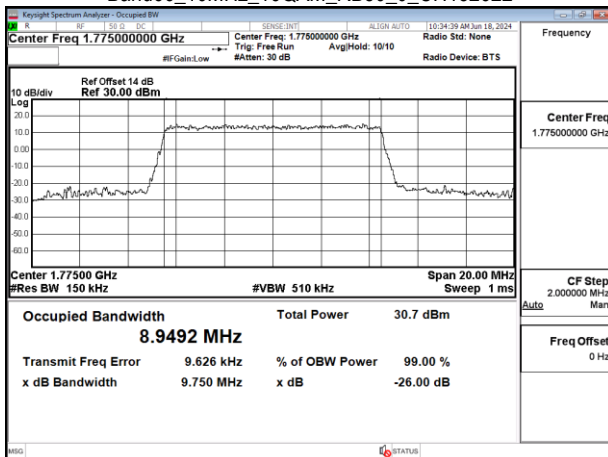
Band66_10MHz_16QAM_RB50_0_CH132622
