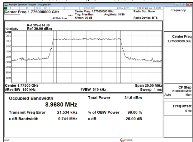
Band66_10MHz_QPSK_RB50_0_CH132622
