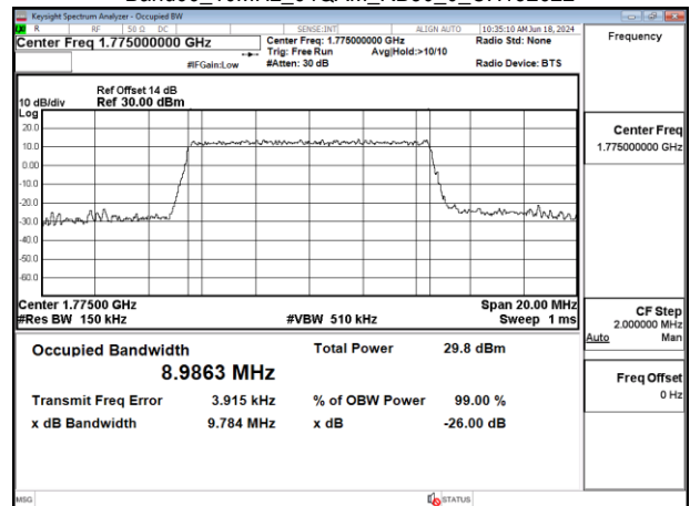
Band66_10MHz_64QAM_RB50_0_CH132622
