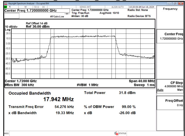
Band66_20MHz_QPSK_RB100_0_CH132322
