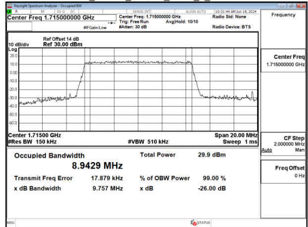
Band66_10MHz_64QAM_RB50_0_CH132322
