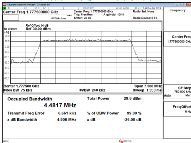
Band66_5MHz_64QAM_RB25_0_CH132647
