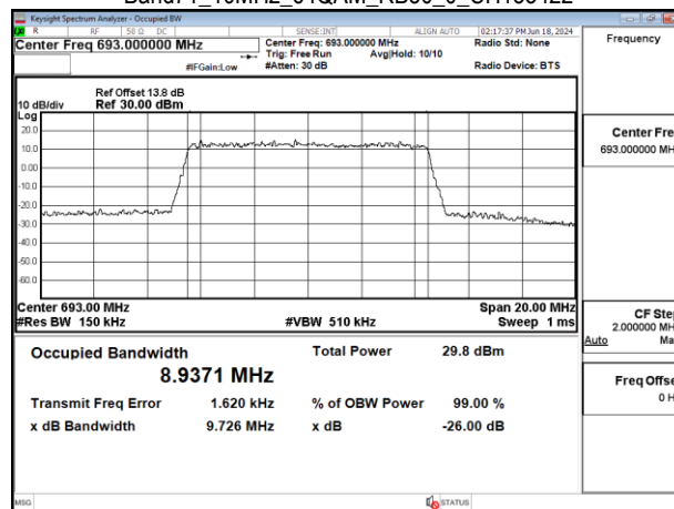
Band71_10MHz_64QAM_RB50_0_CH133422
