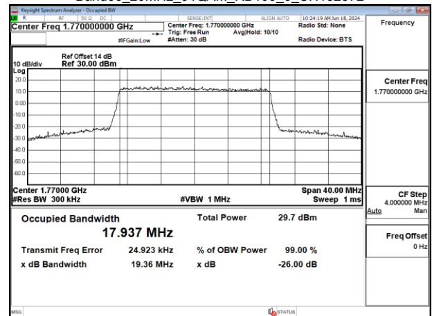
Band66 20MHz_64QAM_RB100_0_CH132572
