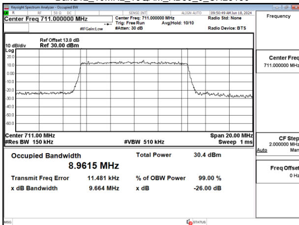
Band12_10MHz_16QAM_RB50_0_CH23130
