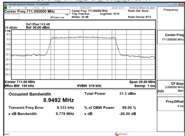
Band12_10MHz_QPSK_RB50_0_CH23130
