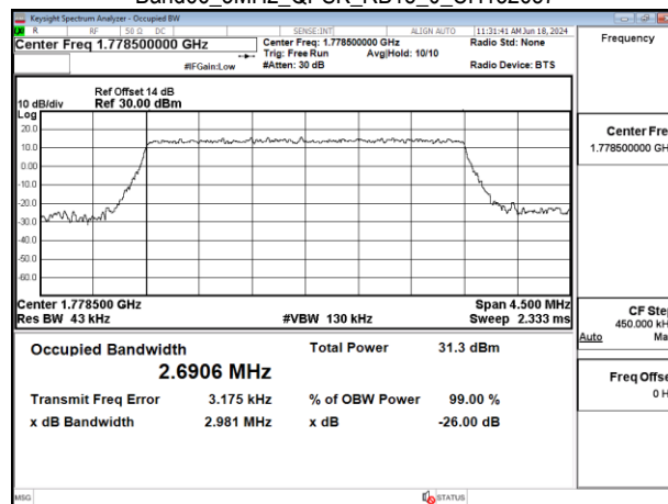
Band66_3MHz_QPSK_RB15_0_CH132657
