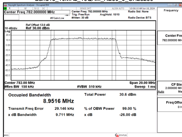
Band13_10MHz_64QAM_RB50_0_CH23230
