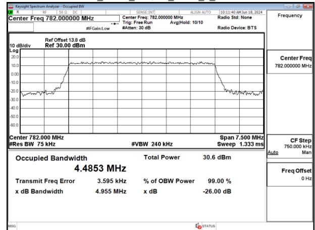
Band13_5MHz_16QAM_RB25_0_CH23255
