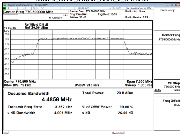
Band13_5MHz_64QAM_RB25_0_CH23230
