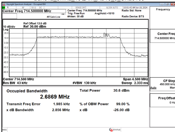
Band12_3MHz_16QAM_RB15_0_CH23165
