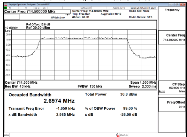
Band12_3MHz_QPSK_RB15_0_CH23165
