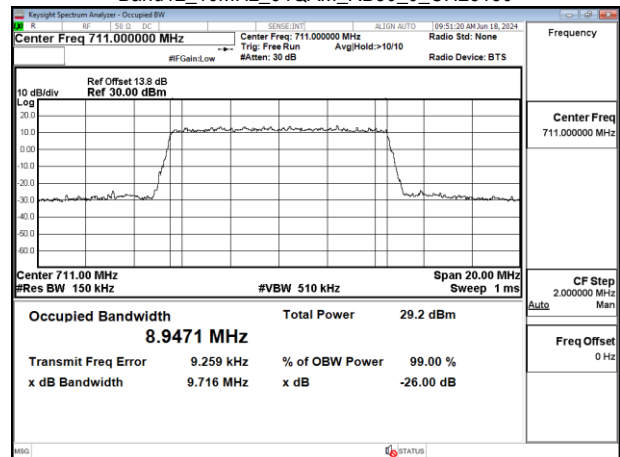
Band12_10MHz_64QAM_RB50_0_CH23130
