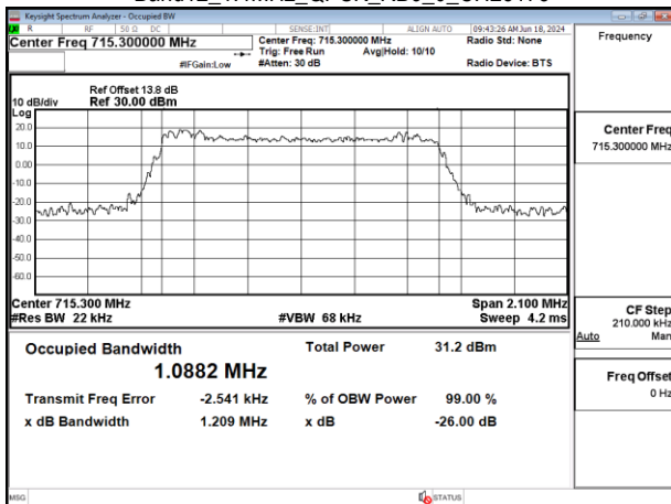
Band12_1.4MHz_QPSK_RB6_0_CH23173
