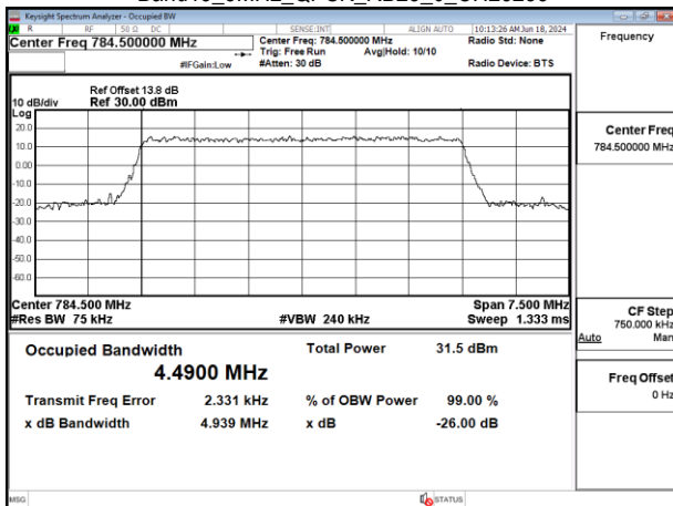
Band13_5MHz_QPSK_RB25_0_CH23255
