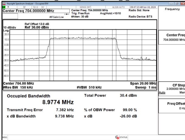
Band12_10MHz_16QAM_RB50_0_CH23095
