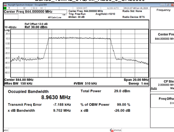
Band5_10MHz_64QAM_RB50_0_CH20600
