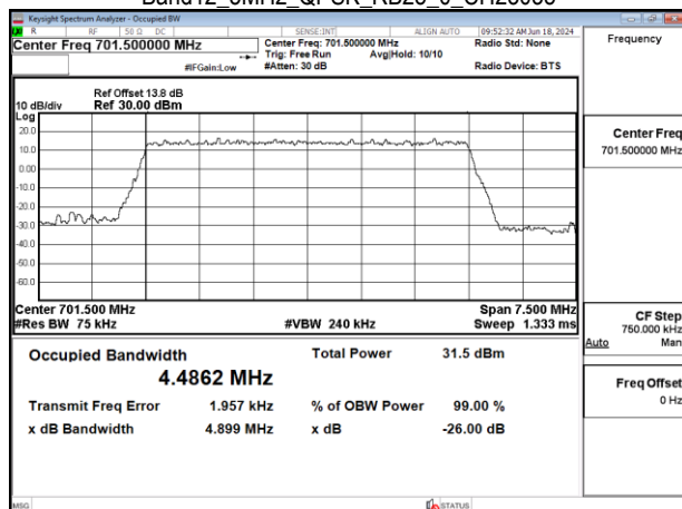
Band12_5MHz_QPSK_RB25_0_CH23095
