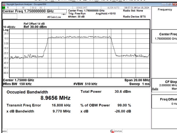
Band4_10MHz_16QAM_RB50_0_CH20350
