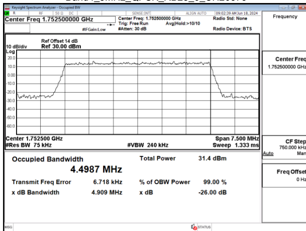
Band4_5MHz_QPSK_RB25_0_CH20375
