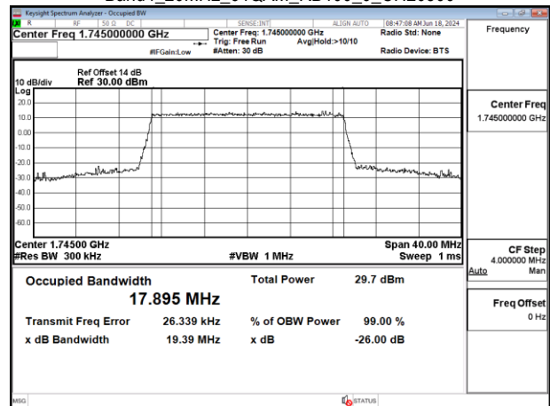
Band4_20MHz_64QAM_RB100_0_CH20300
