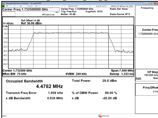
Band4_5MHz_64QAM_RB25_0_CH20375
