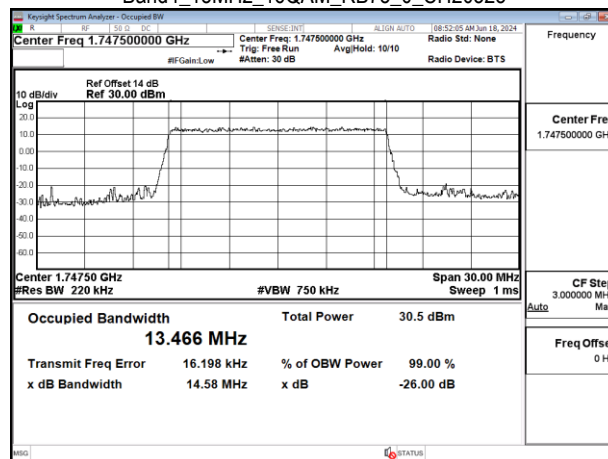
Band4_15MHz_16QAM_RB75_0_CH20325
