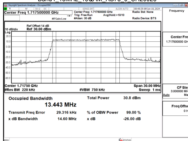
Band4_15MHz_16QAM_RB75_0_CH20175
