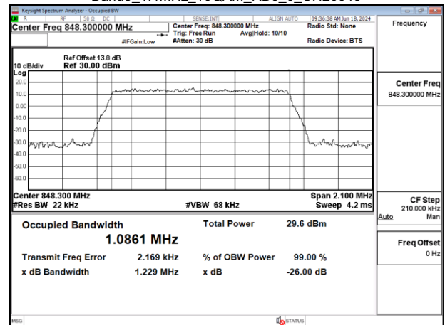
Band5_1.4MHz_16QAM_RB6_0_CH20643
