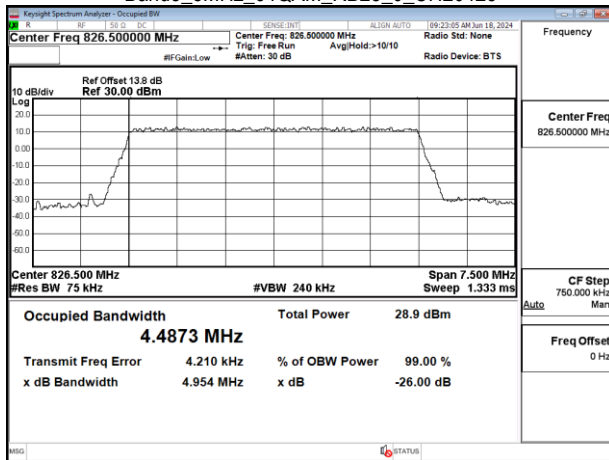
Band5_5MHz_64QAM_RB25_0_CH20525
