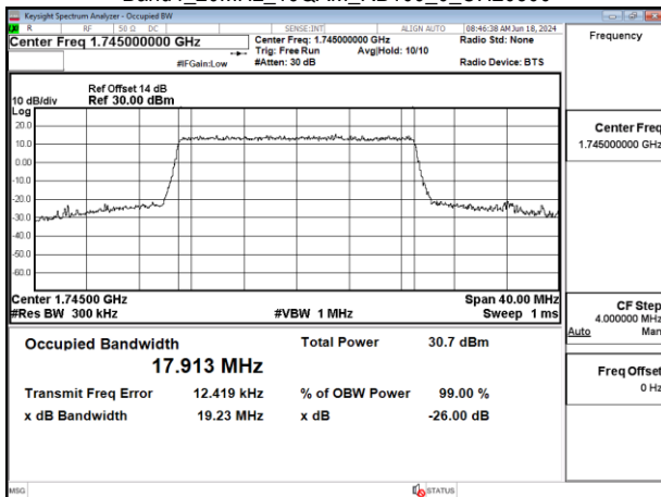
Band4_20MHz_16QAM_RB100_0_CH20300
