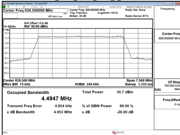
Band5_5MHz_QPSK_RB25_0_CH20525
