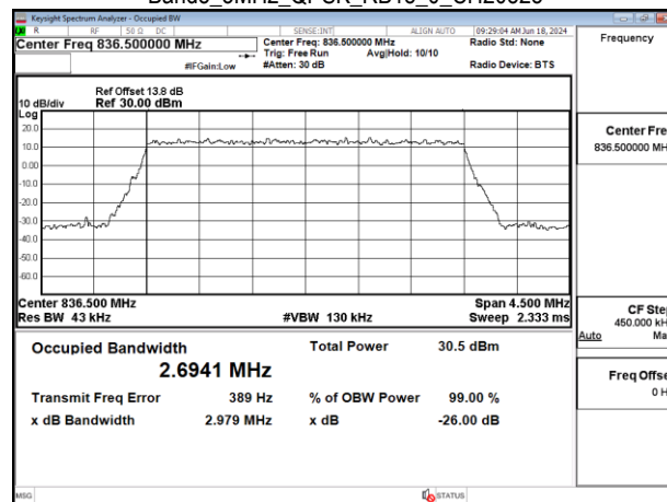
Band5_3MHz_QPSK_RB15_0_CH20635
