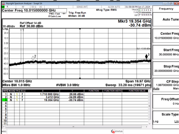
Band4_1.4MHz_QPSK_RB1_0_CH20175
