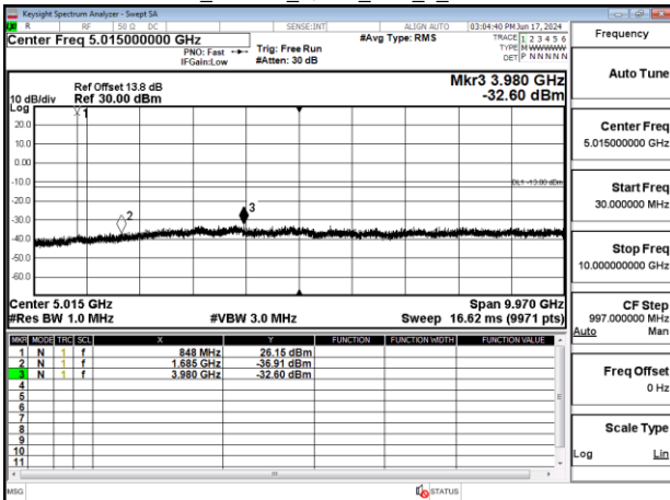
Band5_1.4MHz_QPSK_RB1_0_CH20643
