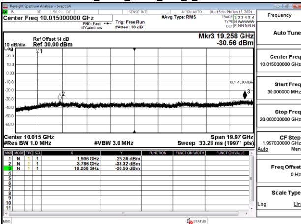
Band2_5MHz_QPSK_RB1_0_CH19175
