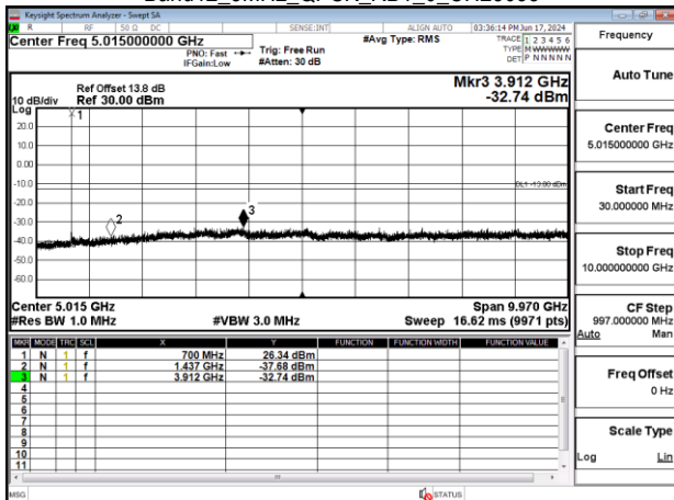
Band12_5MHz_QPSK_RB1_0_CH23095
