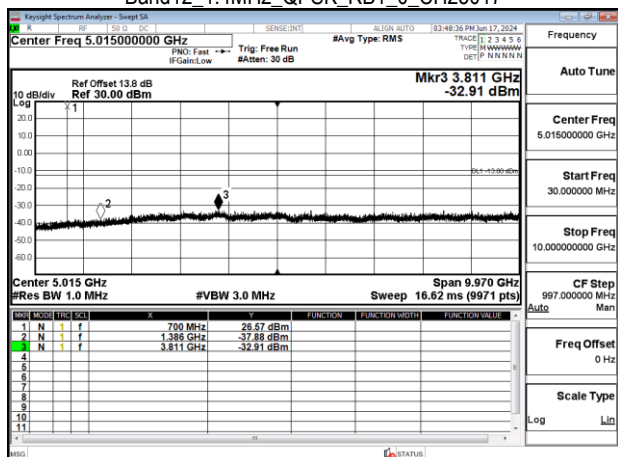
Band12_1.4MHz_QPSK_RB1_0_CH23095
