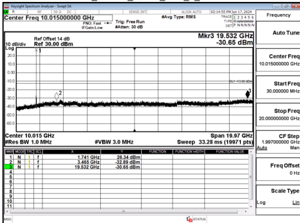
Band4_15MHz_QPSK_RB1_0_CH20325
