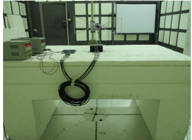
4G_Radiated_Setup
