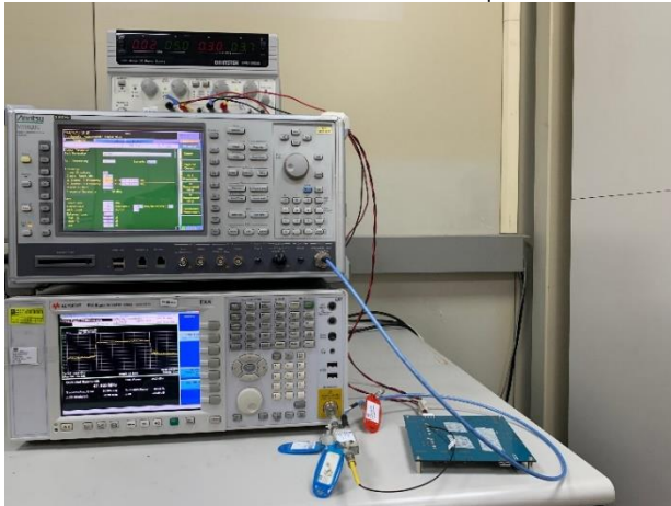
2G&3G_Conducted_SIM2_Setup
