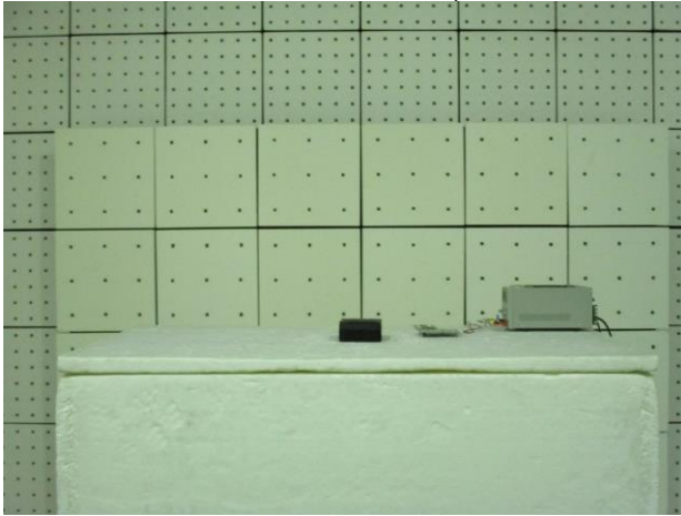
2G&3G_Radiated_Setup
