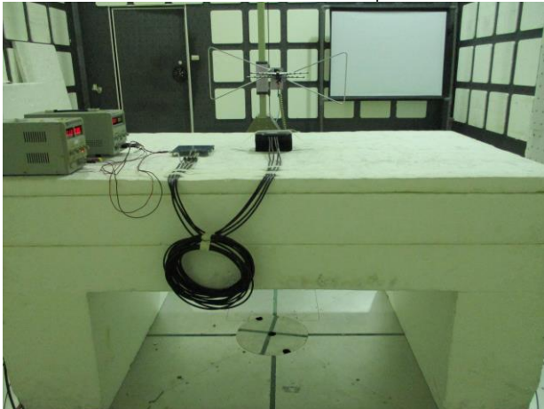
5G&ENDC_Radiated_Setup
