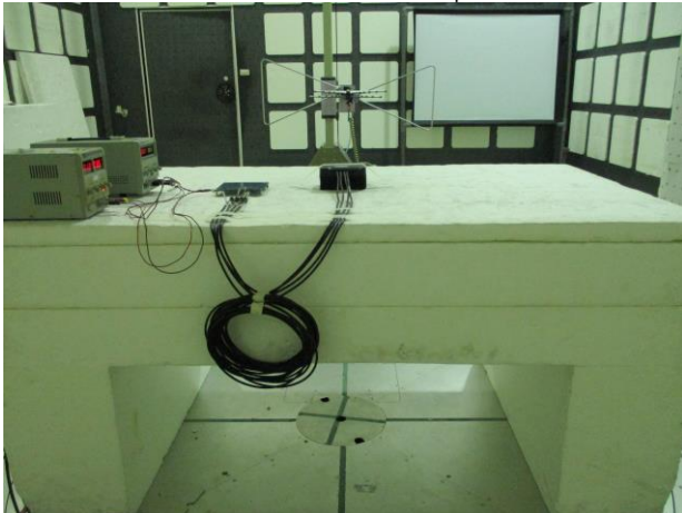
2G&3G_Radiated_Setup
