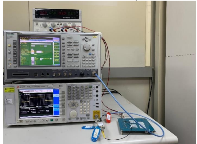
4G_Conducted_SIM2_Setup
