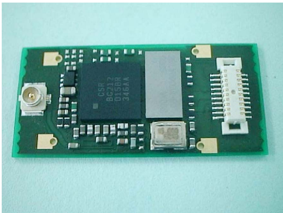
Bluetooth Module without Shield
