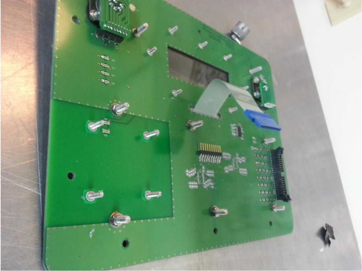
Display Panel Bottom – Showing Under Membrane Tail
