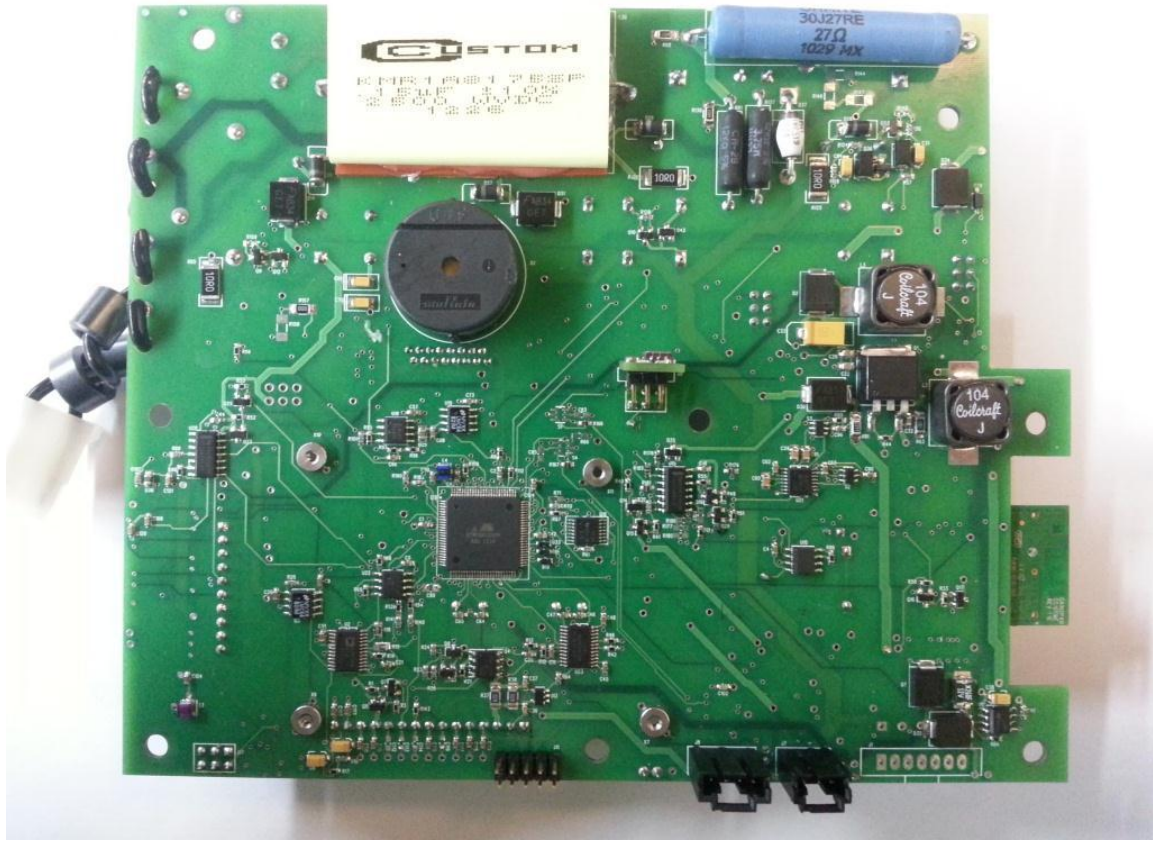
Microcontroller PCBA – Bottom
