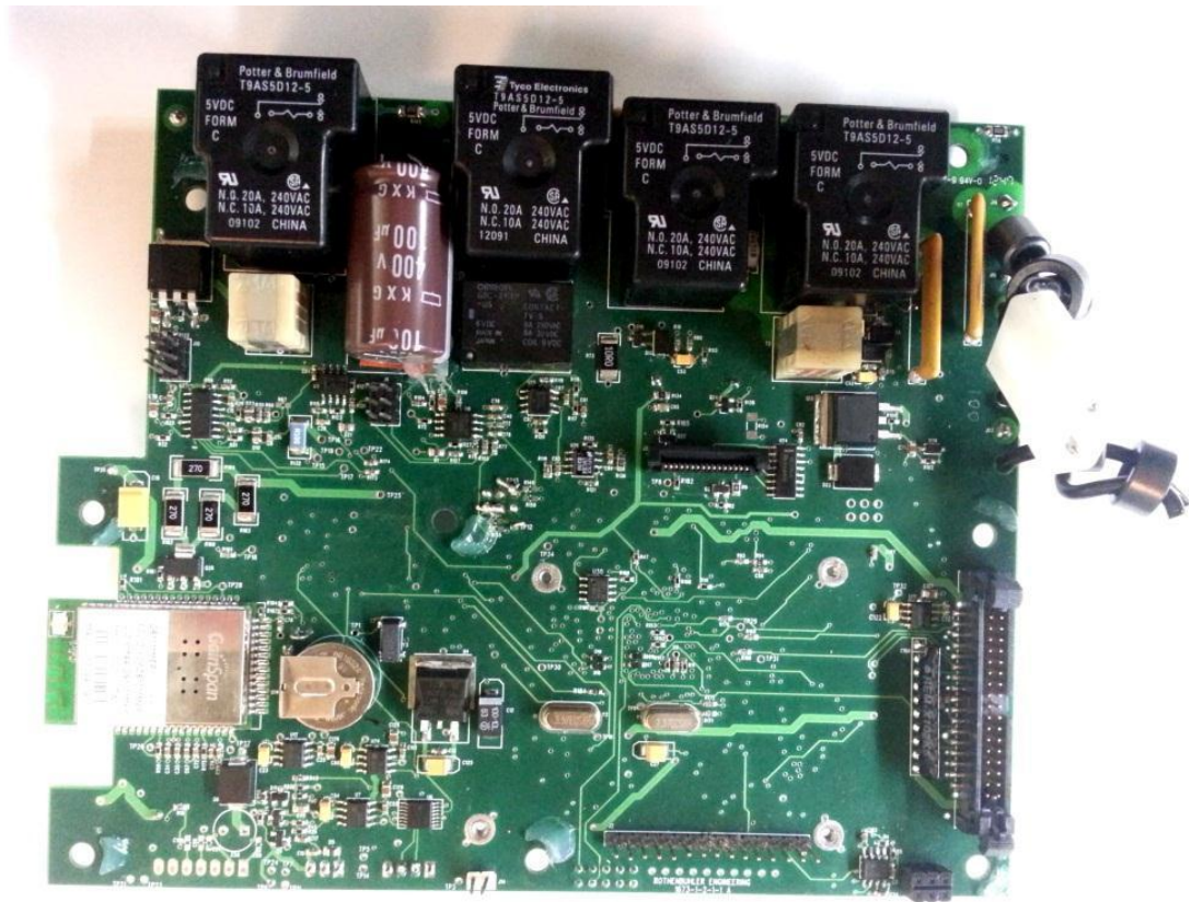
Microcontroller PCBA - Top
