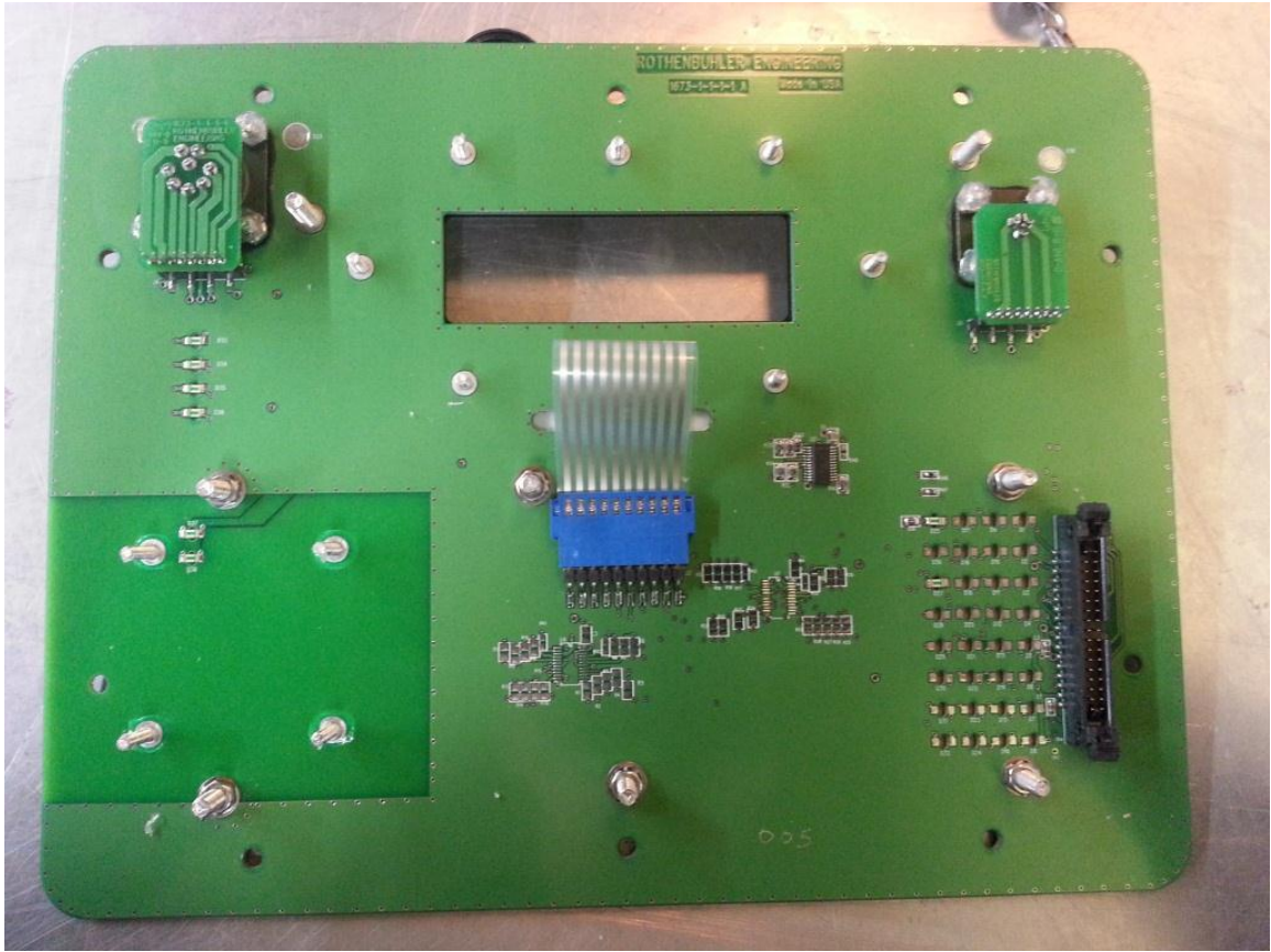
Display Panel PCBA – Bottom
