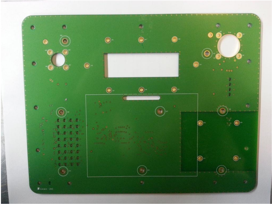
Display Panel PCBA Top no Decal (All component are bottom mounted)
