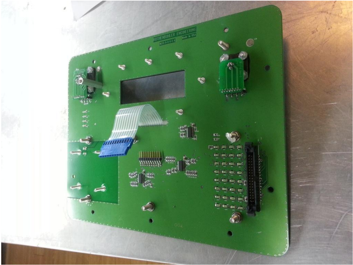
Display Panel PCBA – Bottom Shows Under Membrane Tail
