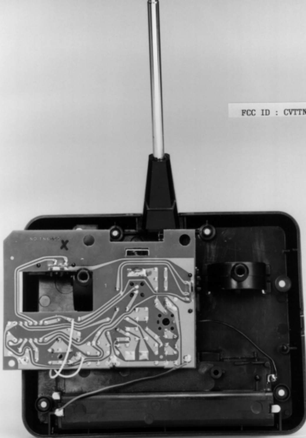
Main PC Board, Foil Side
