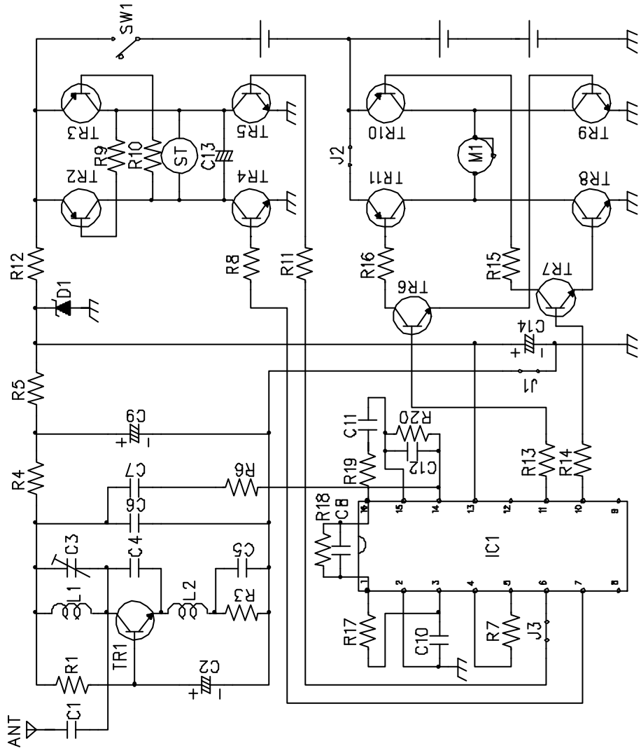
NO.RP7420 CIRCUIT DIAGRAM
