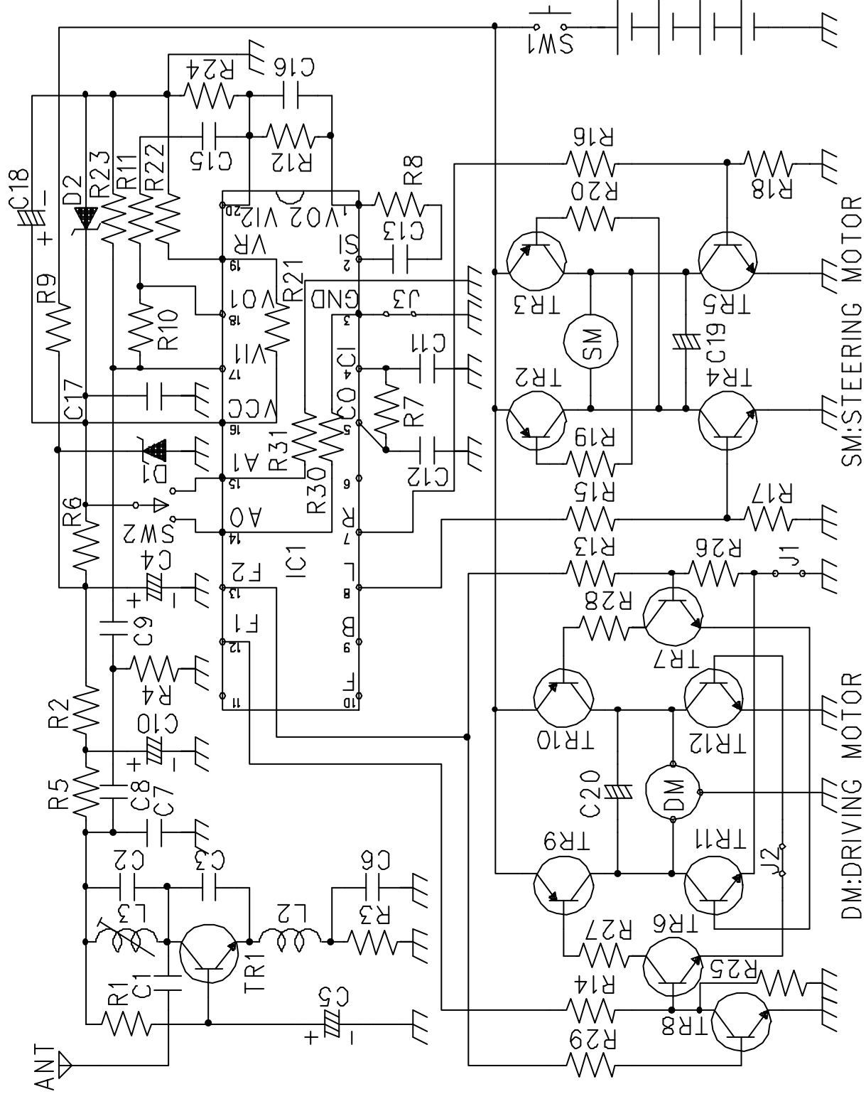
FCC ID:CVTRP7370H CIRCUIT DIAGRAM
