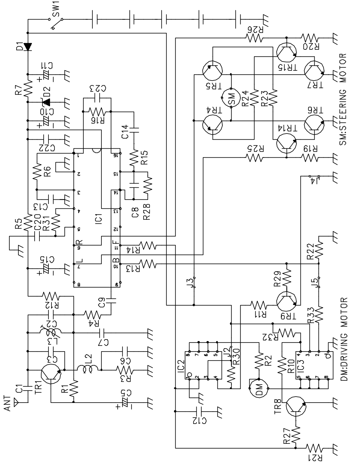
NO.RP7320 CIRCUIT DIAGRAM
