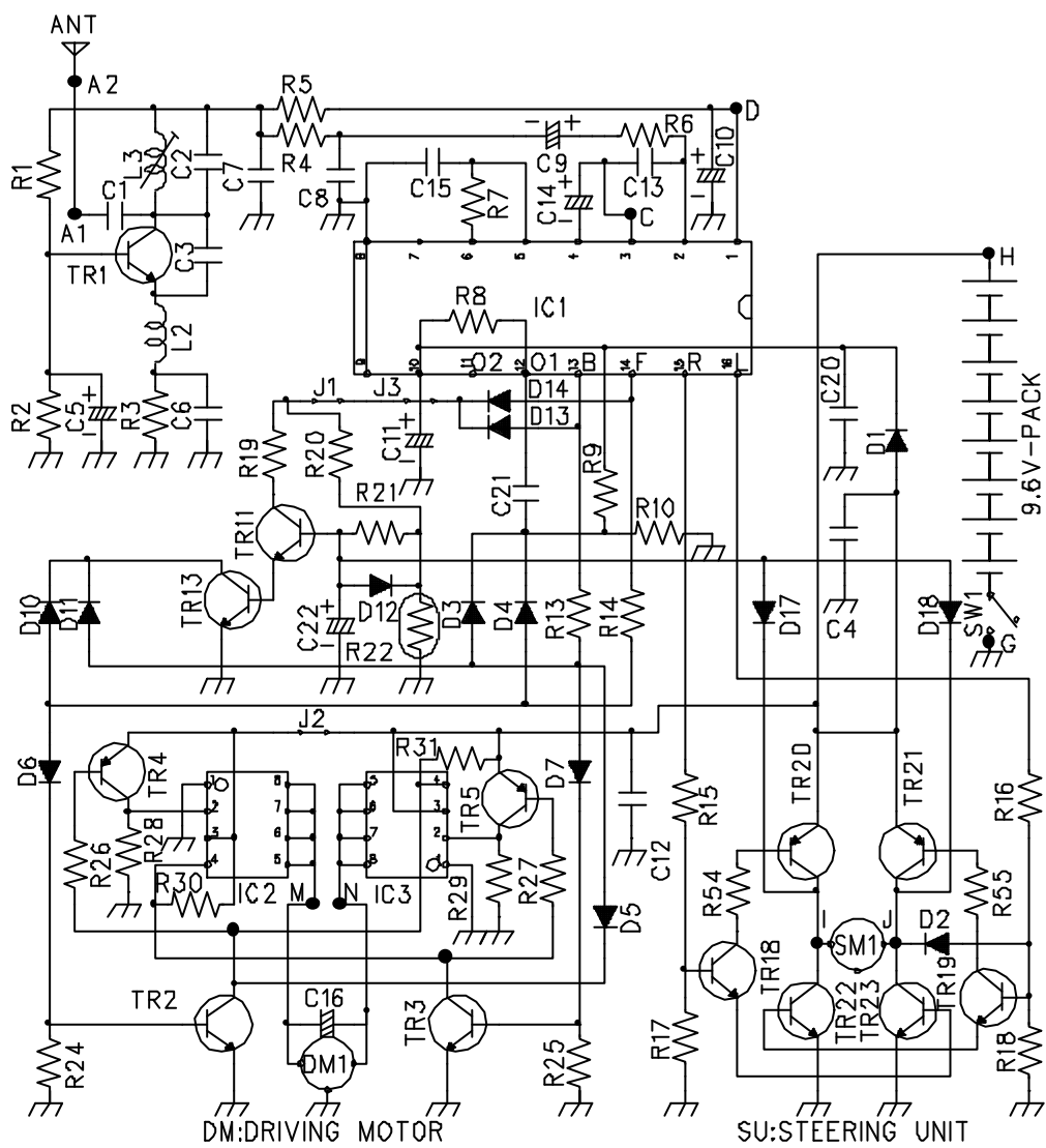
NO.RN6201T(2) CIRCUIT DIAGRAM
