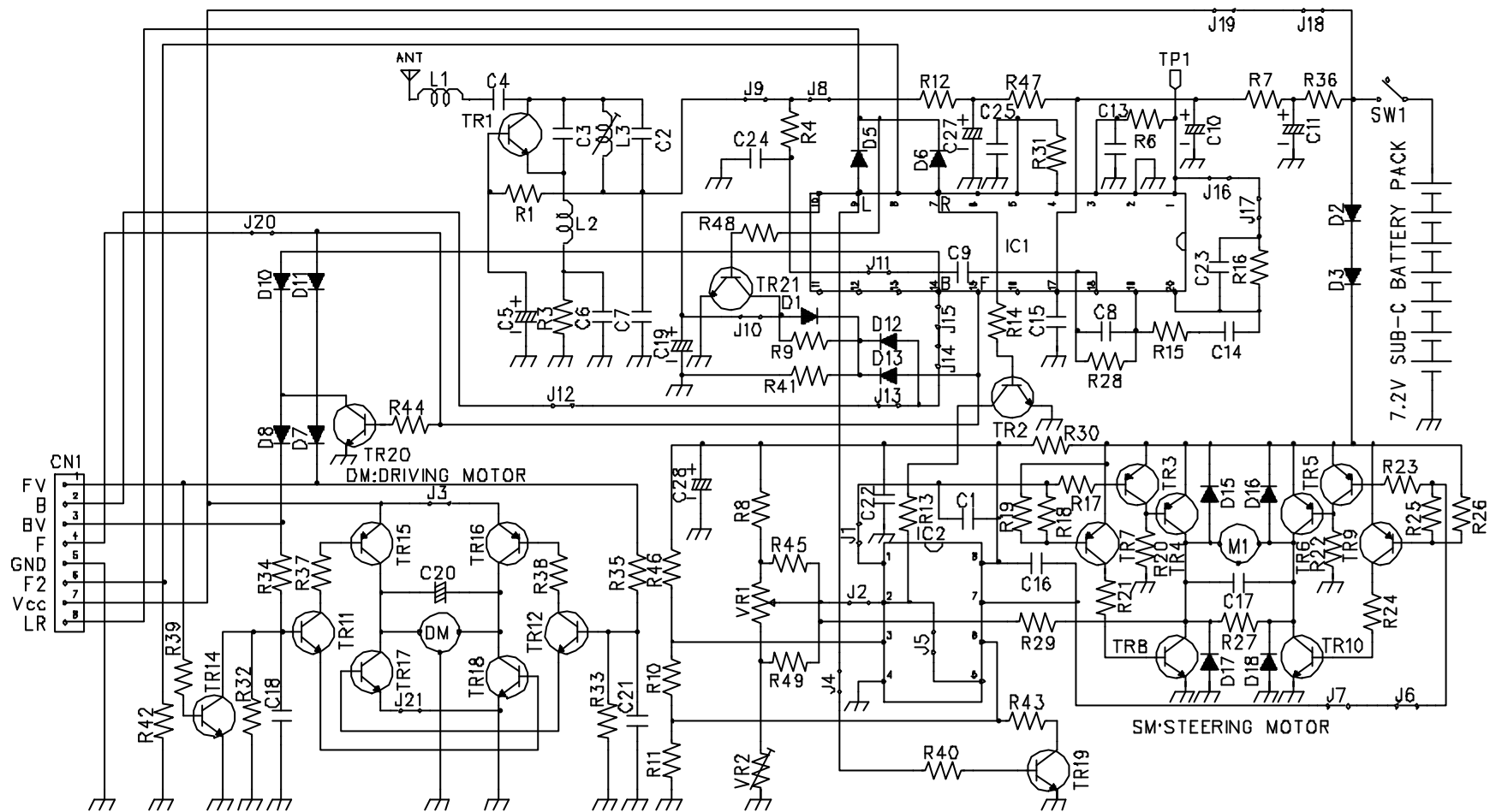
NO.RA6441 CIRCUIT DIAGRAM FCC ID:CVTRA6441H
