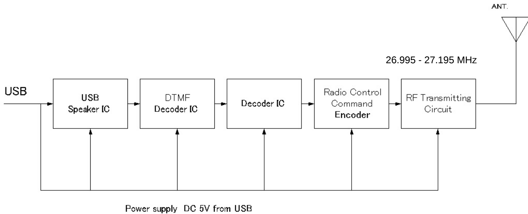
NO.MR2D2TX Block diagram
