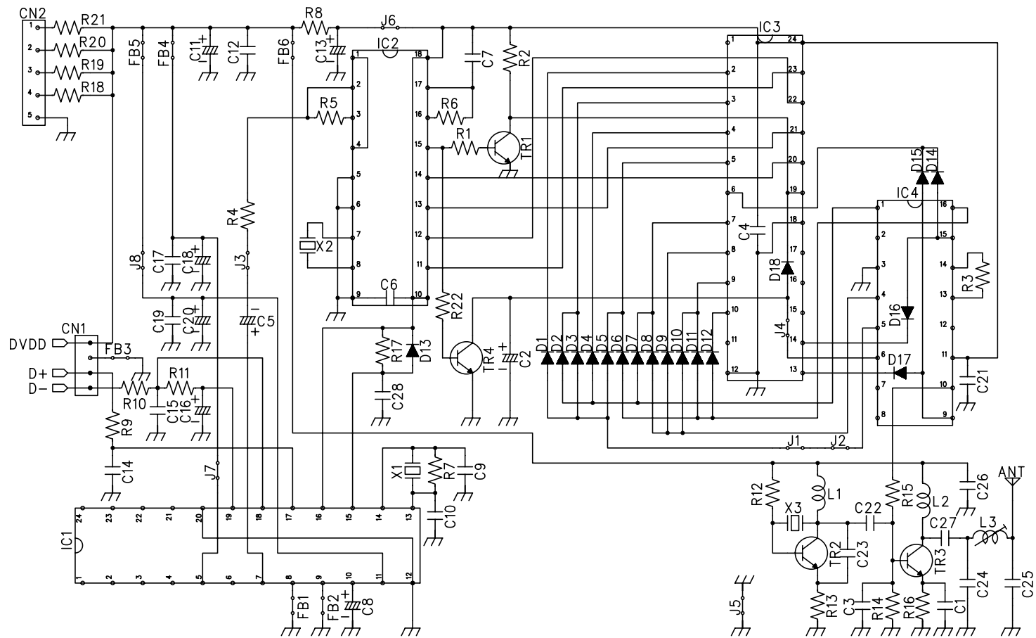
NO.MR2D2TX Circuit diagram
