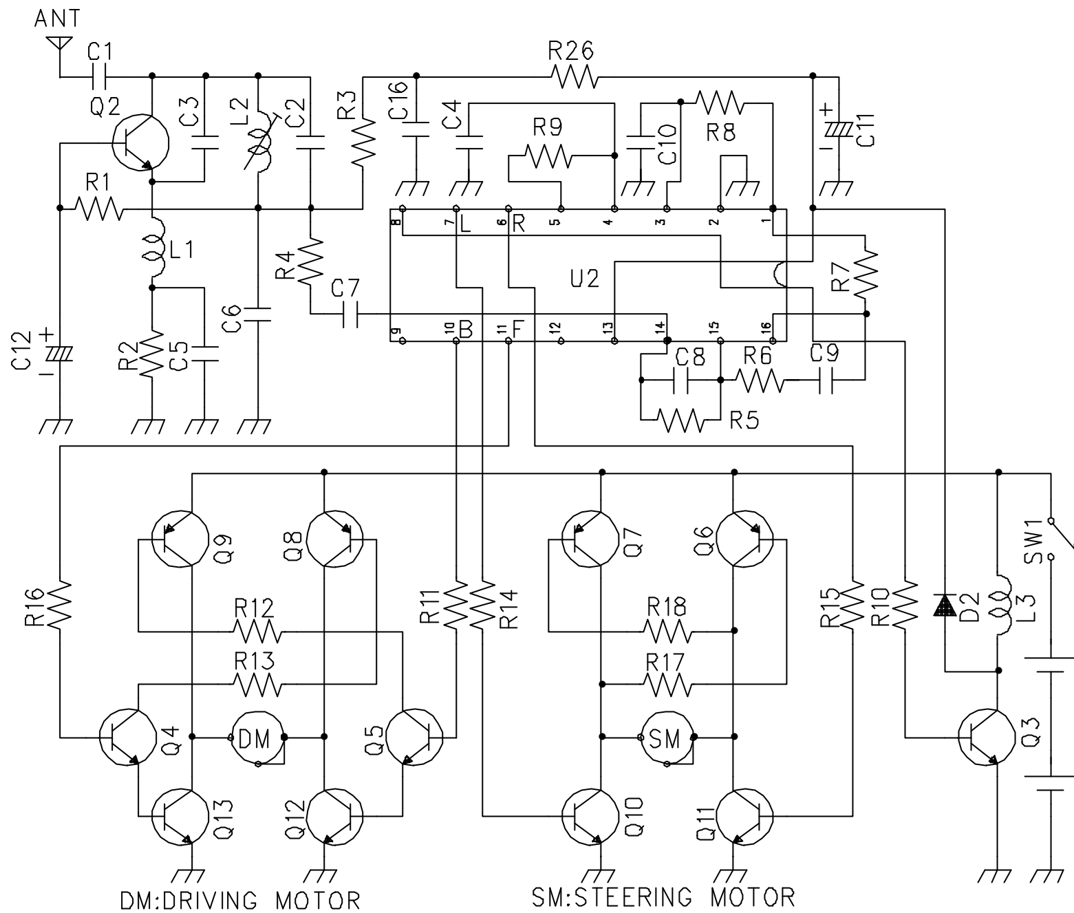
NO.0517RX CIRCUIT DIAGRAM (FCC ID:CVT0517R)
