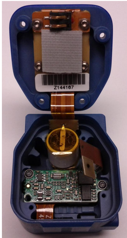
Boards inside enclosure
