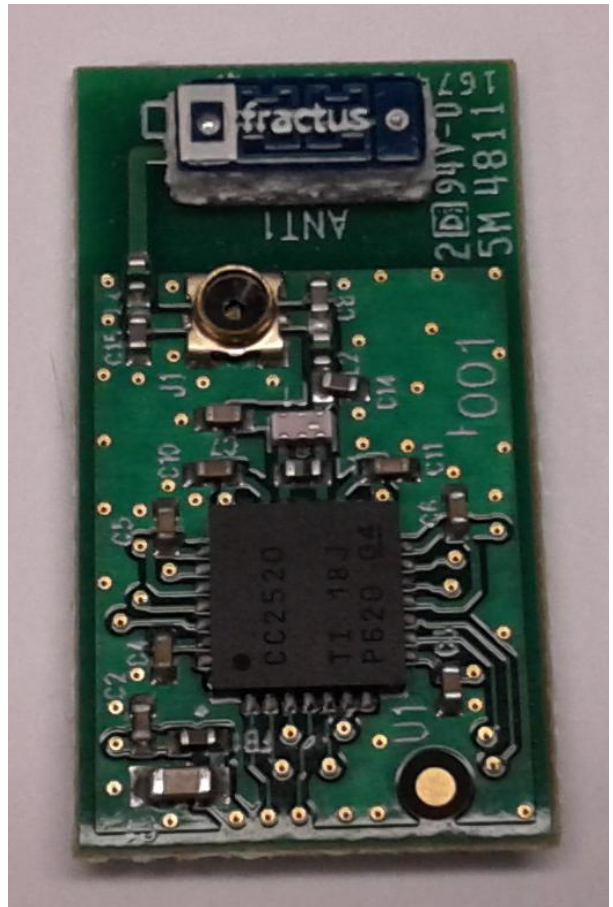
Radio Board
