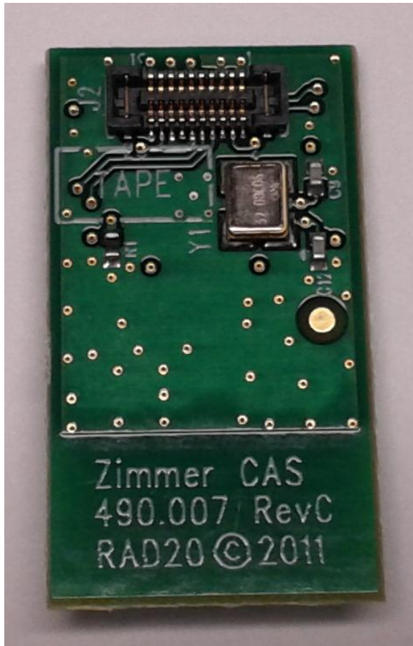
Radio Board
