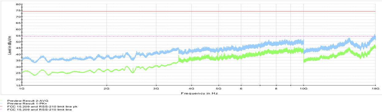
Figure 8.7-11: Radiated spurious emissions 1 to18 GHz, High channel
