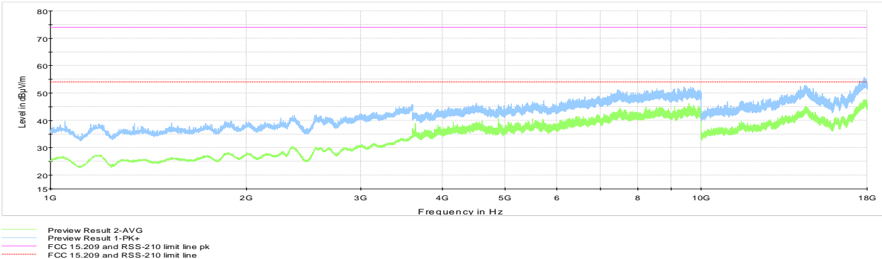
Figure 8.7-10: Radiated spurious emissions 1 to18 GHz, mid channel
