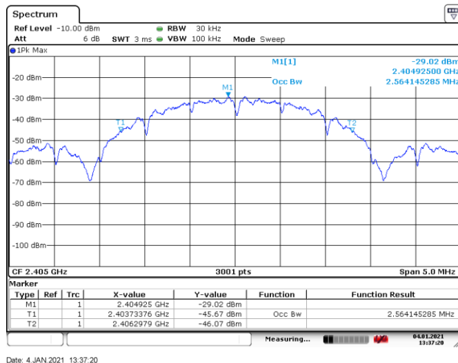
Figure 8.4-4: 99% occupied bandwidth, Tx on low channel
