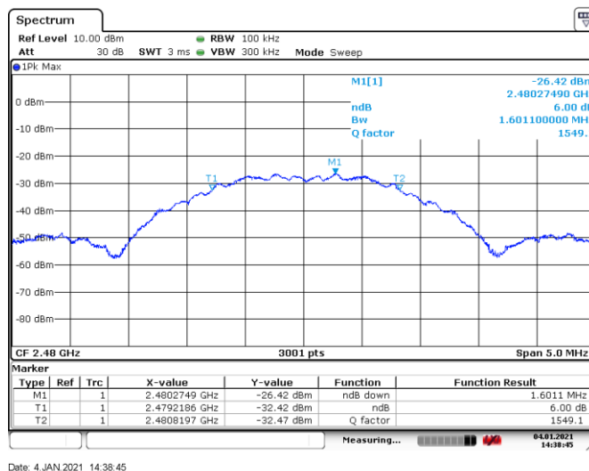
Figure 8.4-3: 6 dB bandwidth, Tx on high channel
