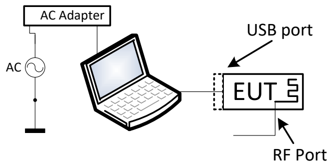
Figure 5.5-2: Antenna port testing block diagram
