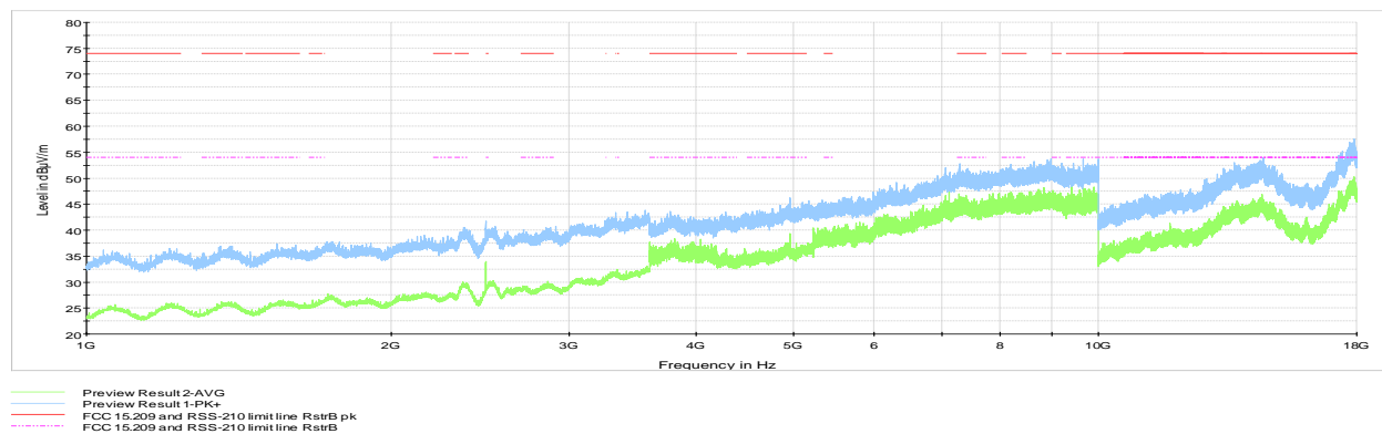
Figure 8.6-11: Radiated spurious emissions 1 to 18 GHz, High channel
