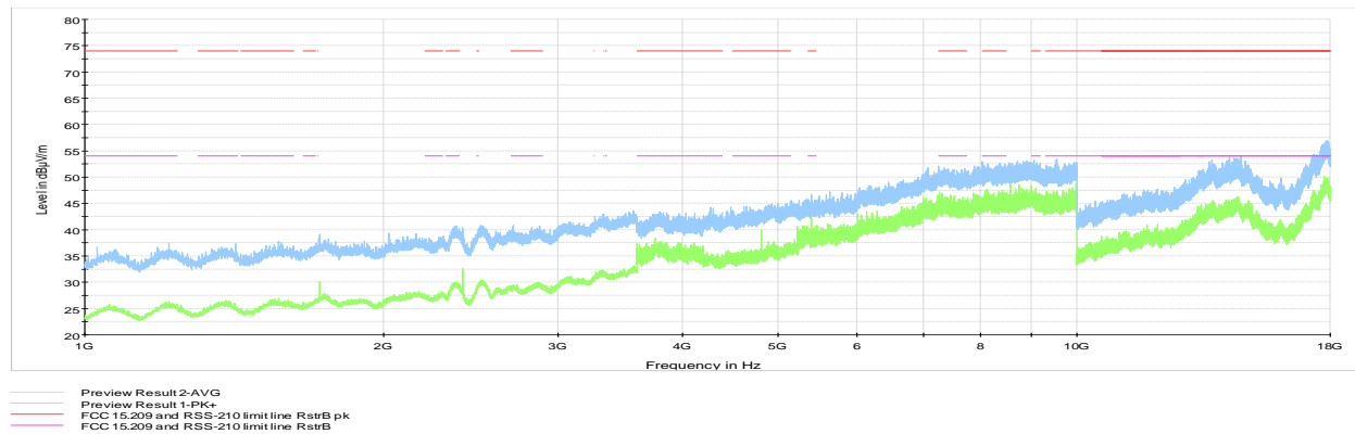
Figure 8.6-9: Radiated spurious emissions 1 to 18 GHz, Low channel
