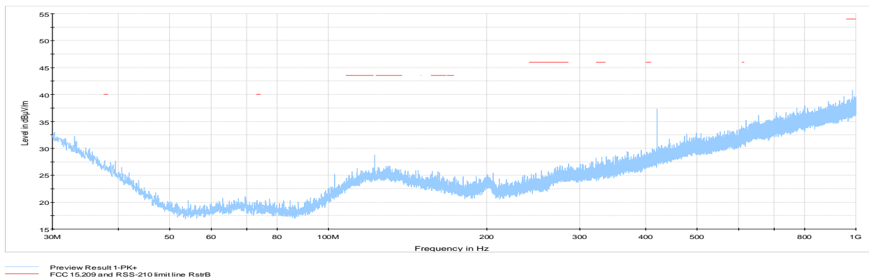
Figure 8.6-8: Radiated spurious emissions 30 MHz to 1 GHz, High channel
