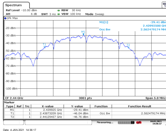
Figure 8.4-5: 99% occupied bandwidth, Tx on mid channel
