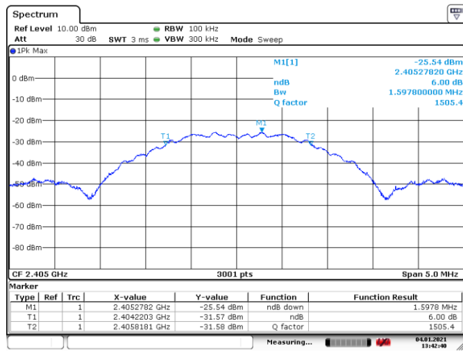
Figure 8.4-1: 6 dB bandwidth, Tx on low channel
