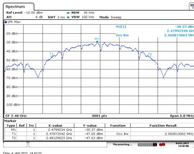
Figure 8.4-6: 99% occupied bandwidth, Tx on high channel
