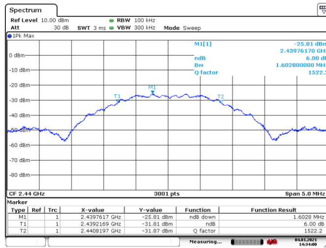
Figure 8.4-2: 6 dB bandwidth, Tx on mid channel
