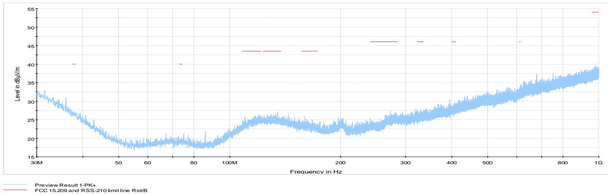
Figure 8.6-6: Radiated spurious emissions 30 MHz to 1 GHz, Low channel
