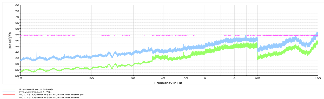
Figure 8.6-10: Radiated spurious emissions 1 to 18 GHz, mid channel
