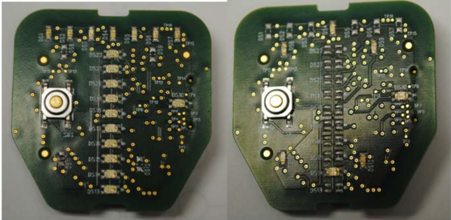
Figure 3 User Interface board top side, left is Cut Guide type, right is Reference type
