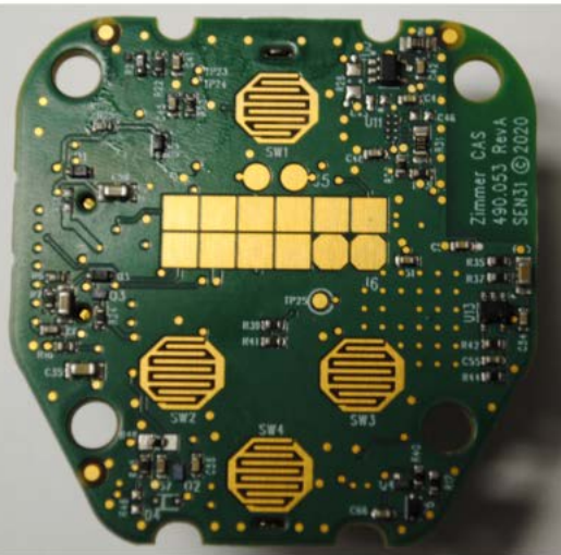
Figure 2 Sensor board top and bottom side
