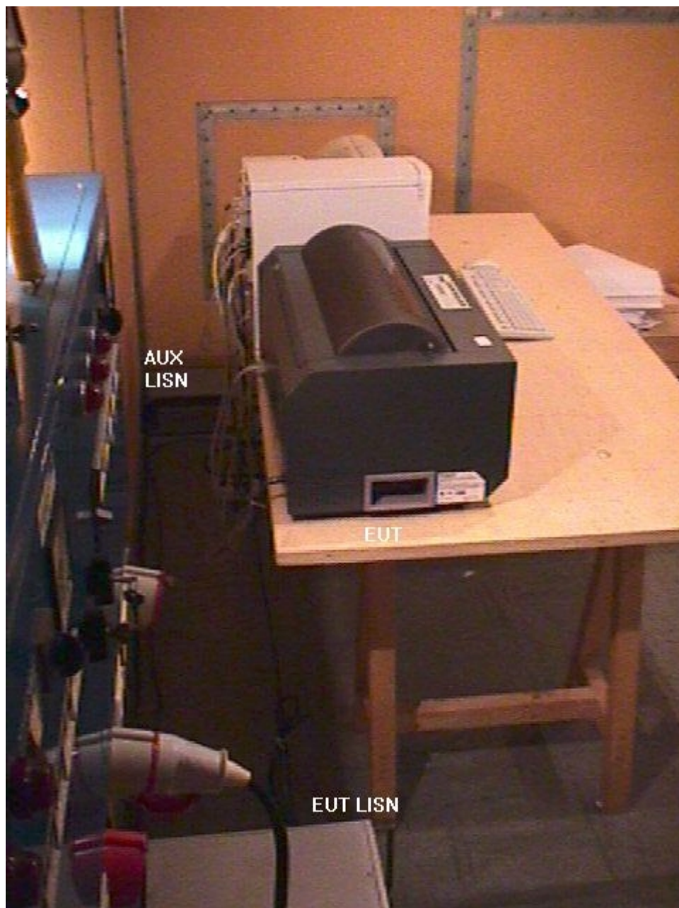
picture 5: conducted measurement rear view serial transmission
