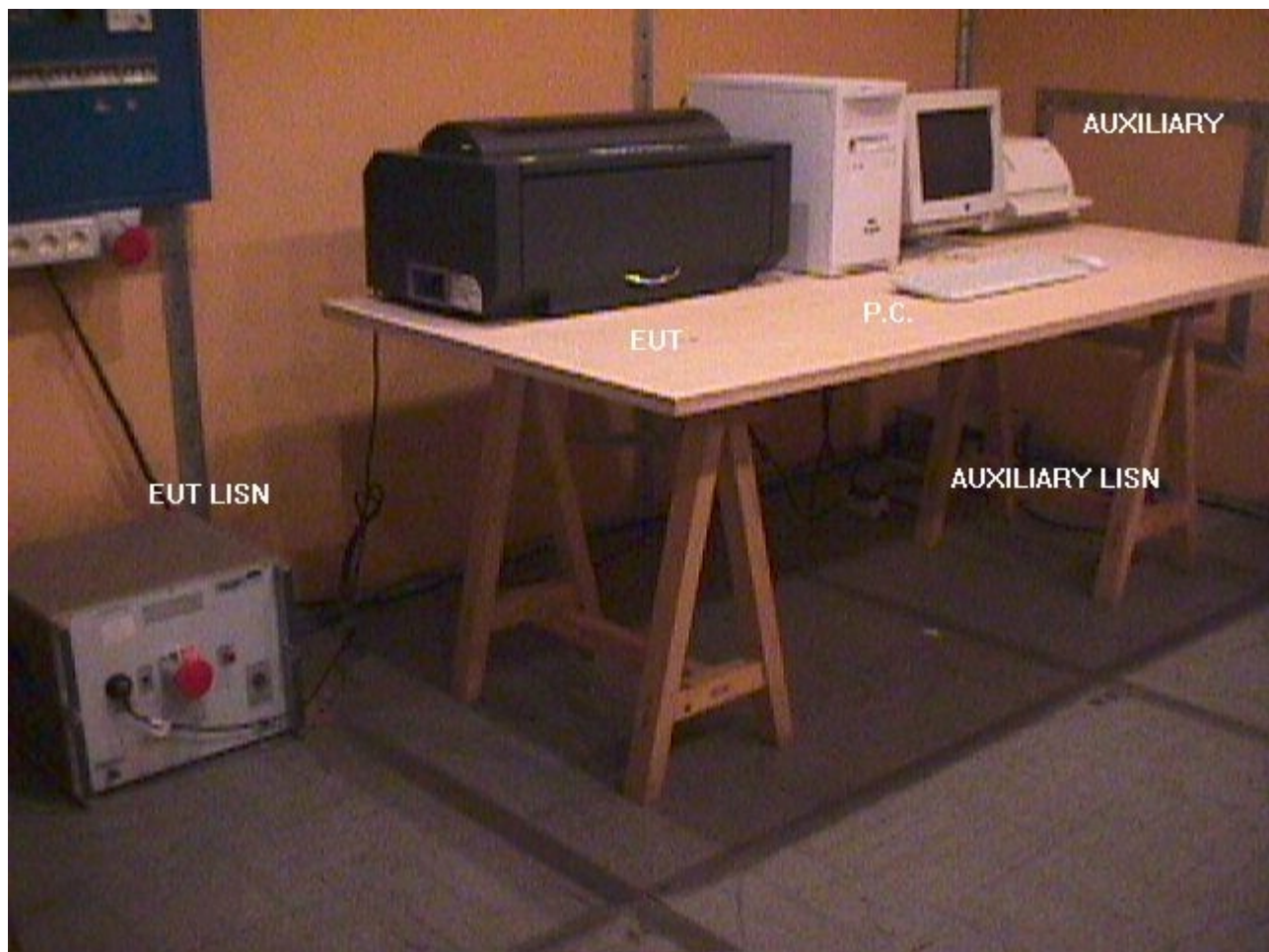
picture 4: conducted measurement front view
