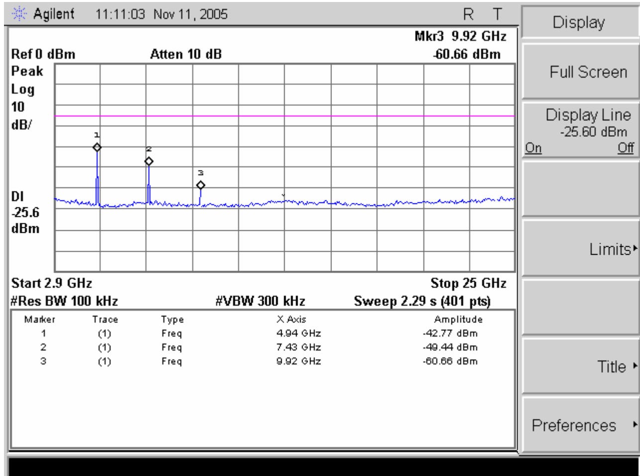
Plot 18. Channel 78 Spurious Conducted Emissions Test Plot (3)
