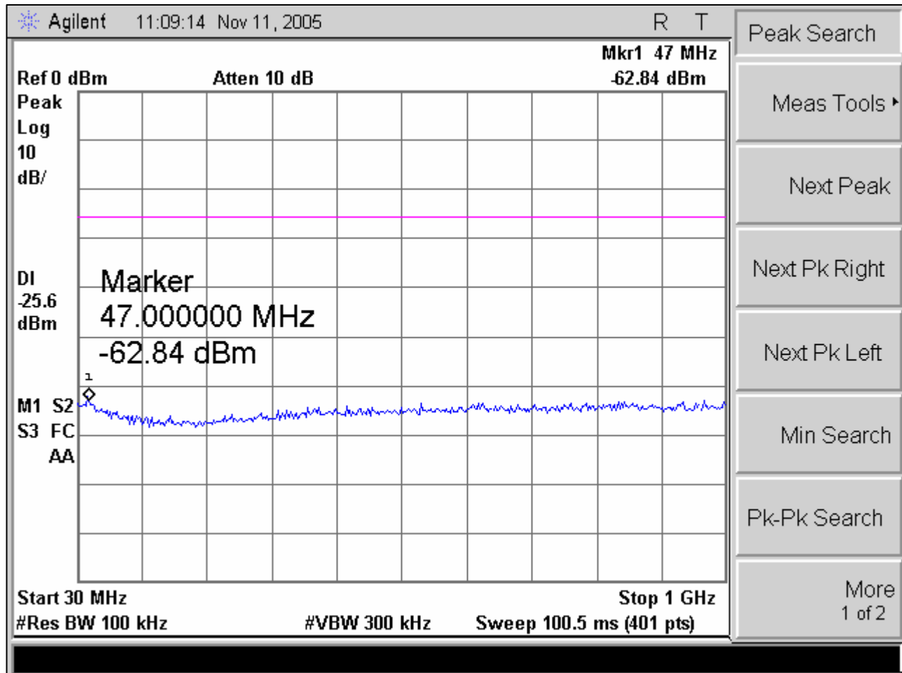
Plot 12. Channel 78 Spurious Conducted Emission Test Plot (1)
