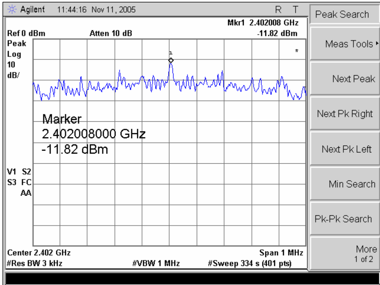
Plot 19. Power Spectral Density Test Results (Channel 1)
