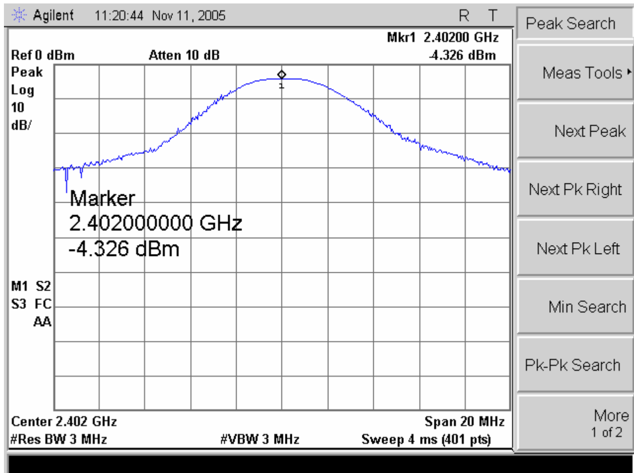
Plot 7. Peak Power Output Test Results – Channel 1
