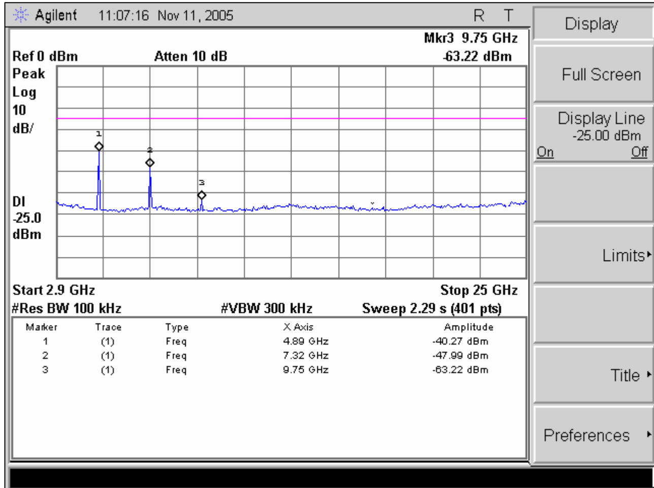
Plot 17. Channel 38 Spurious Conducted Emissions Test Plot (3)
