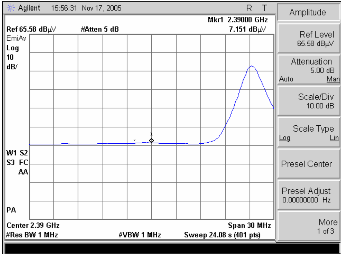
Plot 22. Channel 1 Band Edge Test Results, Average (Channel 1)
