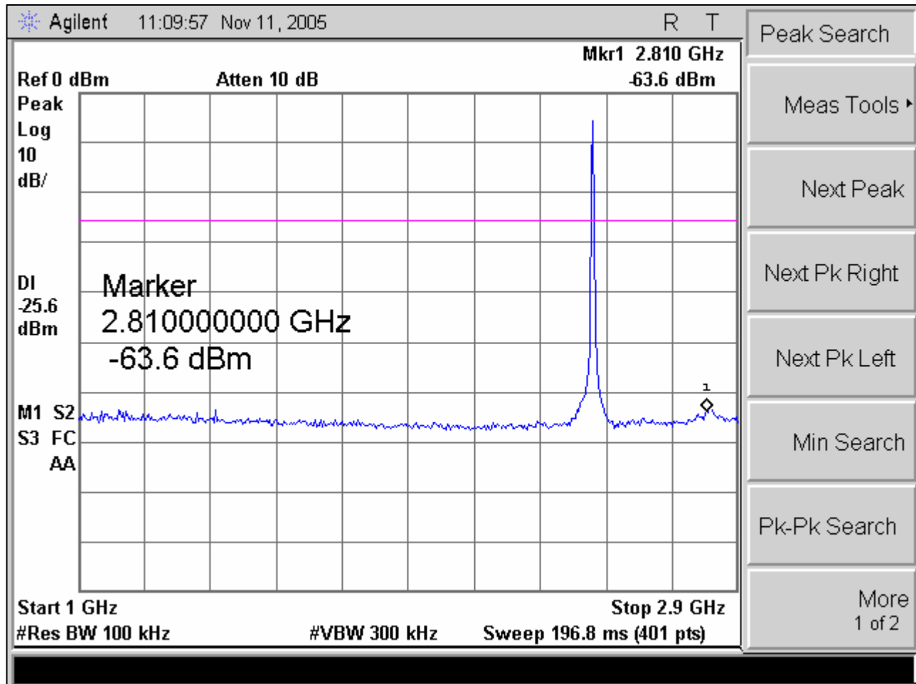
Plot 15. Channel 78 Spurious Conducted Emissions Test Plot (2)
