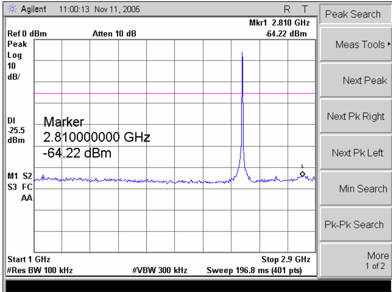
Plot 13. Channel 1 Spurious Conducted Emission Test Plot (2)
