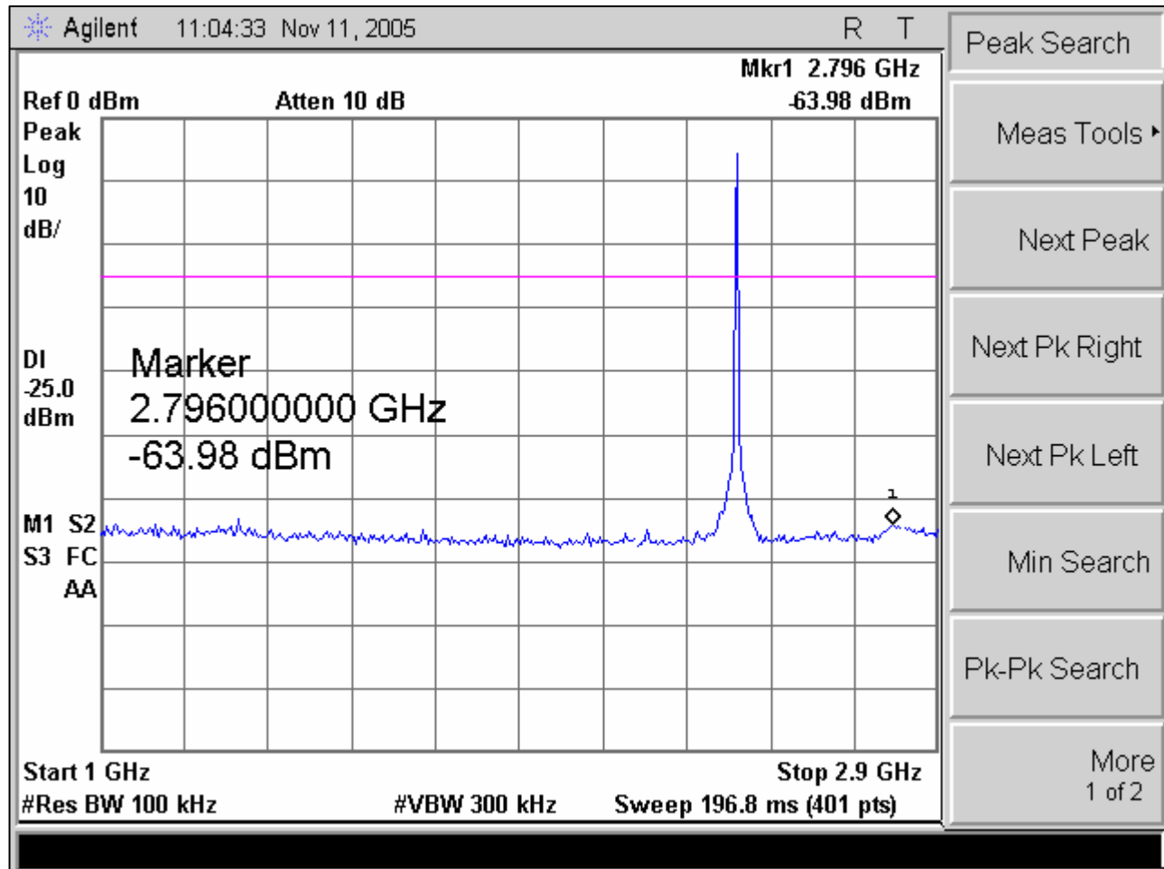
Plot 14. Channel 38 Spurious Conducted Emission Test Plot (2)
