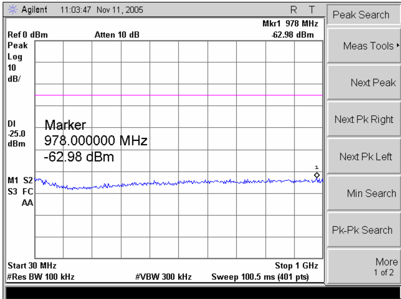
Plot 11. Channel 38 Spurious Conducted Emission Test Plot (1)
