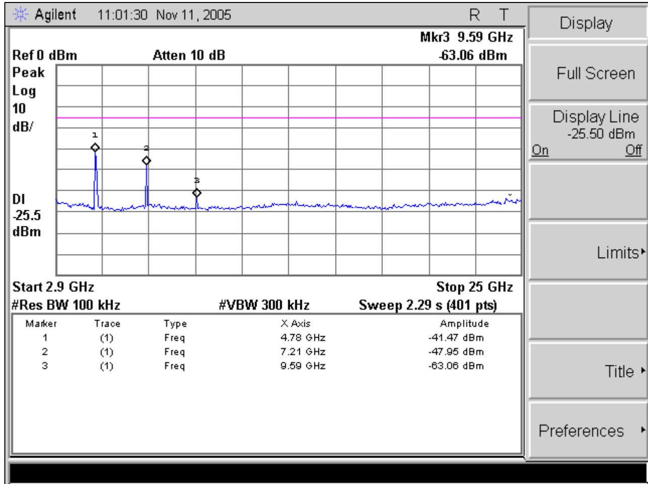
Plot 16. Channel 1 Spurious Conducted Emissions Test Plot (3)
