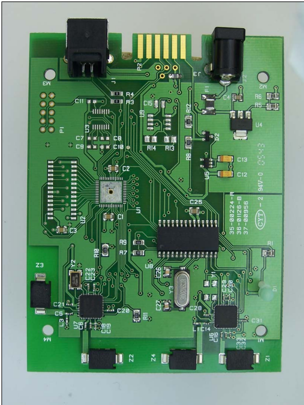
Photograph 1. Antenna Requirement Test Setup
