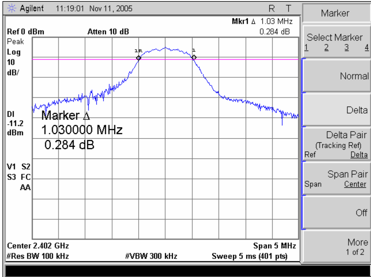
Plot 4. Occupied Bandwidth; Test Results, Channel 1
