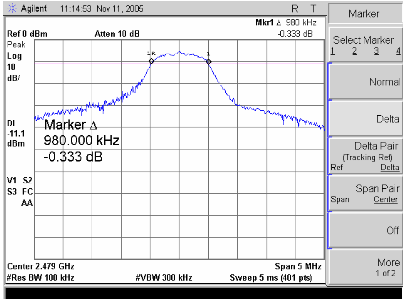
Plot 6. Occupied Bandwidth; Test Results, Channel 78
