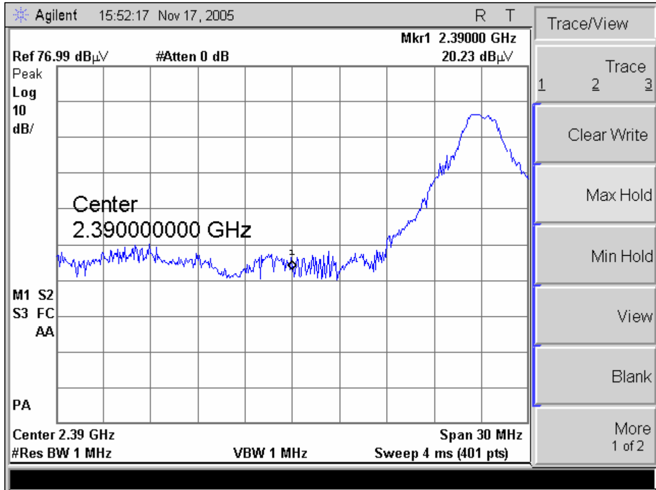
Plot 23. Channel 1 Band Edge Test Results, Peak (Channel 1)
