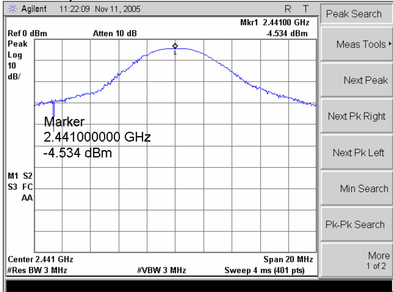
Plot 8. Peak Power Output Test Results – Channel 38
