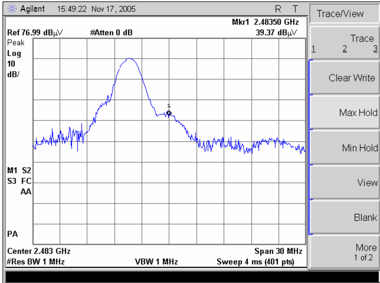
Plot 25. Channel 78 Band Edge Test Results, Peak (Channel 78)
