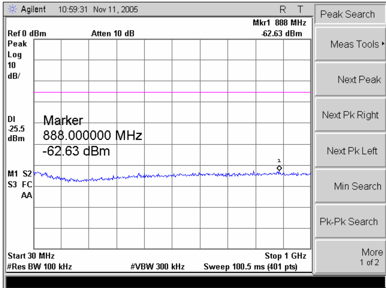
Plot 10. Channel 1 Spurious Conducted Emission Test Plot (1)
