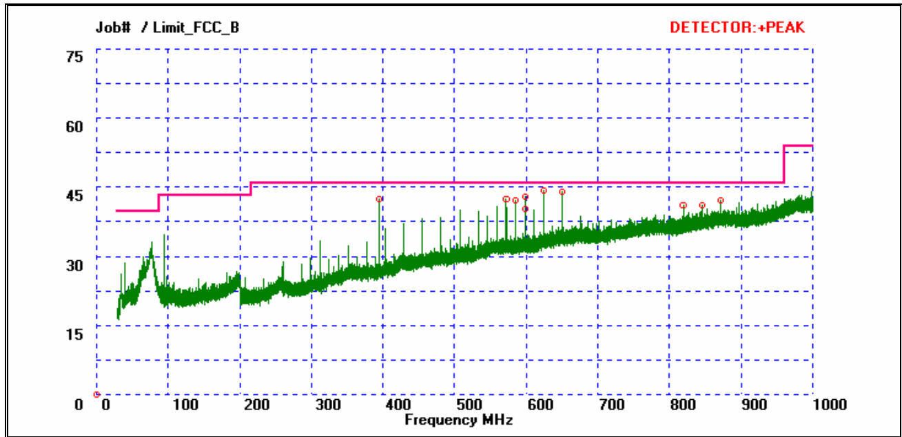
Plot 3. Unintentional Radiators Prescan
