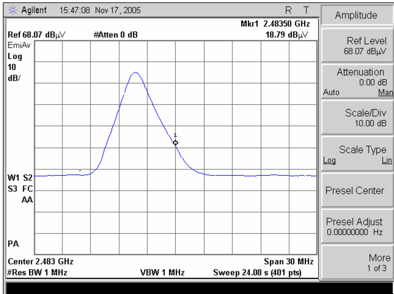
Plot 24. Channel 78 Band Edge Test Results, Average (Channel 78)
