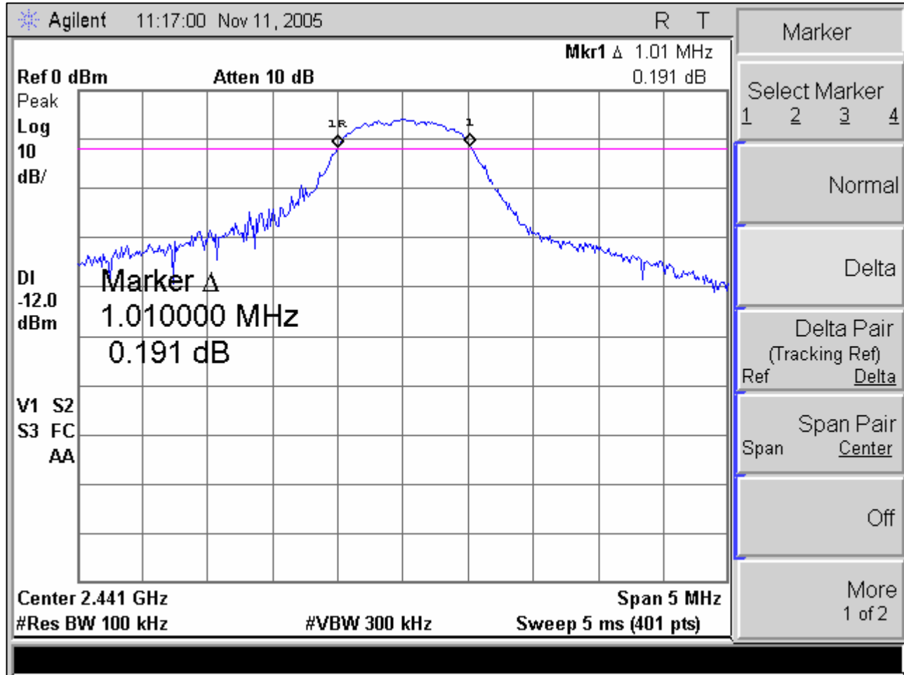
Plot 5. Occupied Bandwidth; Test Results, Channel 38
