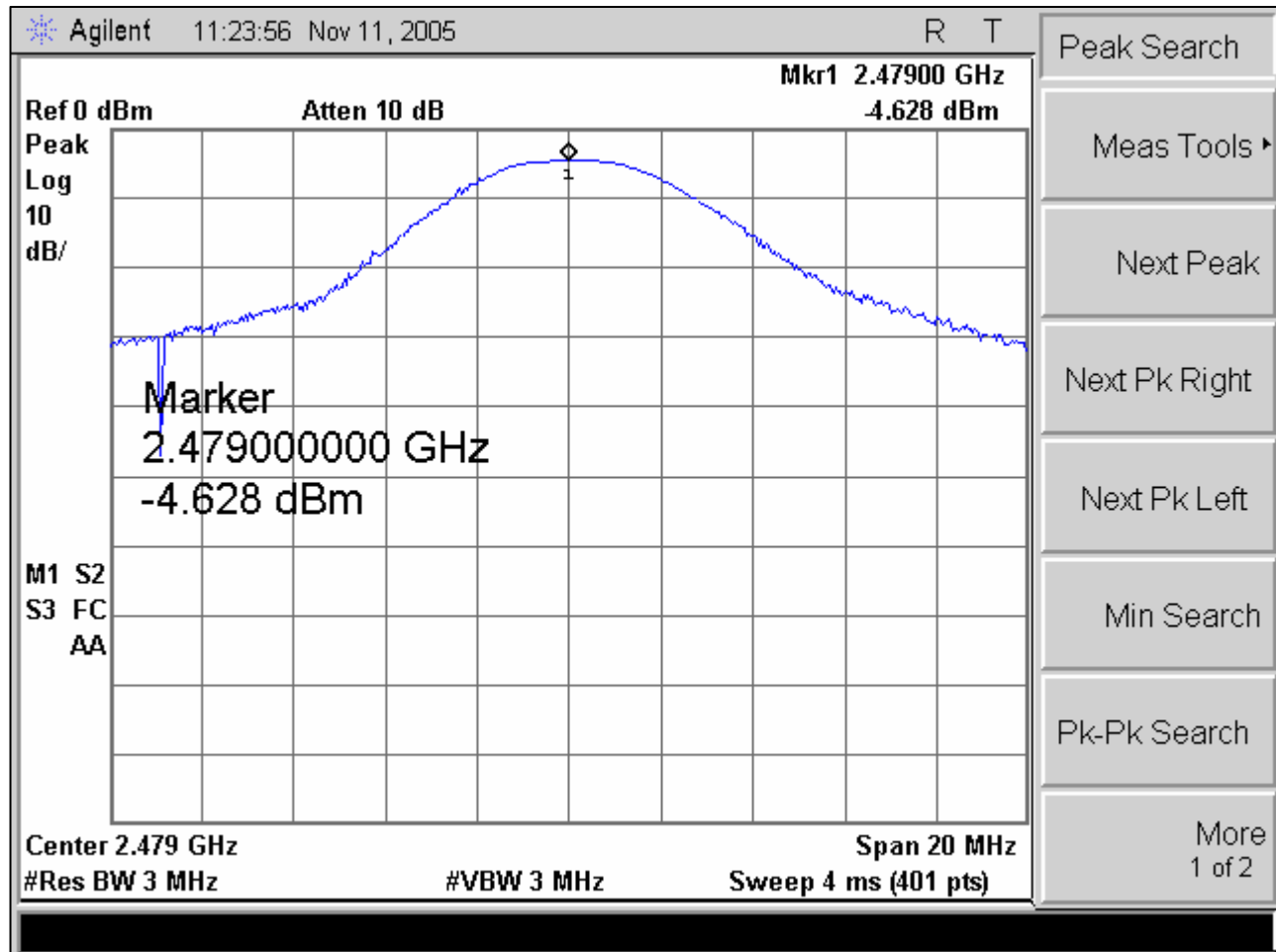
Plot 9. Peak Power Output Test Results – Channel 78
