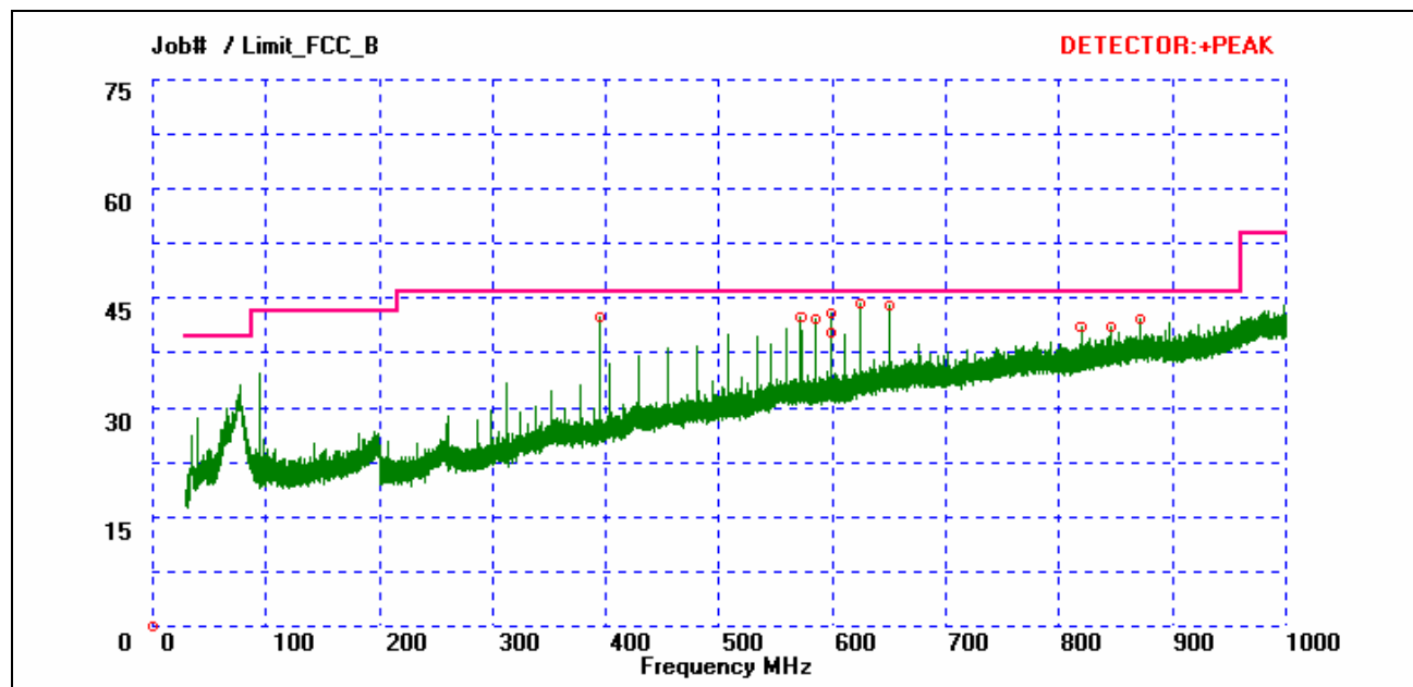
Plot 3. Radiated Emissions Limits Test Results
