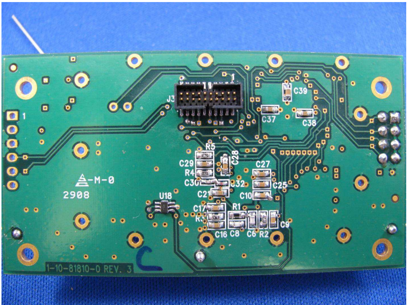
Transceiver – Bottom Side with antenna
