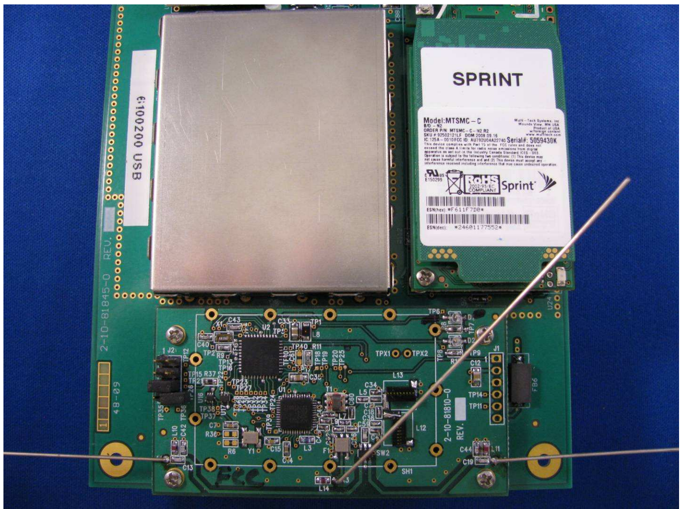
Transceiver mounted on Main Board
