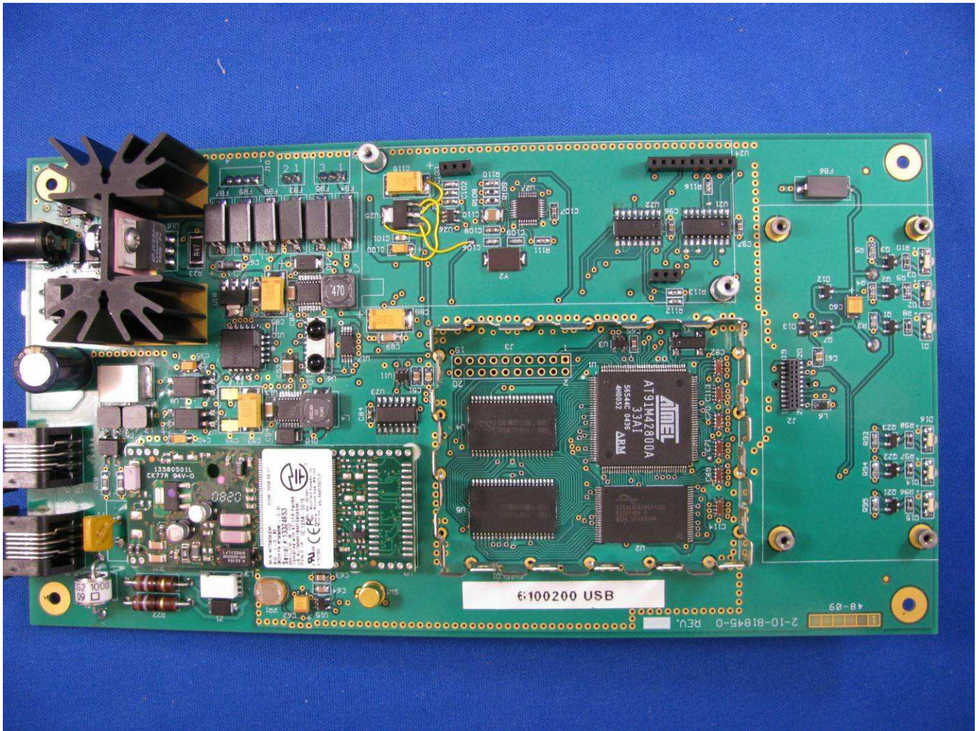
Main Board-Top Side (Depopulated)
