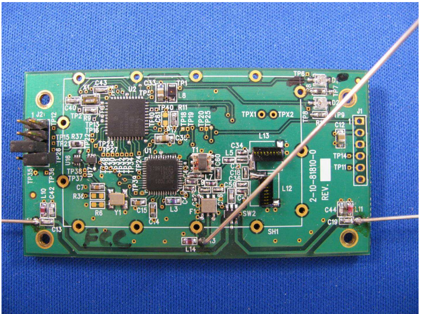
Transceiver – Top Side with antenna
