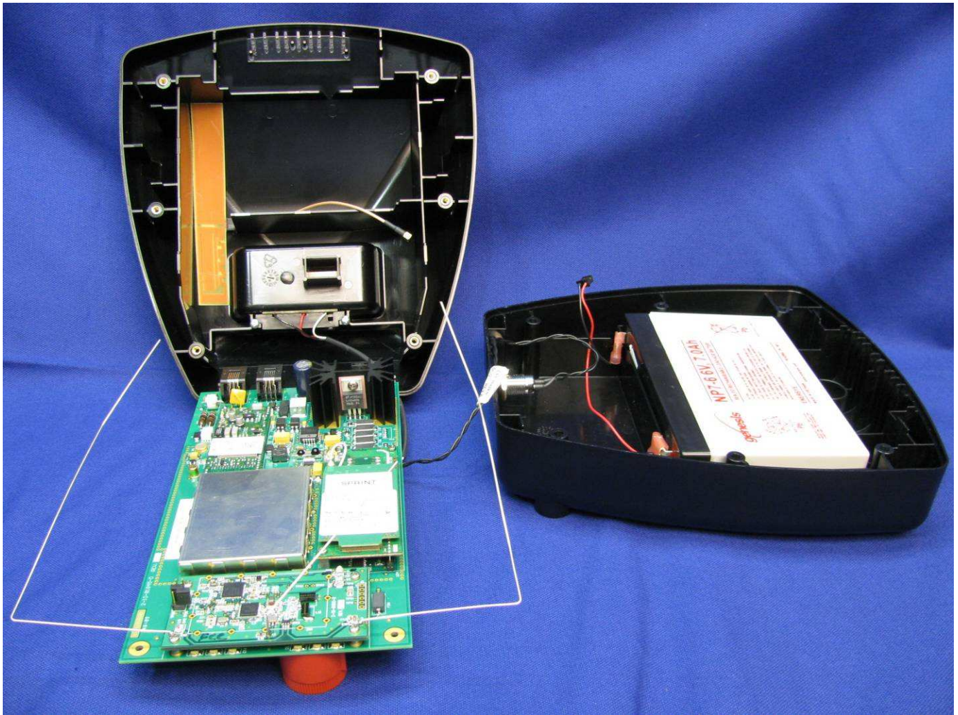
Case Exploded View
