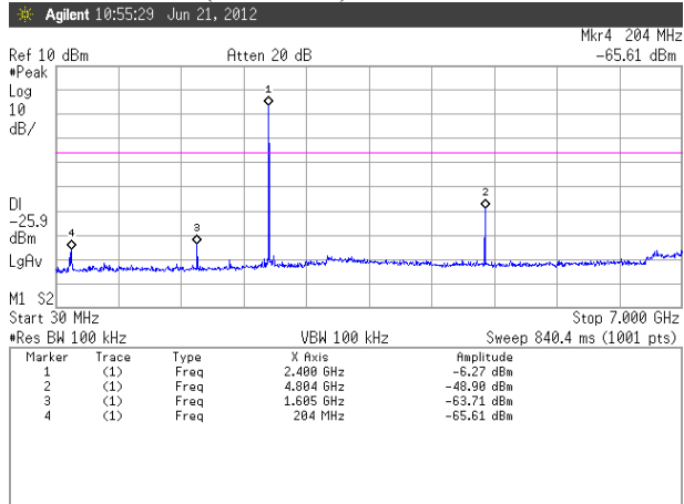
Figure 8. Spurious RF conducted emissions
