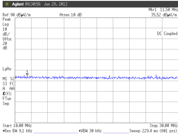
Figure 9. Emission plot for the preliminary radiated measurements
