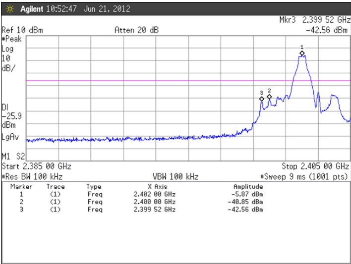
Figure 6. Plot of the Band Edge (Conducted) Lower band-edge
