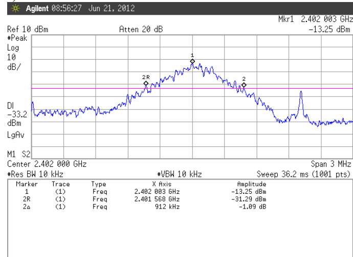
Figure 3. Plot of the 20 dB Channel Bandwidth Basic (GFSK) Lowest Channel (2402 MHz)
