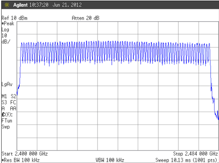
Figure 4. Plot of the Number of Hopping Channels
