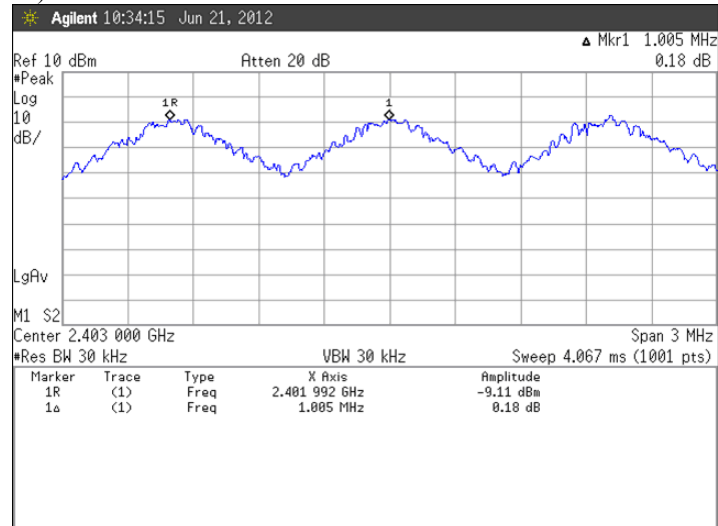
Figure 2. Plot of the Carrier Frequency Separation Basic (GFSK) Lowest Channel (2402 MHz)
