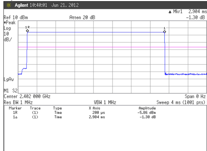
Figure 5. Plot of the Time of Occupancy
