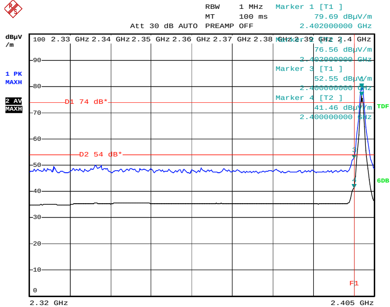
Figure 7. Plot of the Band Edge (Radiated)
