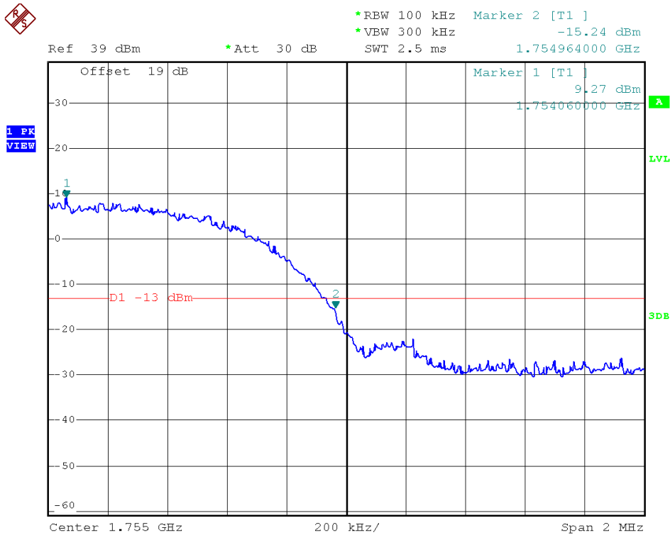
(Plot R: HSDPA1700 Channel = 1513)
