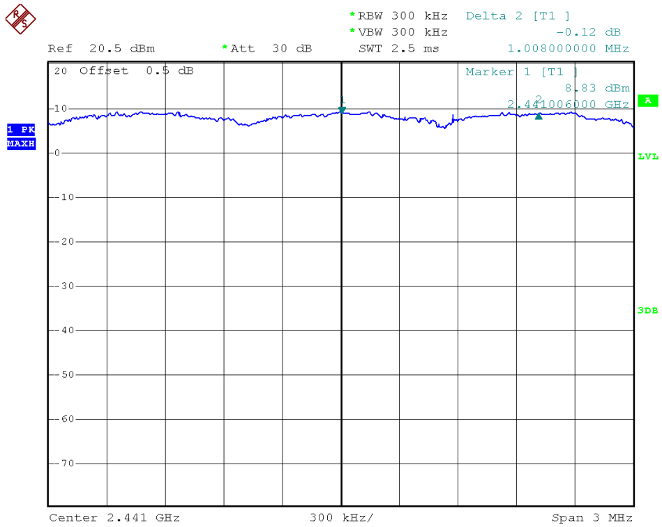
8-DPSK Mode
