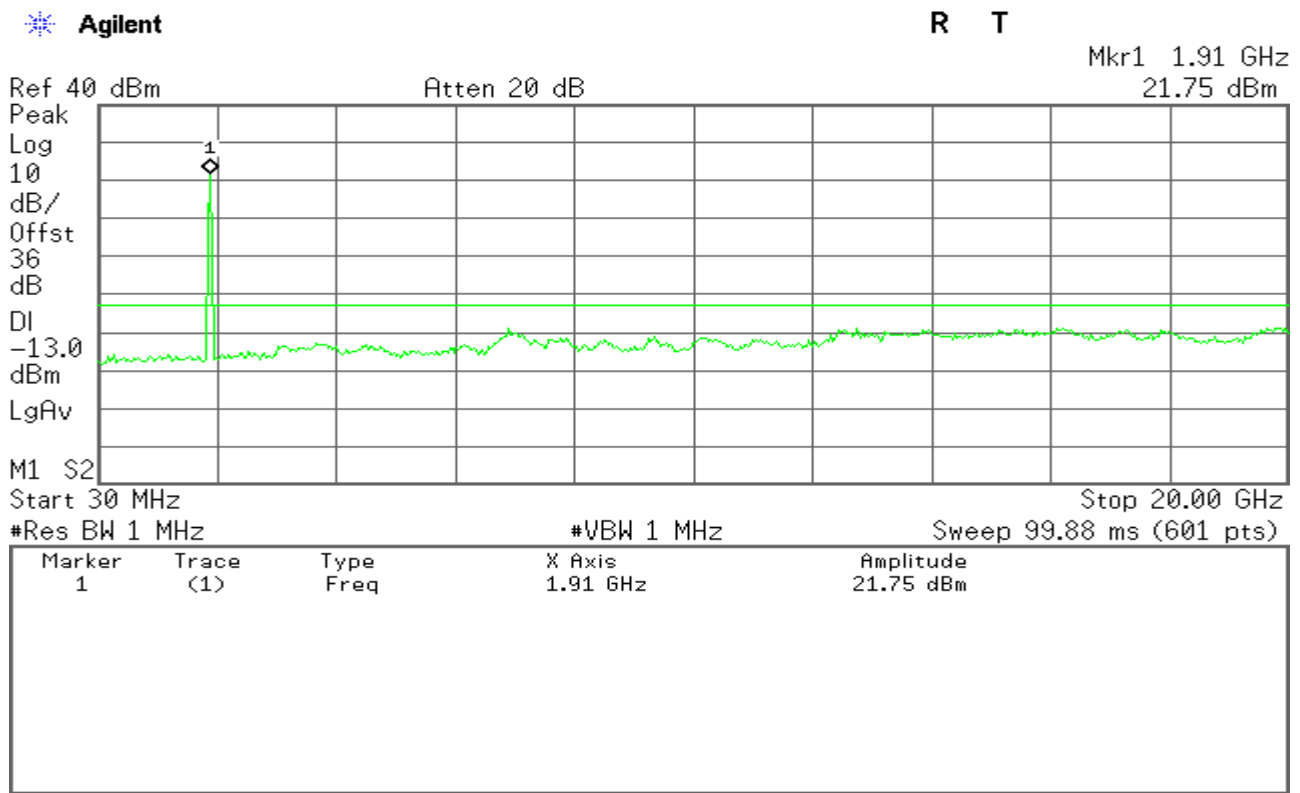
Figure 12-8: Out of Band emission at antenna terminals – WCDMA CH High
