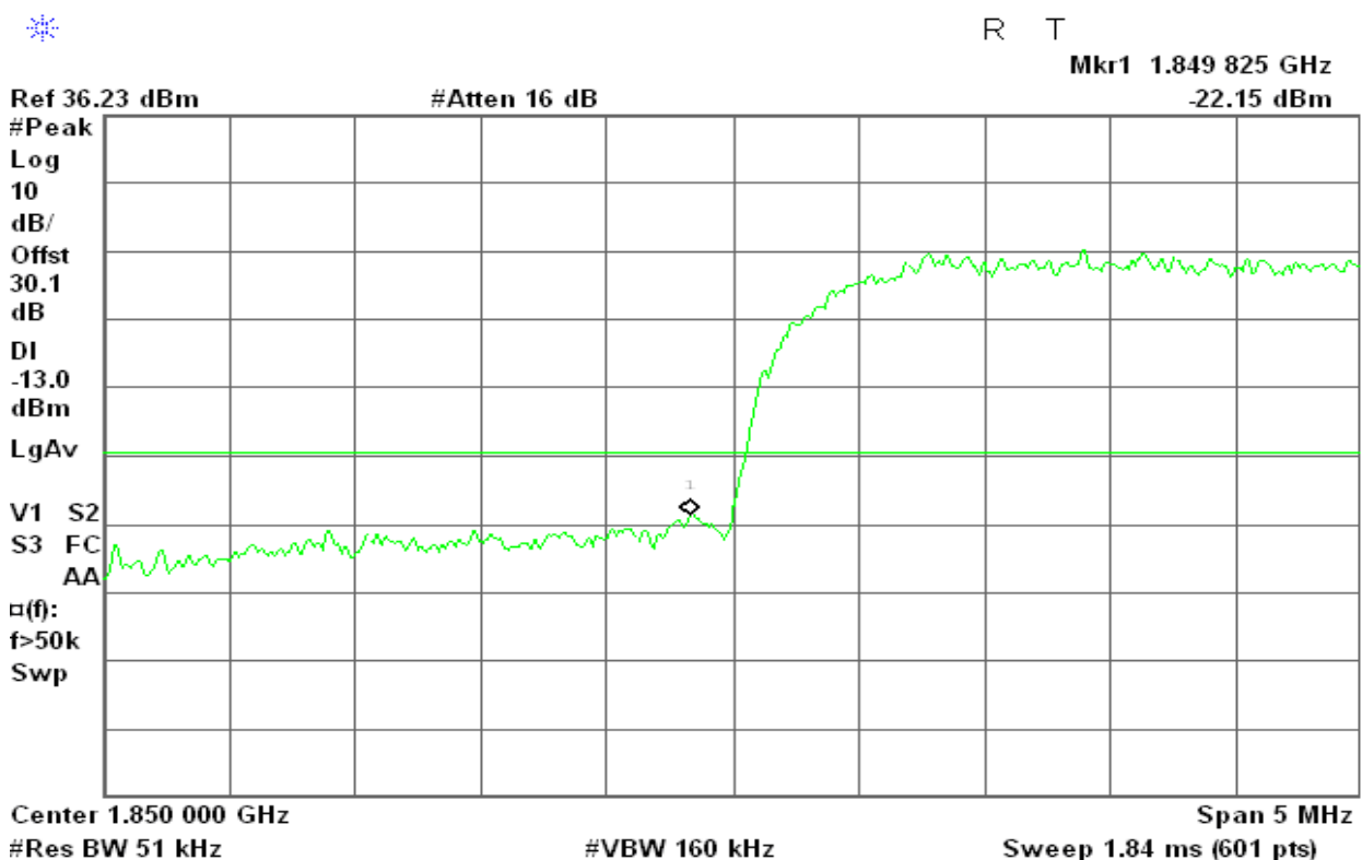
Figure 12-9: Band Edge emissions –WCDMA CH Low
