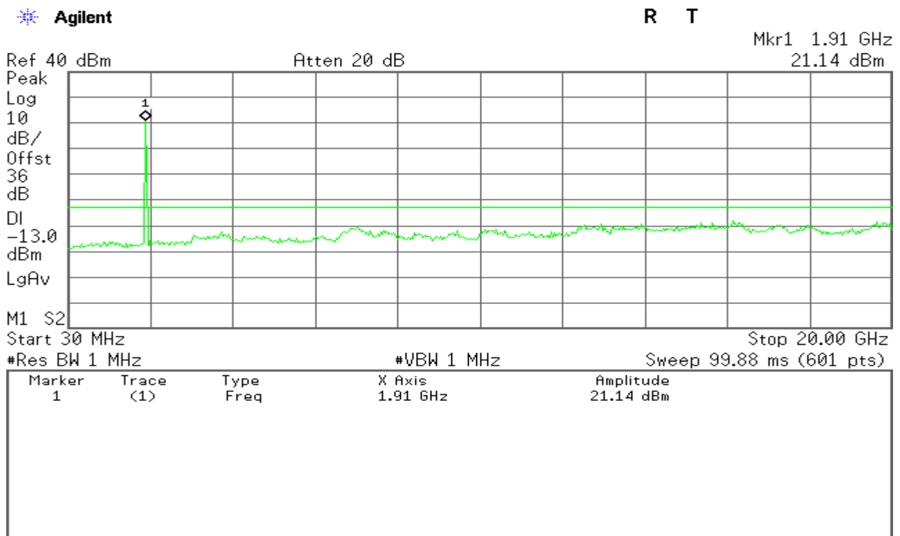
Figure 12-13: Out of Band emission at antenna terminals – HSUPA CH High
