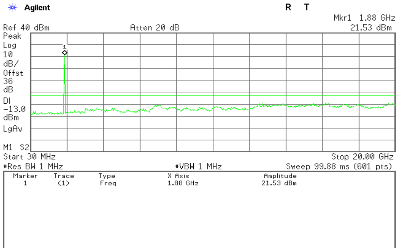
Figure 12-7: Out of Band emission at antenna terminals – WCDMA CH Mid
