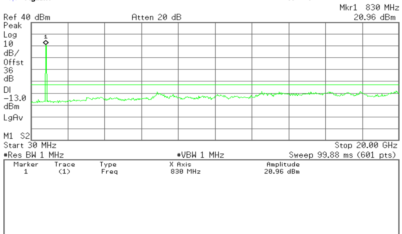
Figure 12-1: Out of Band emission at antenna terminals – HSUPA CH Low
