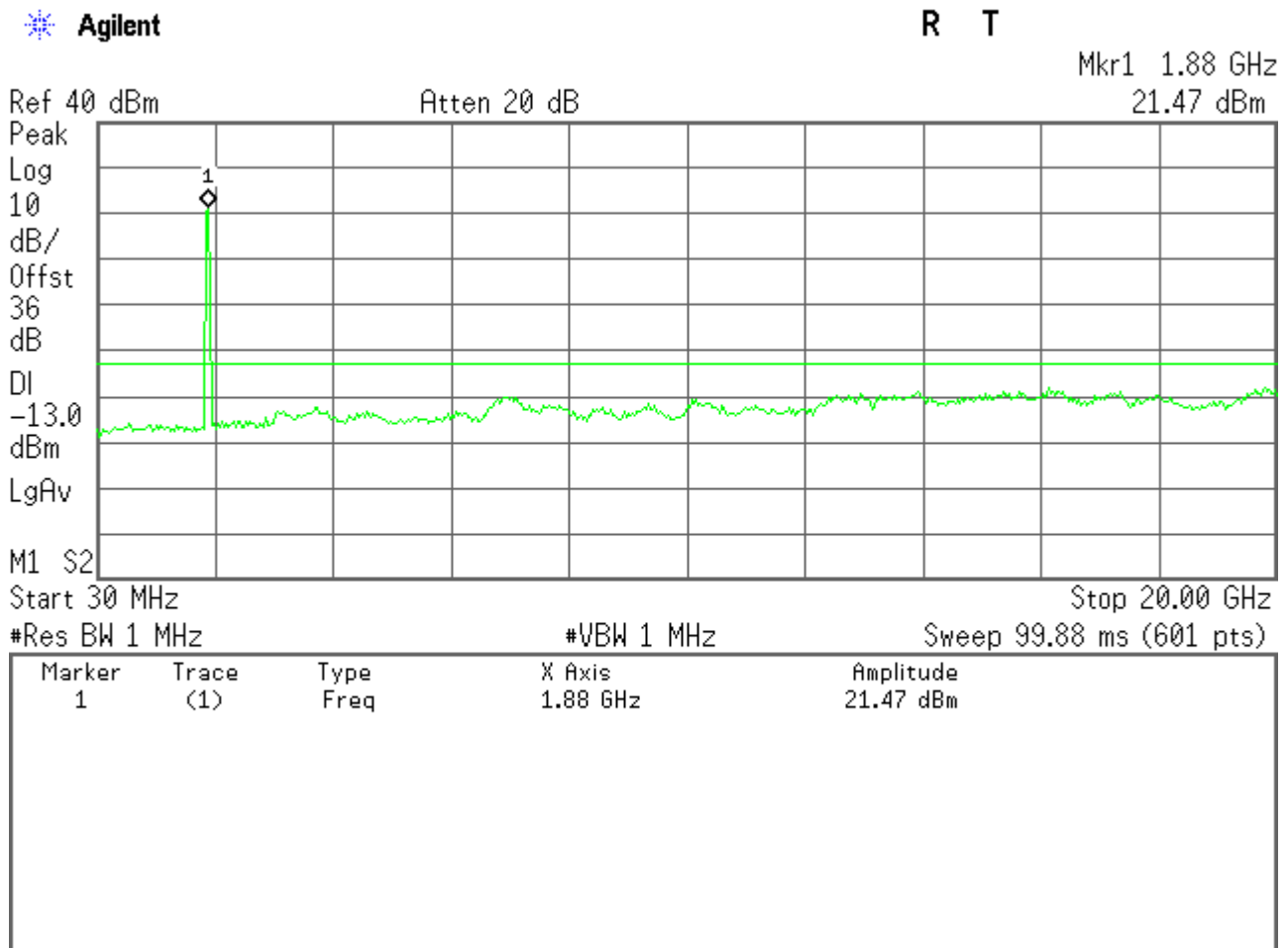
Figure 12-11: Out of Band emission at antenna terminals – HSUPA CH Low
