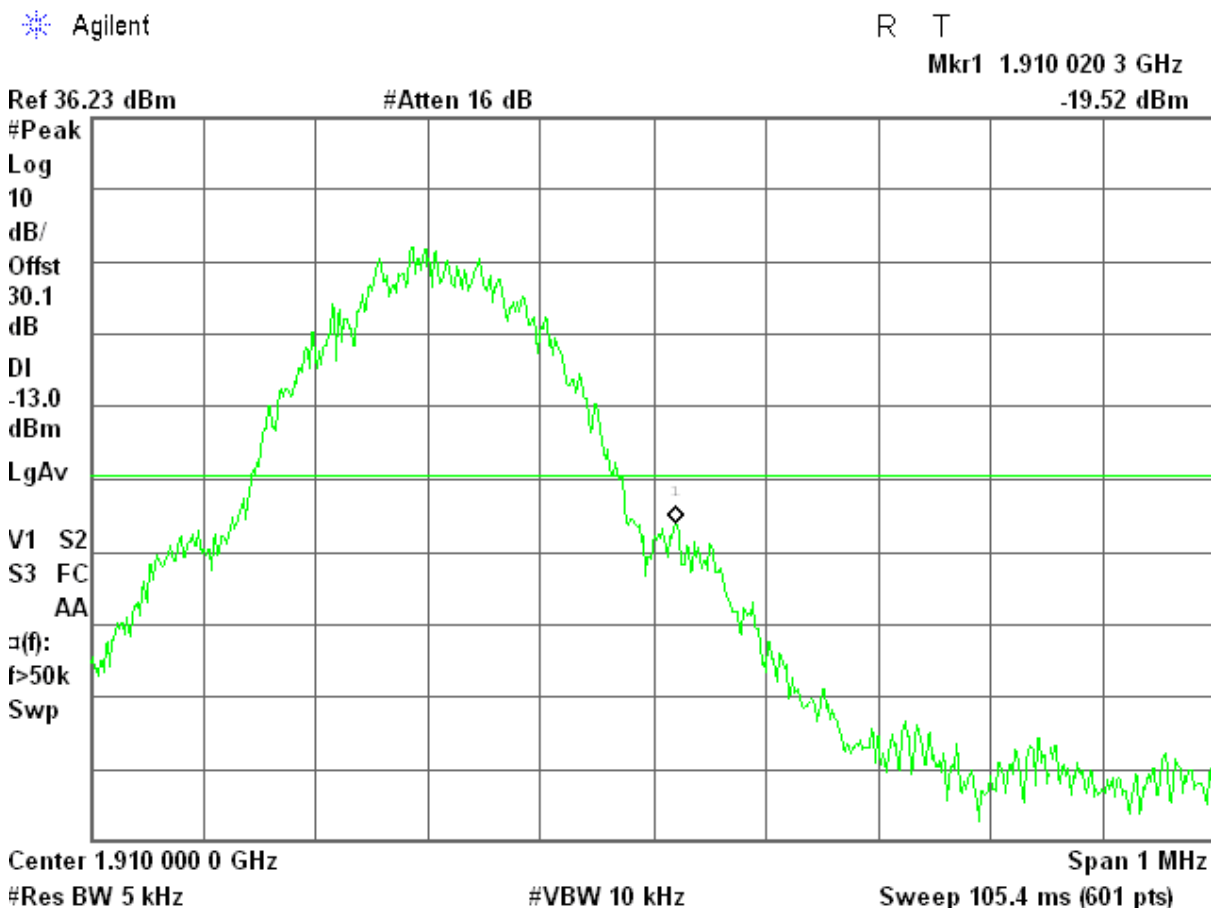
Figure 14-4: Band Edge emissions – EDGE CH High
