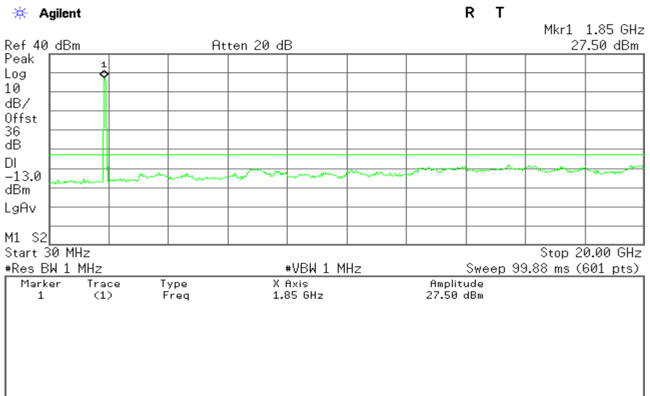
Figure 13-4: Out of Band emission at antenna terminals –EDGE CH Low
