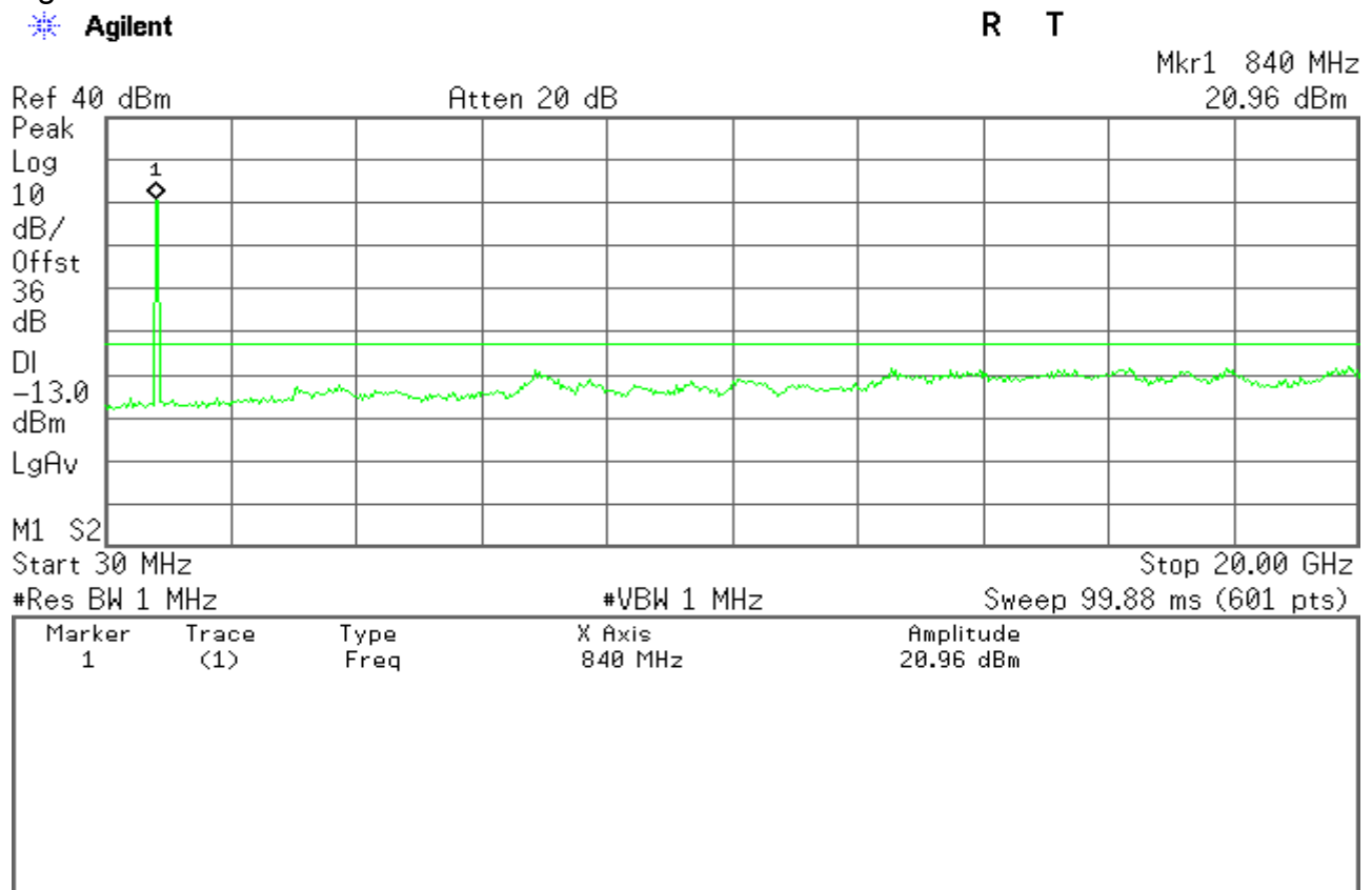
Figure 12-3: Out of Band emission at antenna terminals – HSUPA CH High
