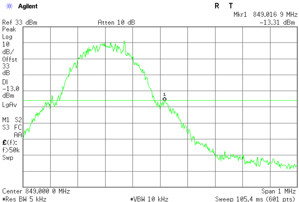
Figure 3-2: Band Edge emissions –GSM CH High
