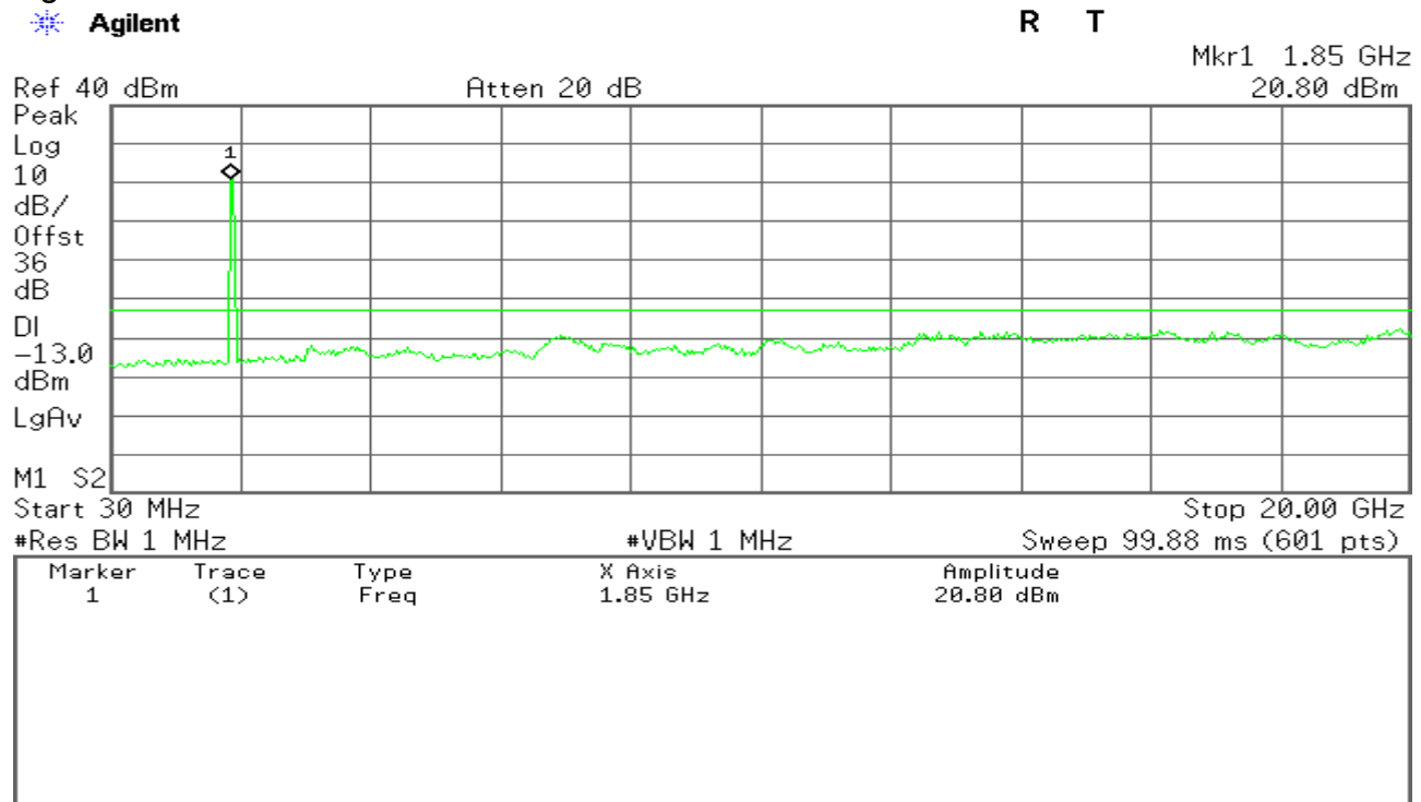
Figure 12-6: Out of Band emission at antenna terminals – WCDMA CH Low
