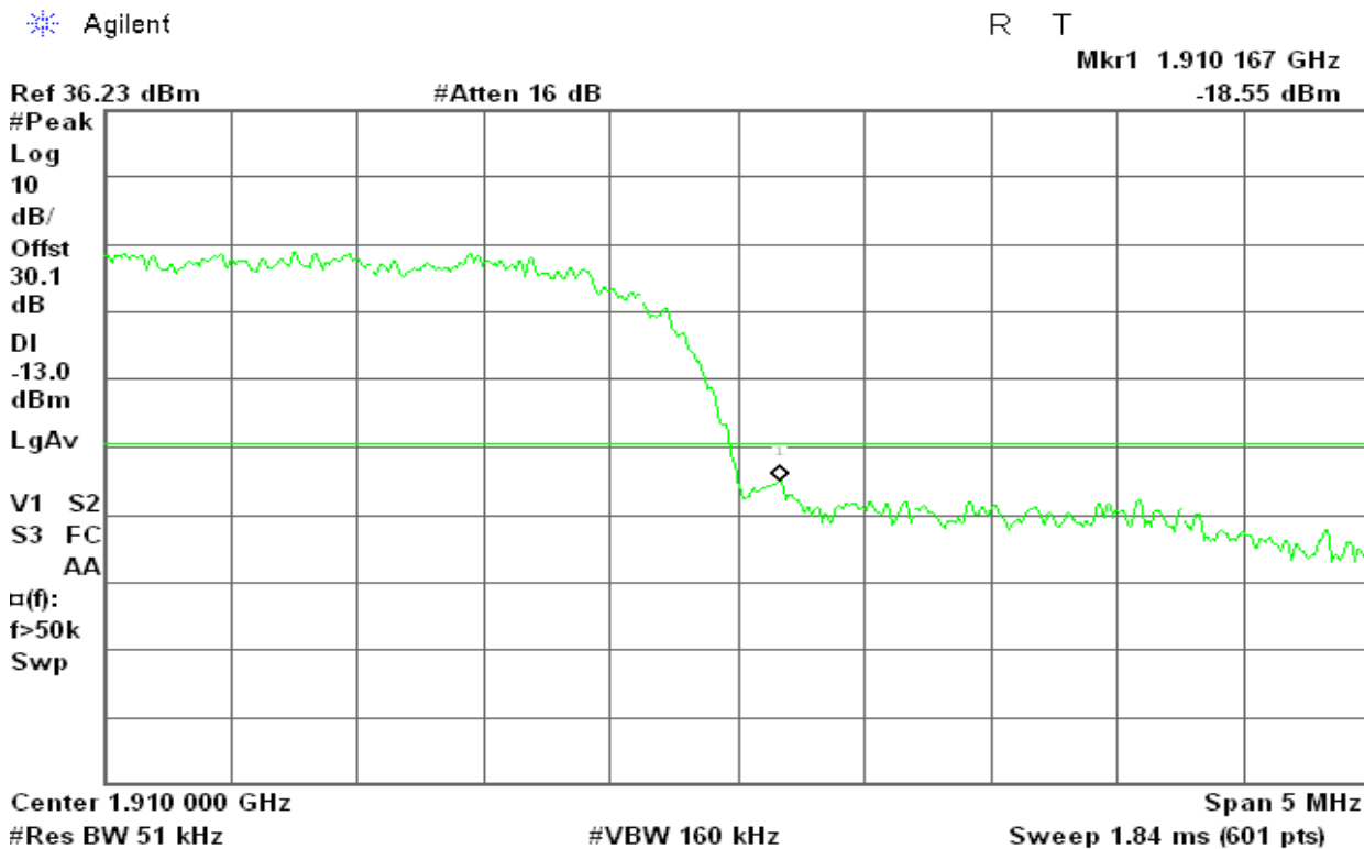
Figure 12-15: Band Edge emissions –WCDMA CH High
