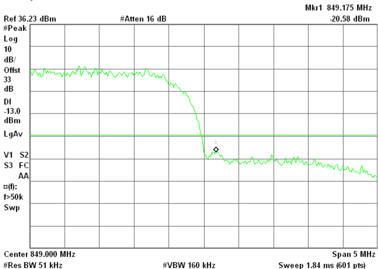
Figure 12-5: Band Edge emissions – HSUPA CH High
