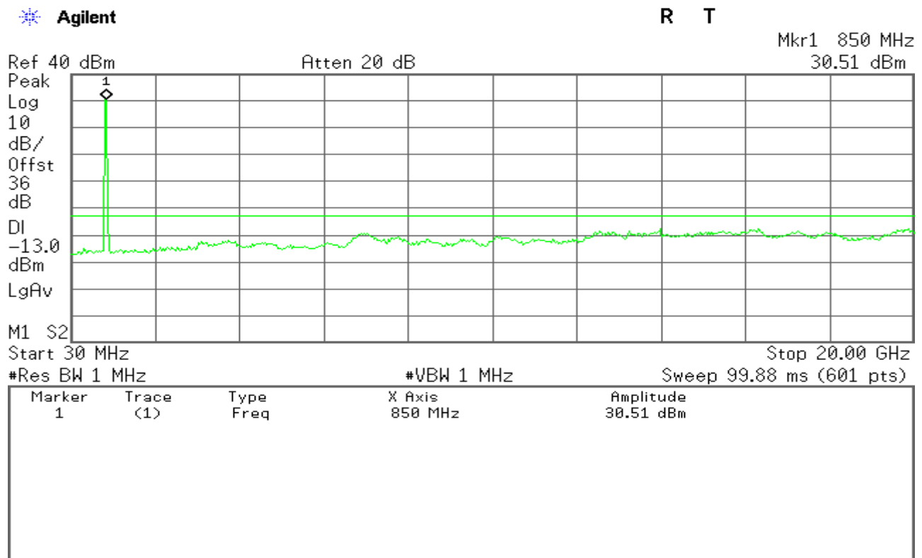
Figure 11-3: Out of Band emission at antenna terminals – WCDMA CH High
