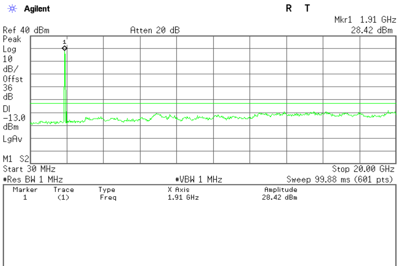
Figure 13-6: Out of Band emission at antenna terminals –EDGE CH High
