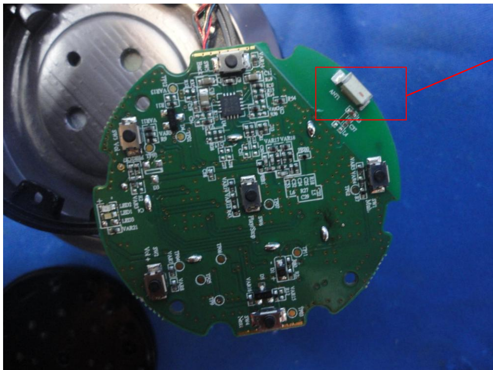
Bluetooth Antenna
