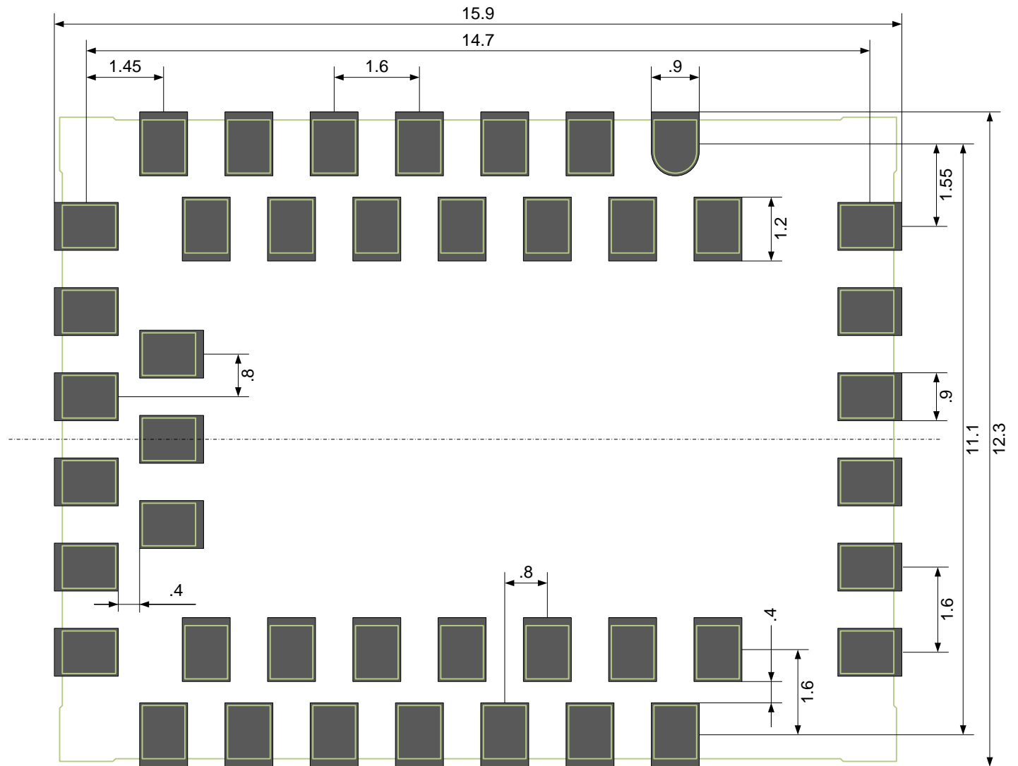
Figure 4. Recommended Land Pattern
