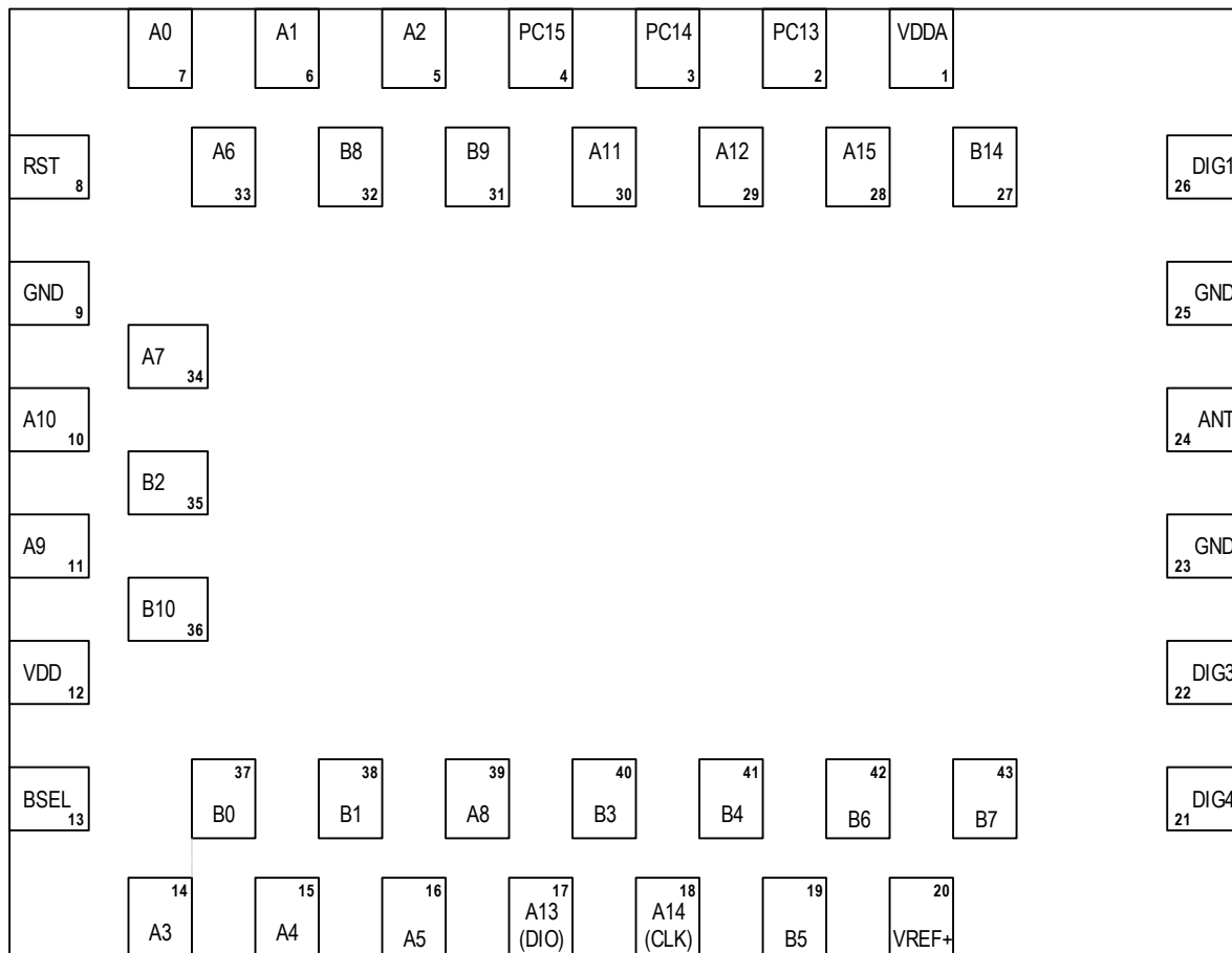
Figure 1. Pin Assignments for 15.6mm × 12.0mm LGA Package – Top View
