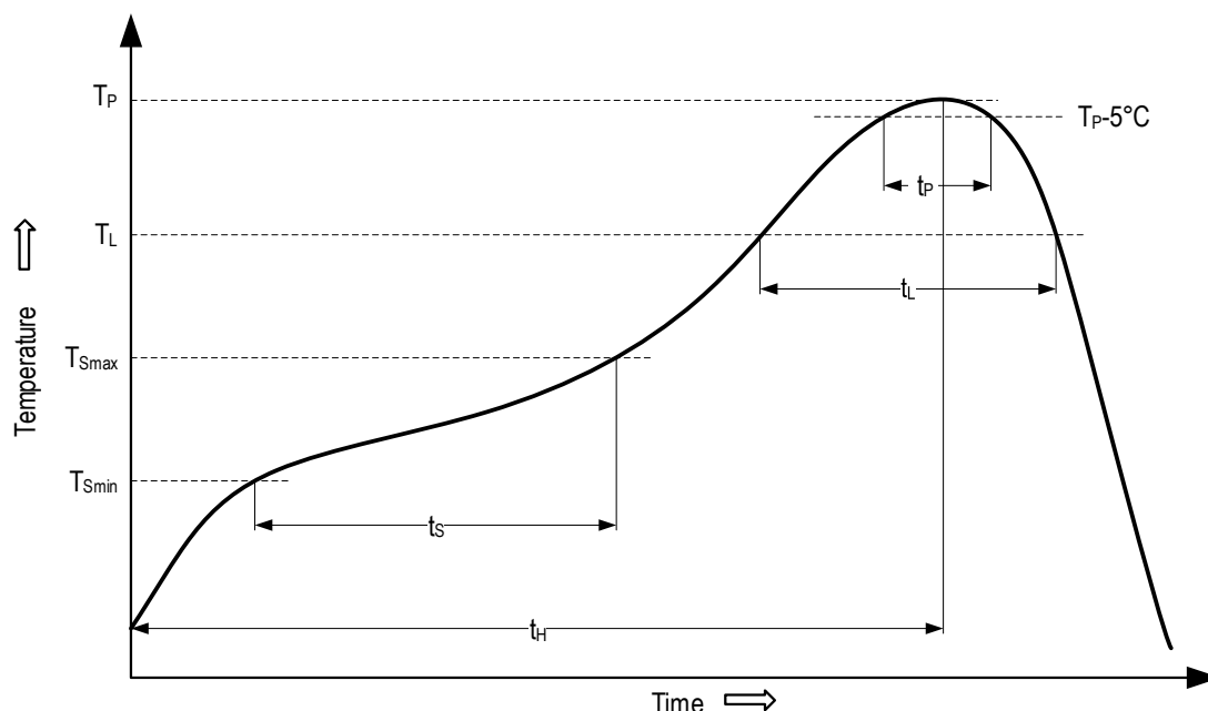
Figure 5. Recommended Temperature Profile for Reflow Soldering (according to J-STD-020D)
