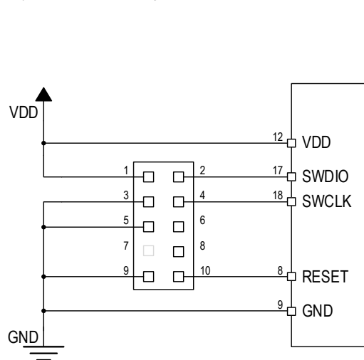
B) 10 Pin Cortex Debug Connector
