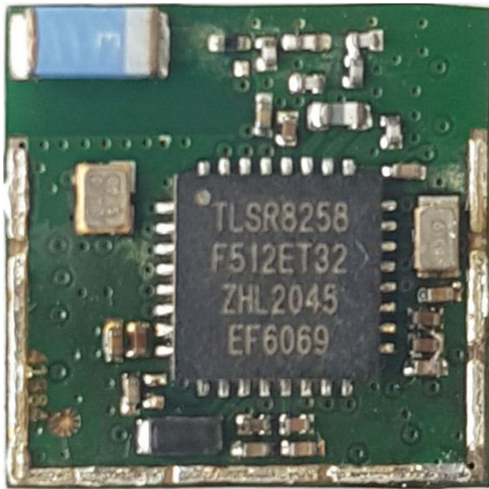
Module Front w/o shielding
